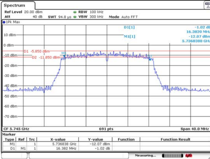
6dB Bandwidth
