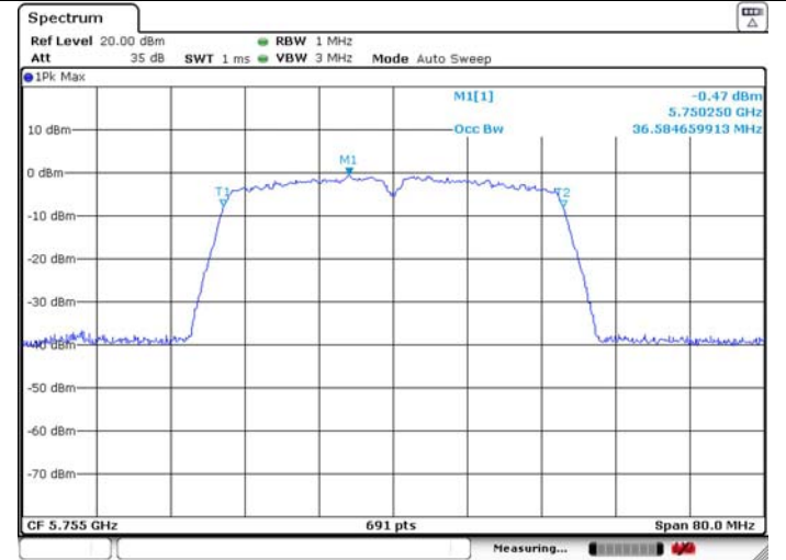
99% Occupied Bandwidth
