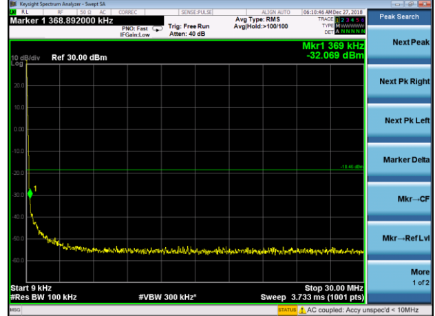
LoRa on channel 0
