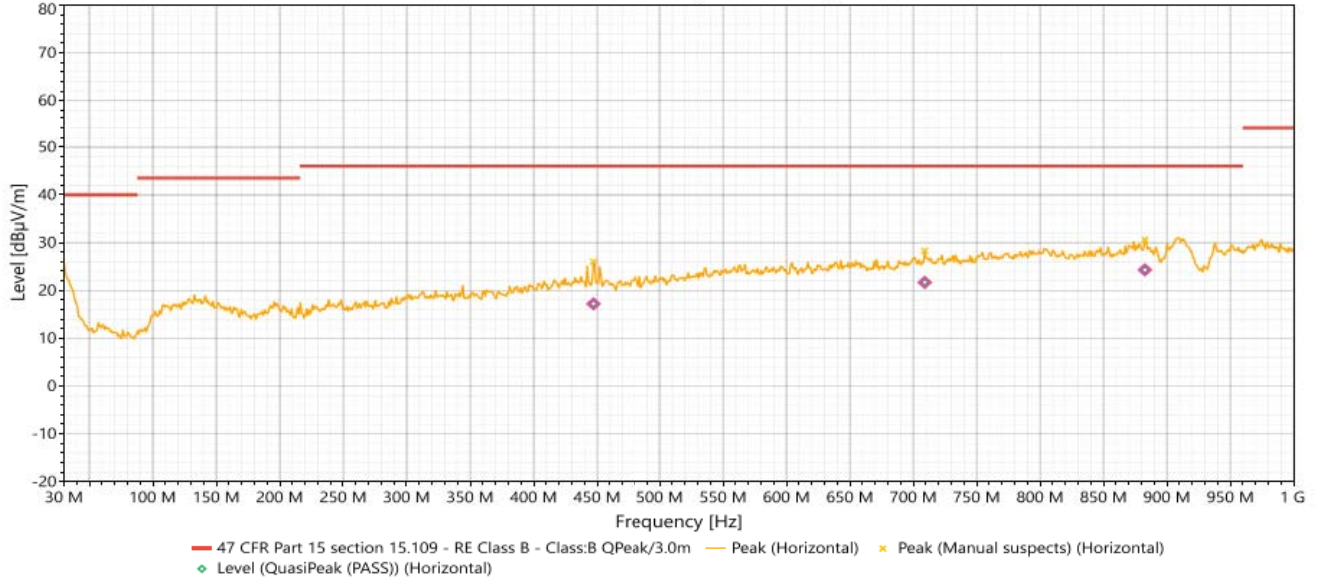
#2 - 30MHz-1GHz (Horizontal)
