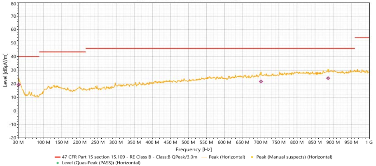
#2 - 30MHz-1GHz (Horizontal)
