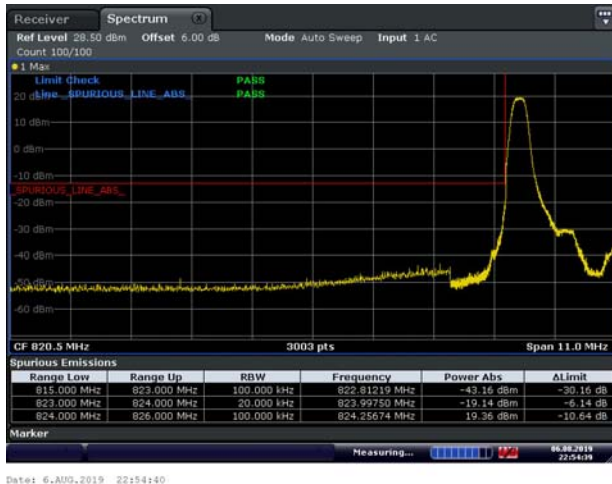
LTE Band 5 QPSK 1.4MHz CH-Low 100%RB
