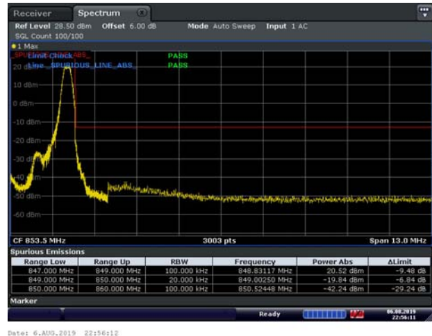
LTE Band 5 QPSK 1.4MHz CH-High 100%RB
