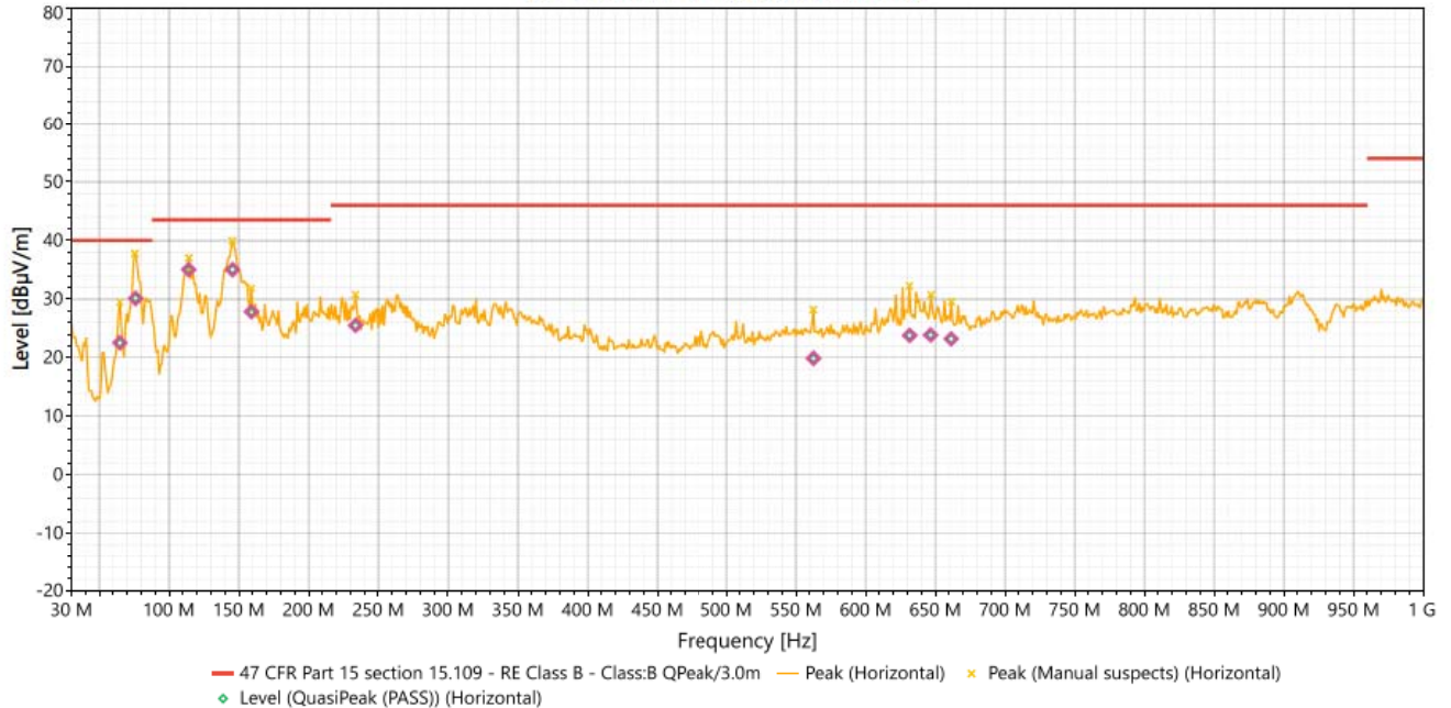
#2 - 30MHz-1GHz (Horizontal)
