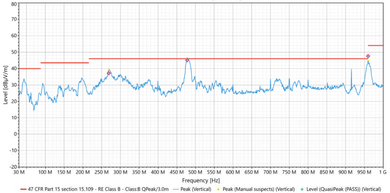
#1 - 30MHz-1GHz (Vertical)
