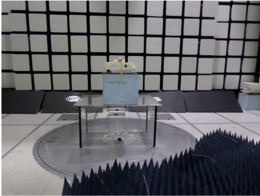
Figure 3: Radiated Emissions, 1-18 GHz - Setup Front View
