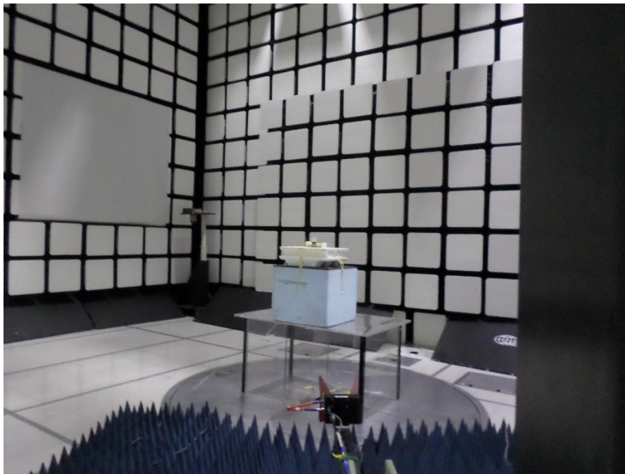
Figure 2: Radiated Emissions, 1-18 GHz - Setup Antenna View
