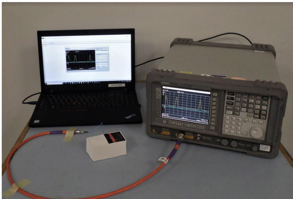
Figure 8: Conducted Spurious Emissions, Test Setup
