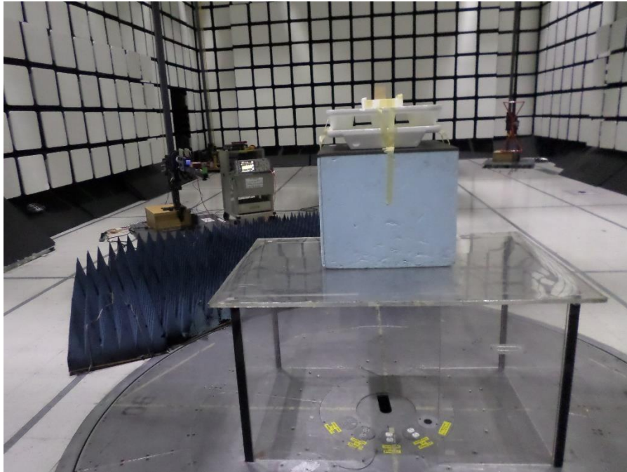
Figure 7: Radiated Emissions, 18-25 GHz - Setup Rear View
