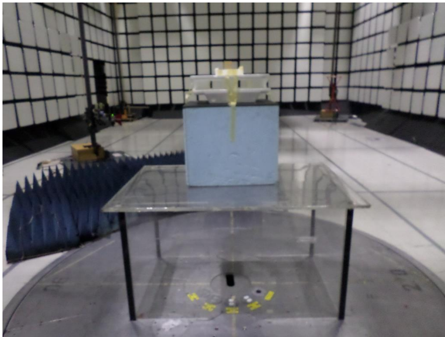
Figure 4: Radiated Emissions, 1-18 GHz - Setup Rear View
