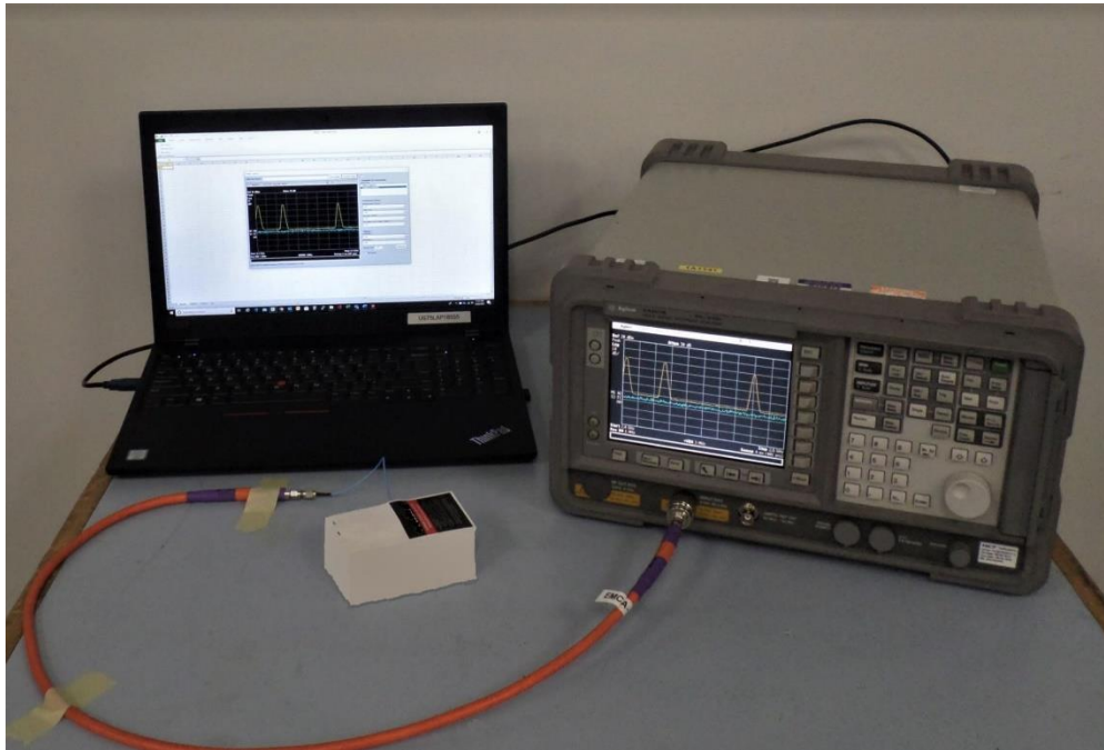
Figure 1: Conducted Measurement, Test Setup
