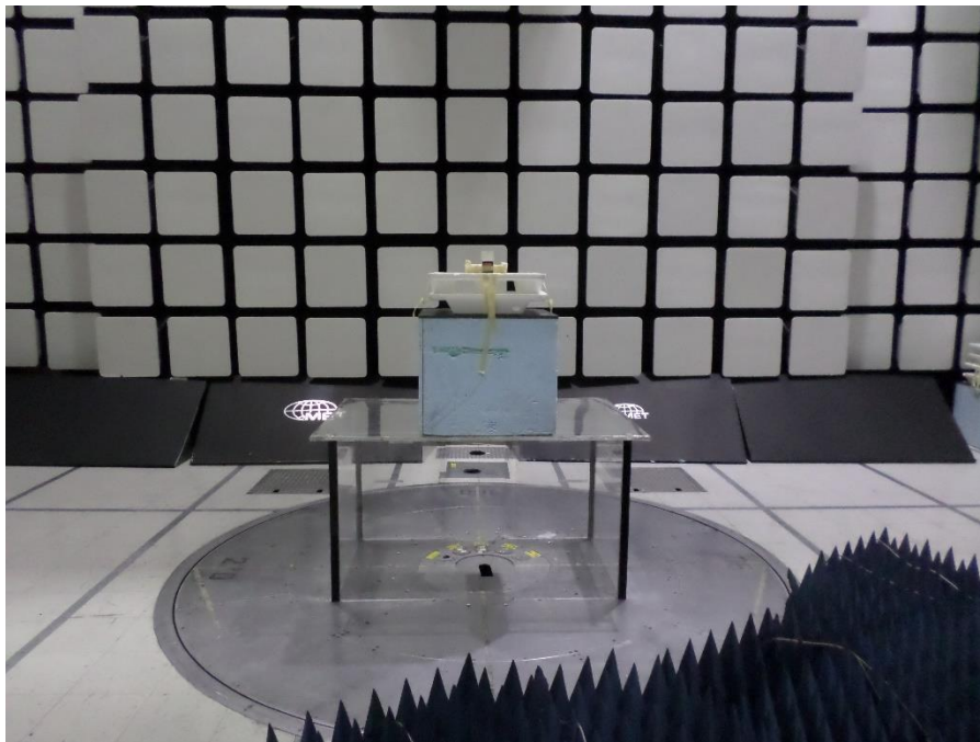
Figure 6: Radiated Emissions, 18-25 GHz - Setup Front View
