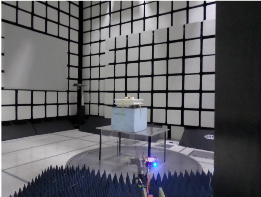
Figure 5: Radiated Emissions, 18-25 GHz - Setup Antenna View
