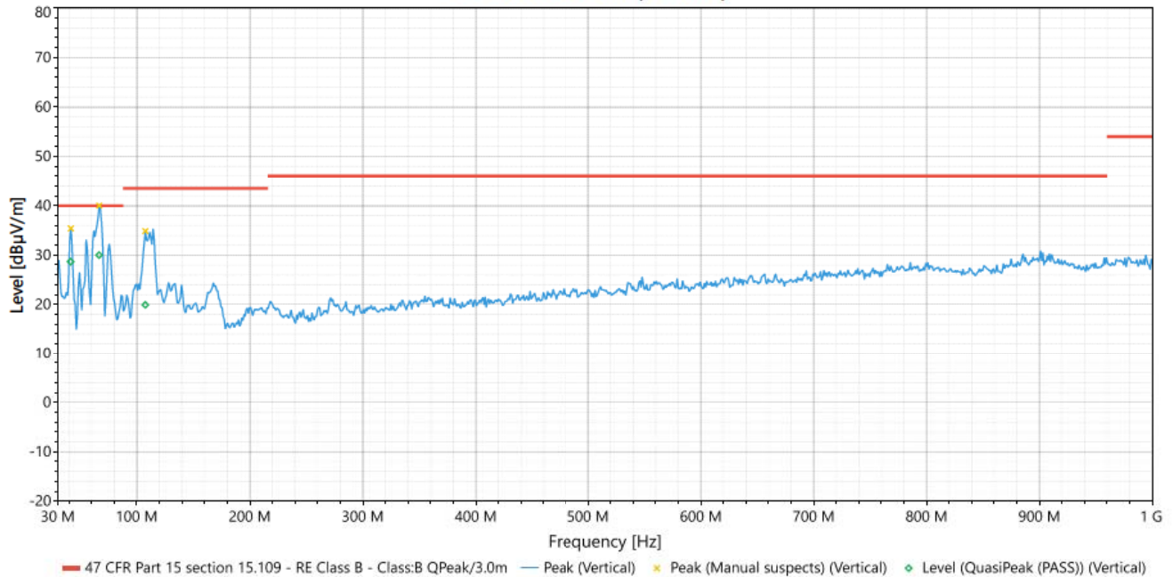
#1 - 30MHz-1GHz (Vertical)
