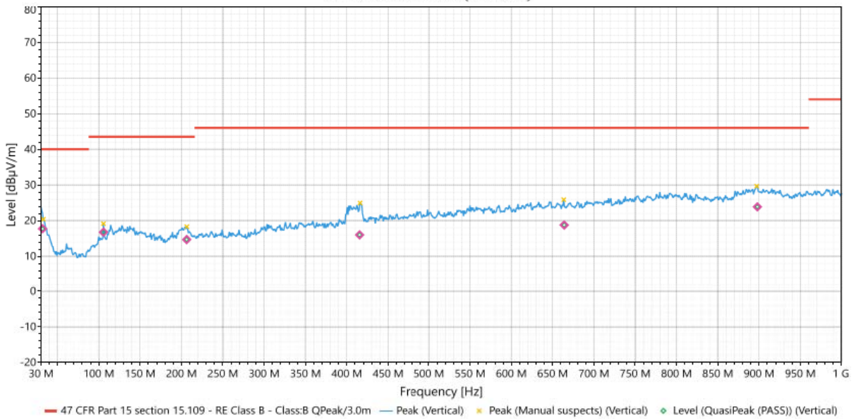
#1 - 30MHz-1GHz (Vertical)
