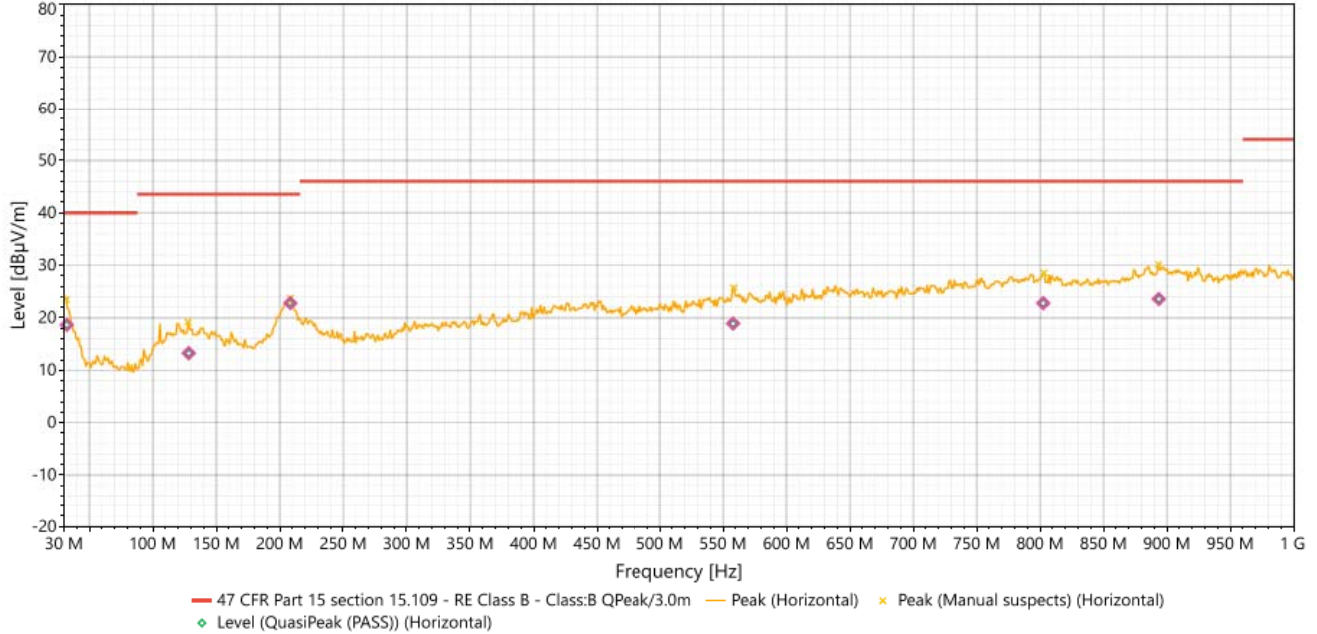
#2 - 30MHz-1GHz (Horizontal)
