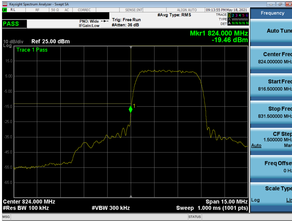
Plot 7-53. Lower Band Edge Plot (WCDMA Cell – Ch. 4132)
