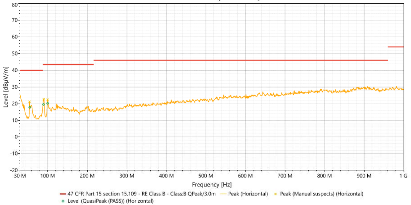
#2 - 30MHz-1GHz (Horizontal)
