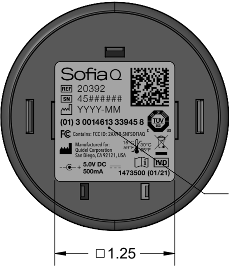
SOFIA Q INSTRUMENT BOTTOM VIEW
