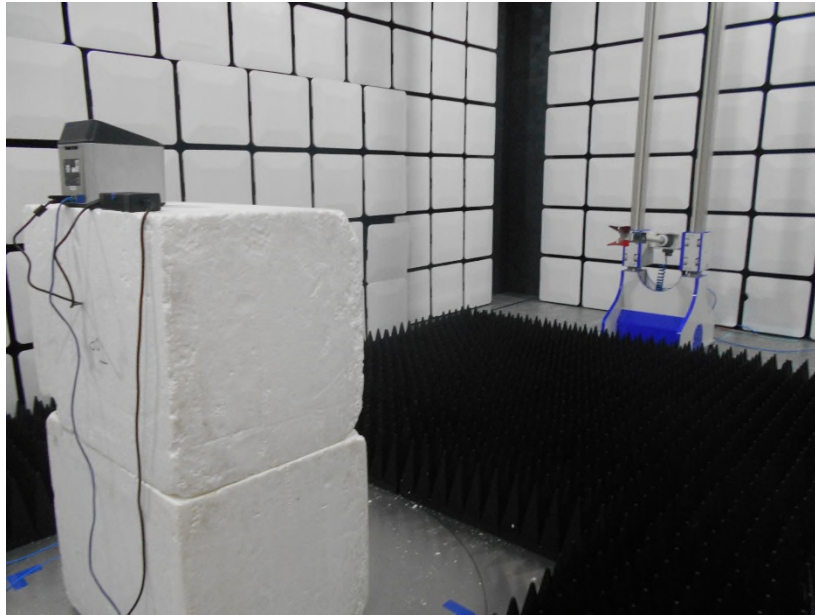
Photo 1.4-1 – Restricted Band-Edge
