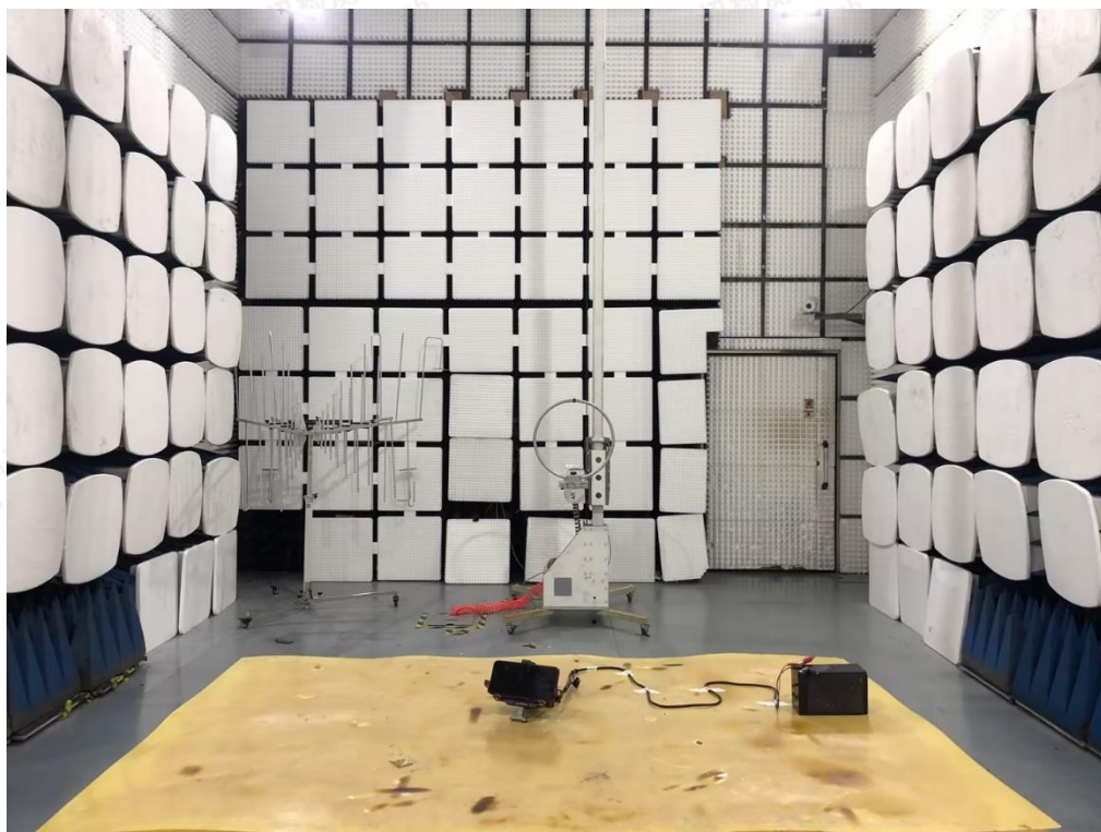
Radiated Emission below 30MHz-DC charge mode
