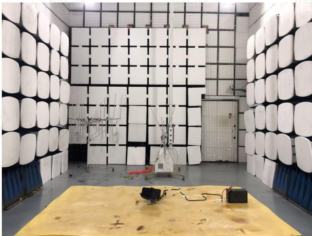
Radiated Emission below 1GHz-DC charge mode
