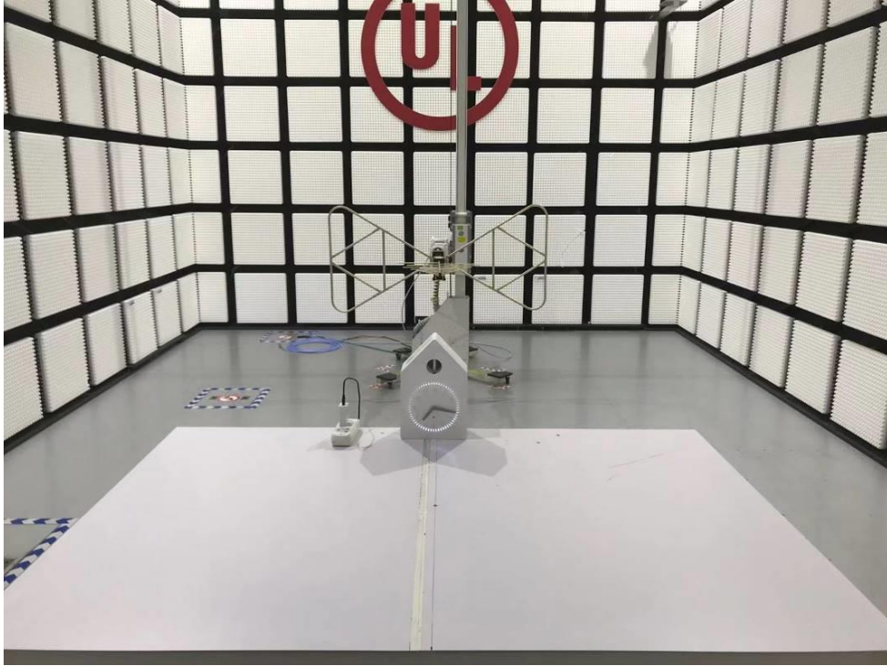
Radiated Disturbance up to 1GHz
