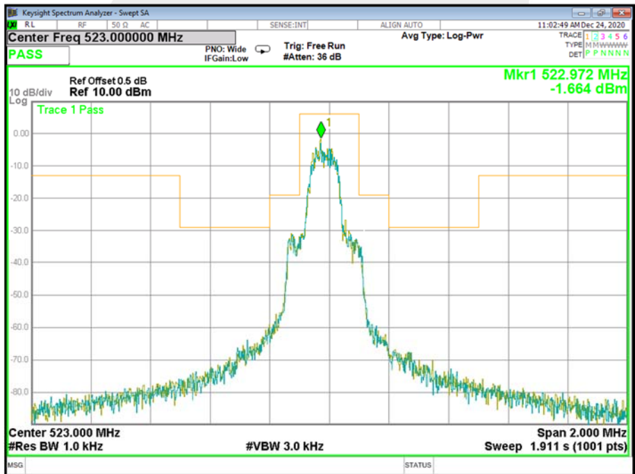
Emission Mask Mid Channel
