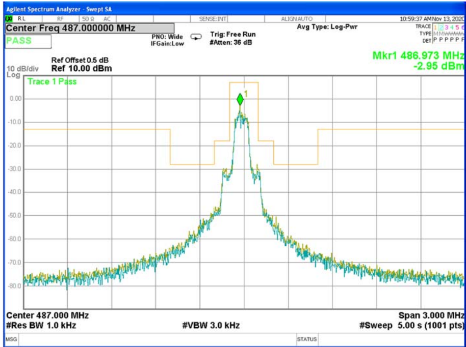
Emission Mask Low Channel
