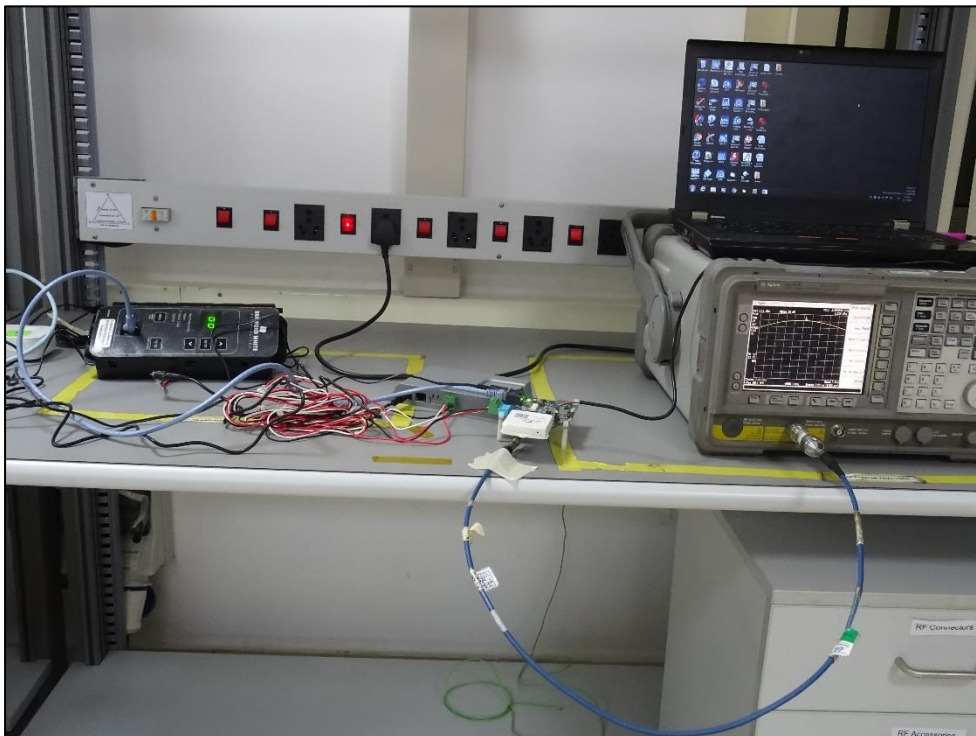
Antenna Port Test Setup Photo
