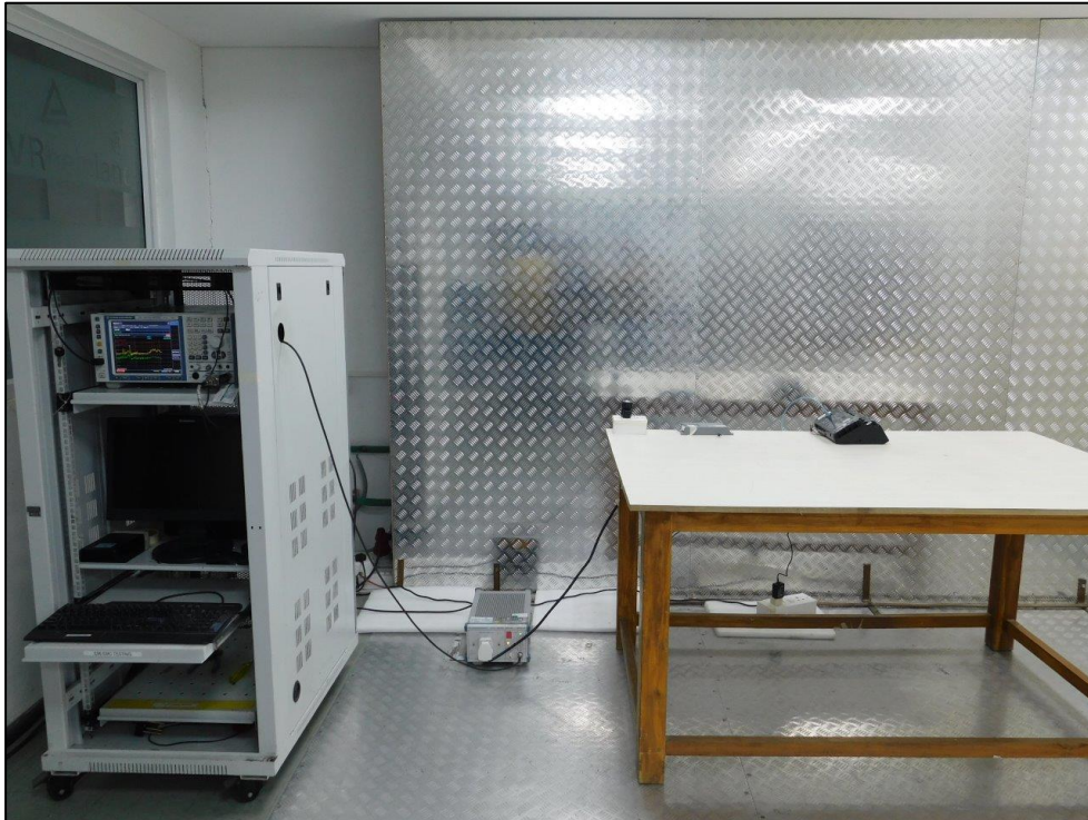
Conducted Emissions on AC Powerlines Test Setup
