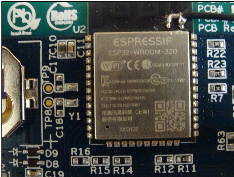
RF Module Close-up View
