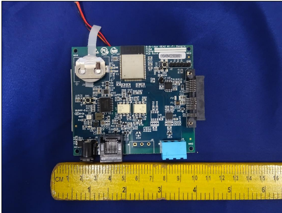
EUT PCB Dimensional View (Length)
