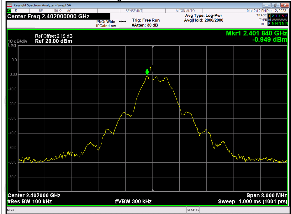
Band Edge NVNT 2402MHz Emission
