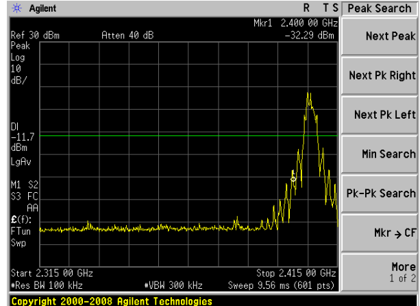
GFSK mode: Band Edge-Low Channel
