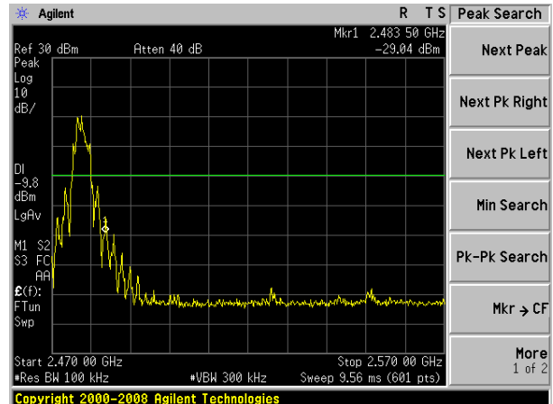
GFSK mode: Band Edge- High Channel
