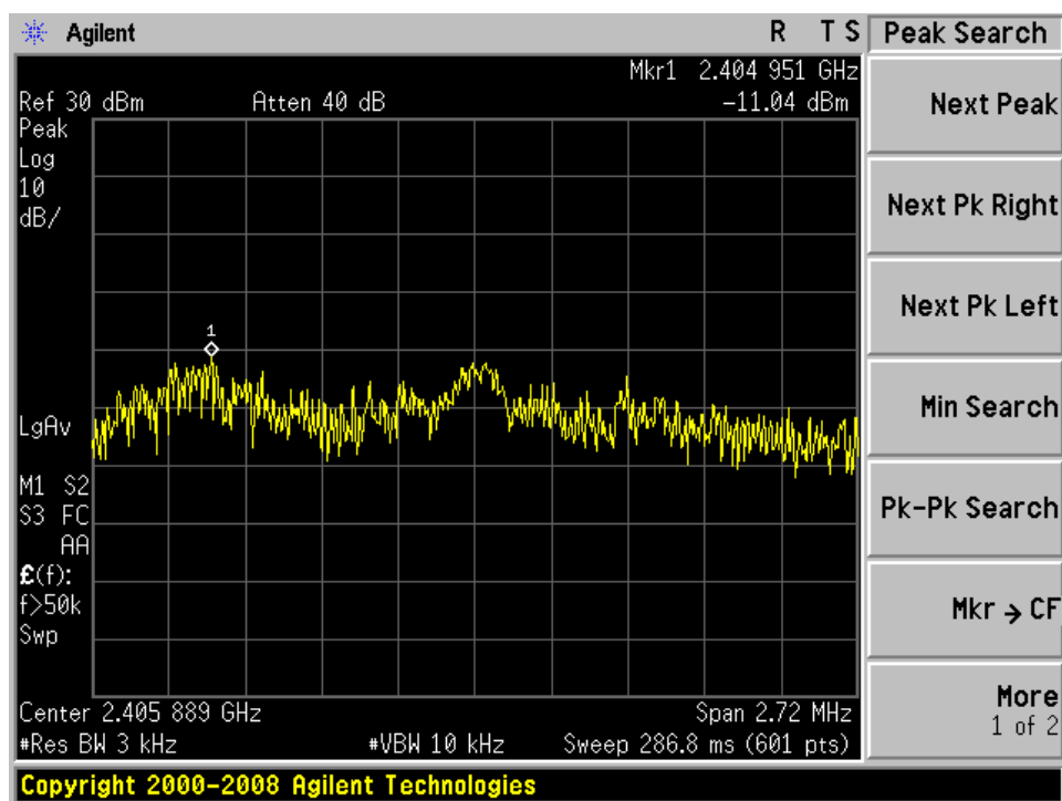
Power spectral density plot on channel Low
