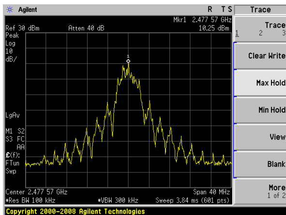
GFSK on channel High Channel
