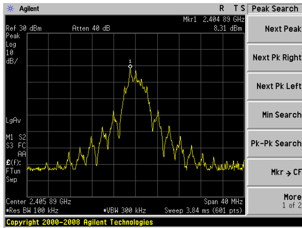
GFSK on channel Low Channel
