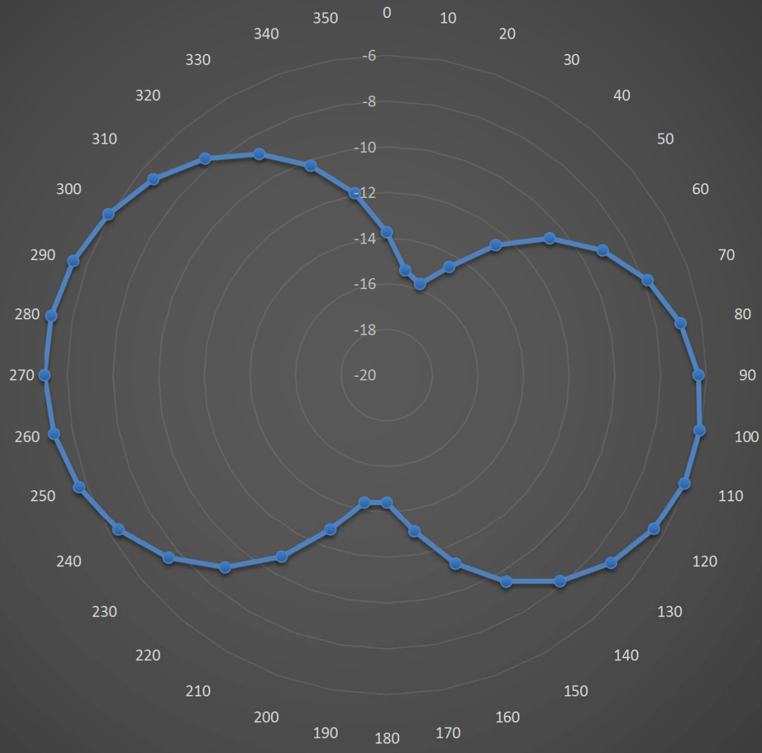
Freq='915MHz' Theta='90deg' dBi(GainTotal)
