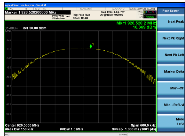
Peak output Power plot on channel 103(1Mbps)
