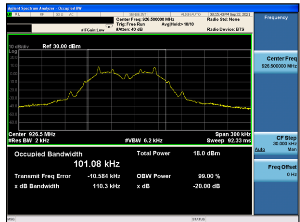
20dB Bandwidth plot on channel 103 (1Mbps)
