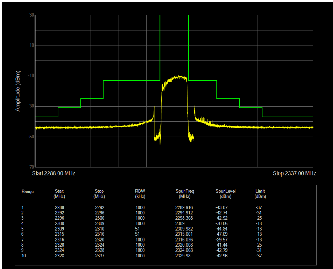
Band40a QPSK BW=10MHz Channel=38750 RB Size=1 Position=#Max
