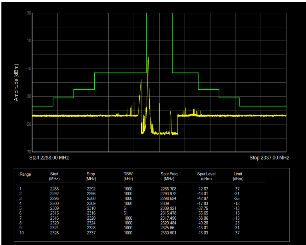
Band40a 16QAM BW=10MHz Channel=38750 RB Size=1 Position=#Max
