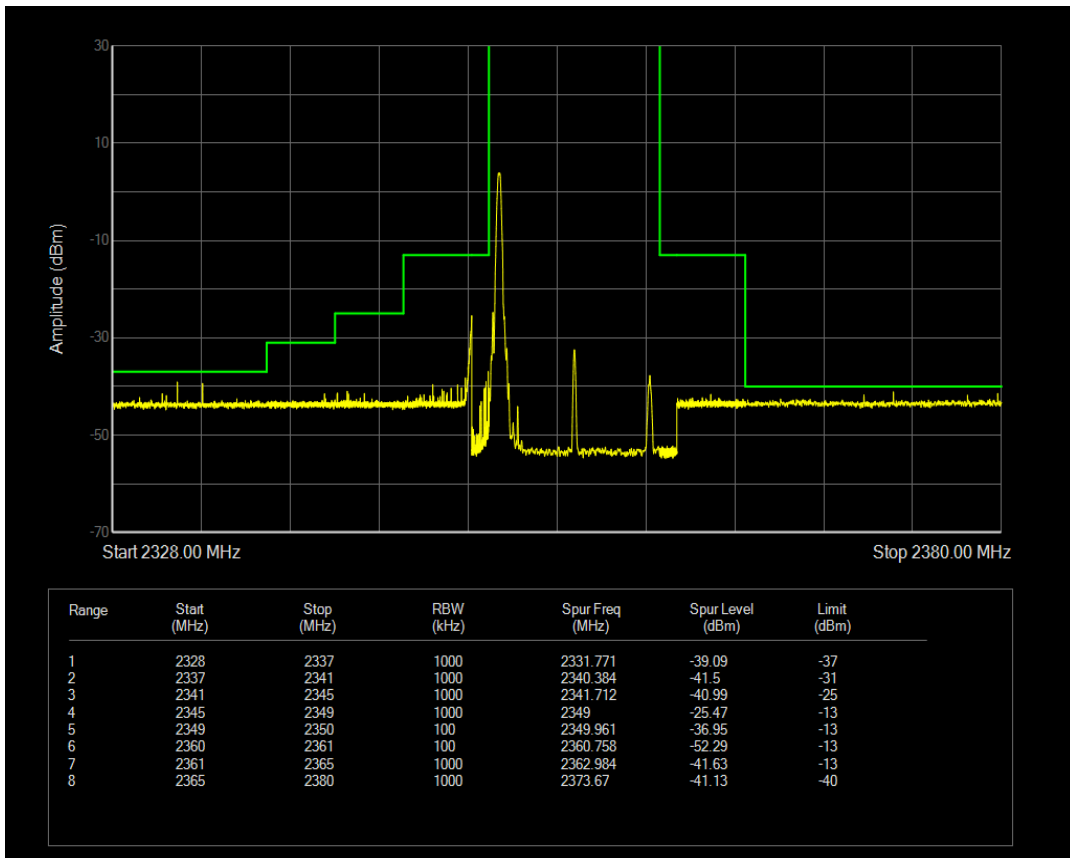
Band40b 16QAM BW=5MHz Channel=39225 RB Size=25 Position=#0
