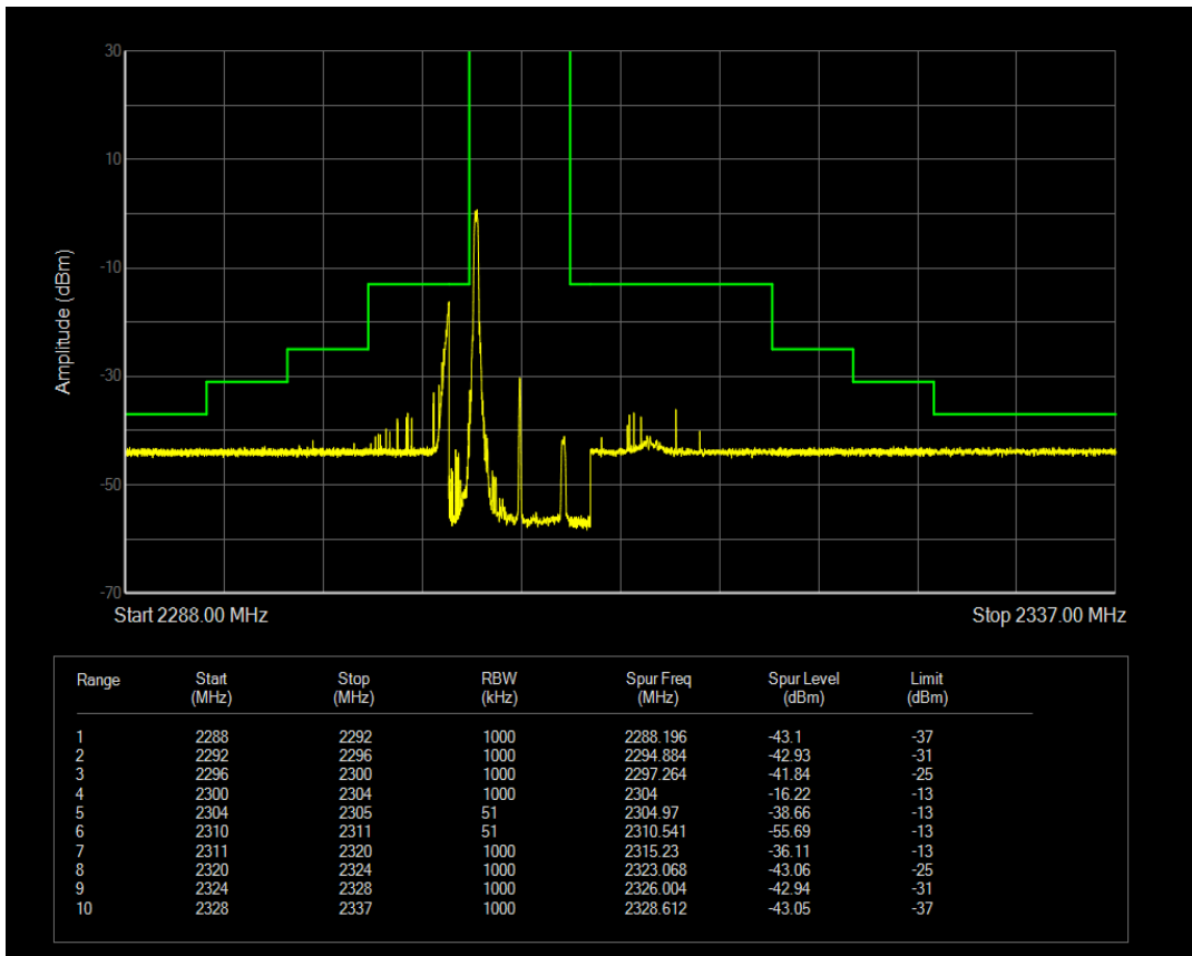
Band40a 16QAM BW=5MHz Channel=38725 RB Size=1 Position=#Max
