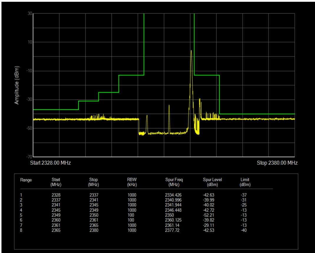
Band40b 16QAM BW=5MHz Channel=39225 RB Size=1 Position=#0
