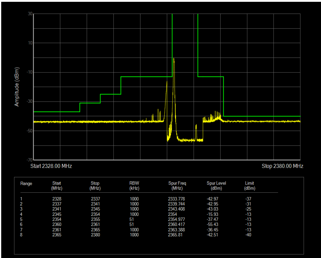
Band40b QPSK BW=5MHz Channel=39225 RB Size=1 Position=#Max
