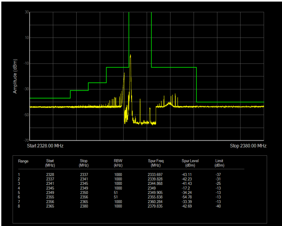
Band40b QPSK BW=5MHz Channel=39175 RB Size=1 Position=#Max
