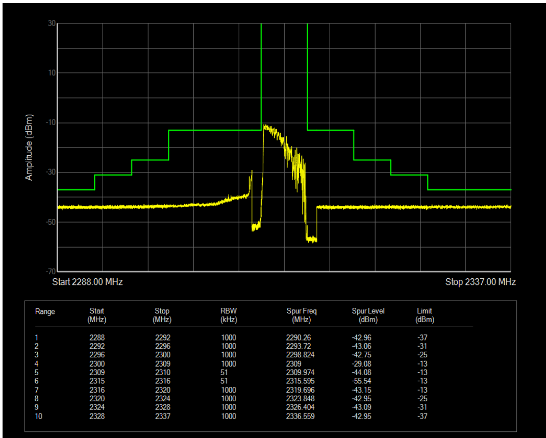
Band40a 16QAM BW=5MHz Channel=38775 RB Size=1 Position=#Max
