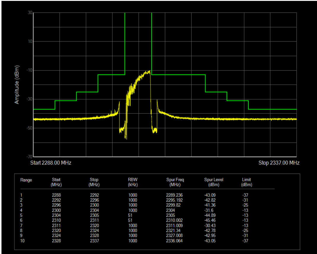
Band40a 16QAM BW=5MHz Channel=38775 RB Size=1 Position=#0
