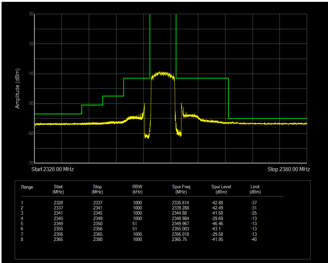
Band40b 16QAM BW=5MHz Channel=39175 RB Size=1 Position=#0
