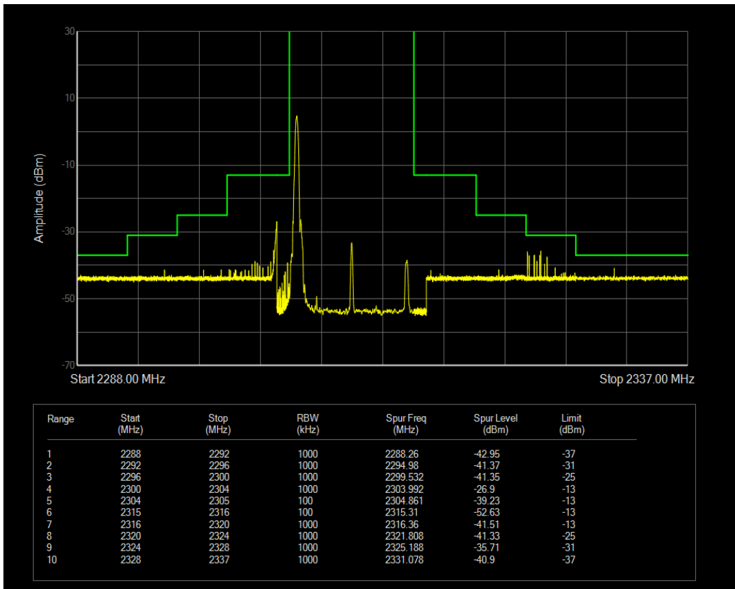
Band40a 16QAM BW=5MHz Channel=38775 RB Size=25 Position=#0
