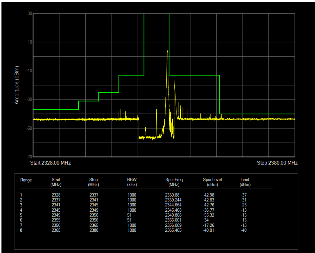
Band40b 16QAM BW=5MHz Channel=39175 RB Size=25 Position=#0
