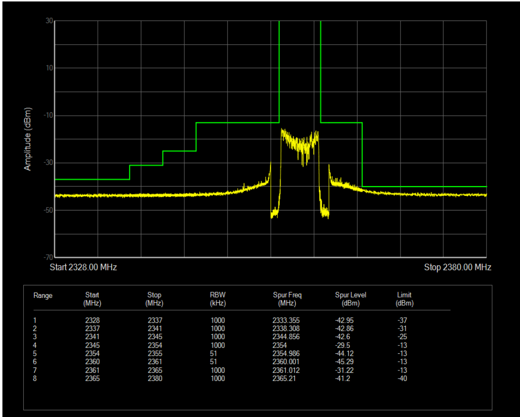
Band40b 16QAM BW=10MHz Channel=39200 RB Size=1 Position=#Max
