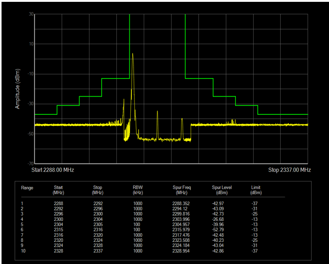
Band40a 16QAM BW=5MHz Channel=38725 RB Size=25 Position=#0
