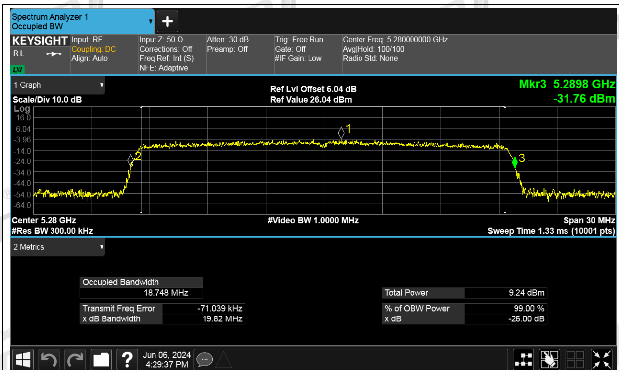
-26dB Bandwidth NVNT ax20 5280MHz Ant3
