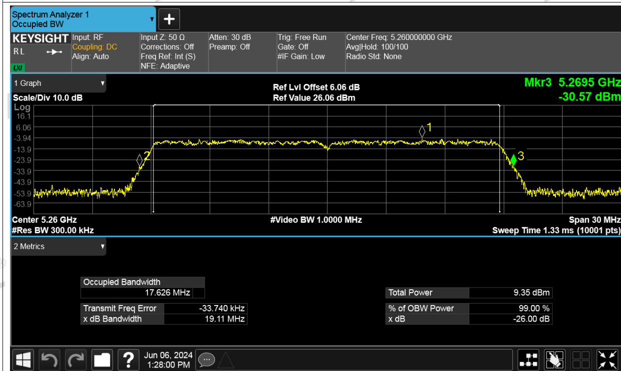
-26dB Bandwidth NVNT ac20 5260MHz Ant3
