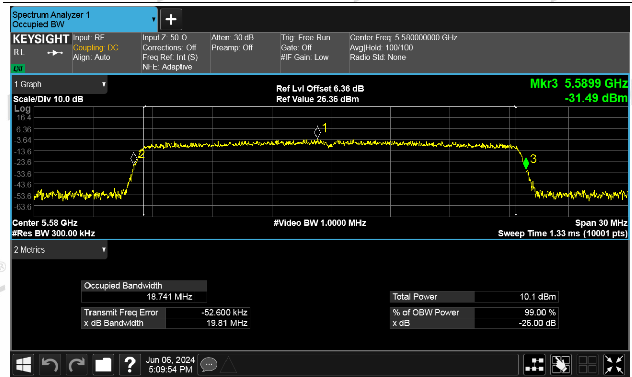
-26dB Bandwidth NVNT ax20 5580MHz Ant3
