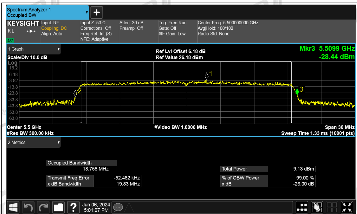
-26dB Bandwidth NVNT ax20 5500MHz Ant3
