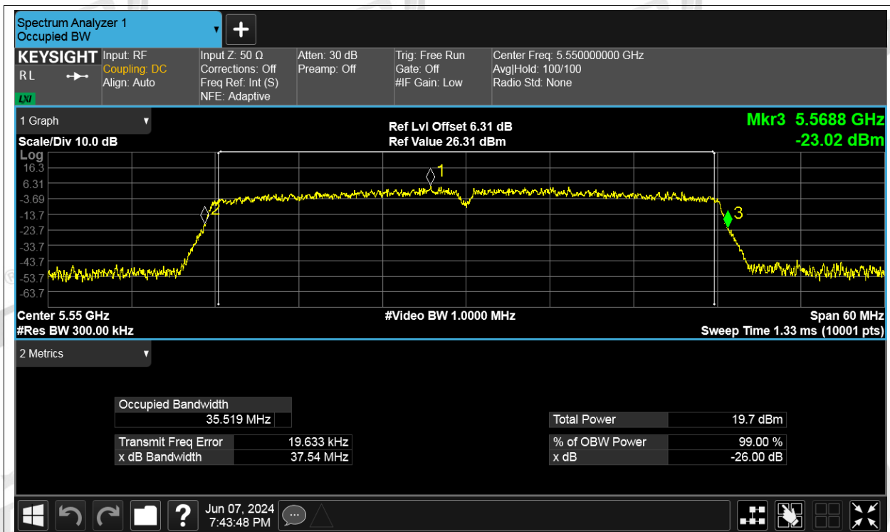
-26dB Bandwidth NVNT ac40 5550MHz Ant3
