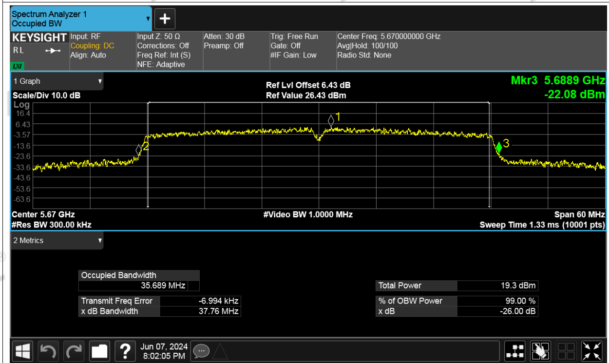
-26dB Bandwidth NVNT ac40 5670MHz Ant3
