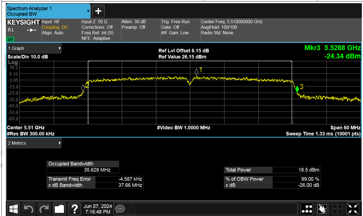
-26dB Bandwidth NVNT ac40 5510MHz Ant3
