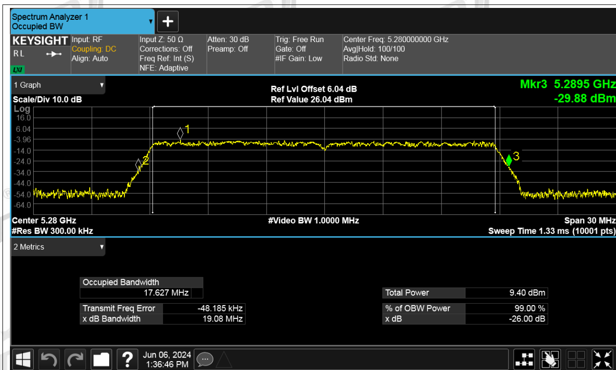
-26dB Bandwidth NVNT ac20 5280MHz Ant3
