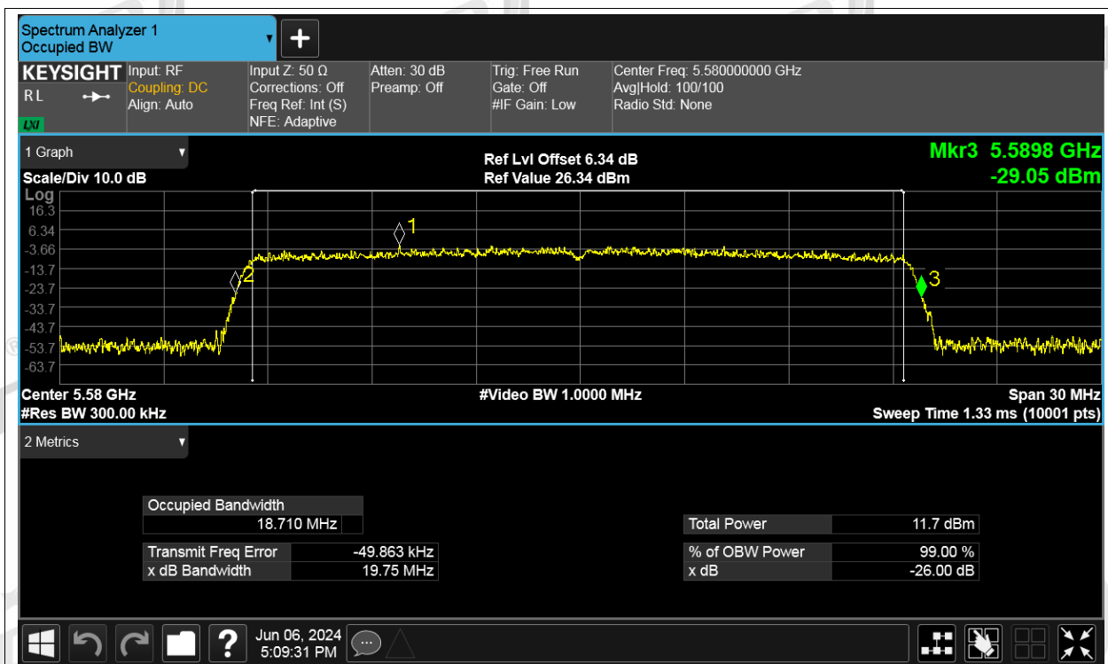
-26dB Bandwidth NVNT ax20 5580MHz Ant2
