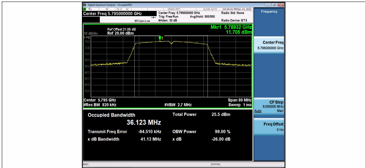
11N40MIMO Ant2 5795
