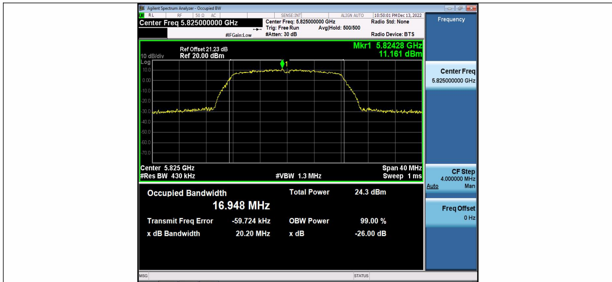
11A Ant2 5825
