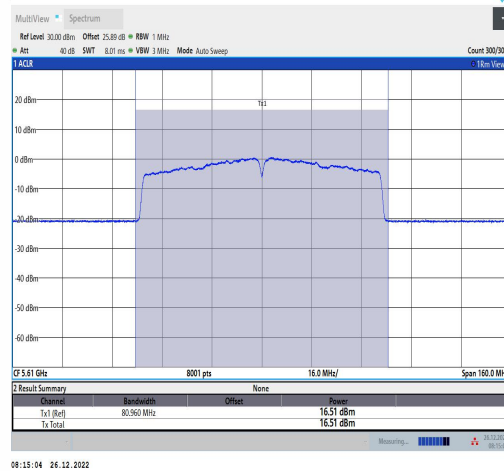
11AC80MIMO-Ant2-5610-TPC L-----15.32-76.00-1.19
