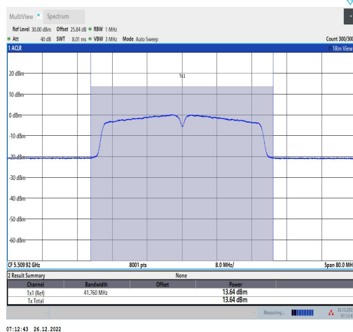
11AC40MIMO-Ant1-5510-TPC L-----12.95-85.37-0.69
