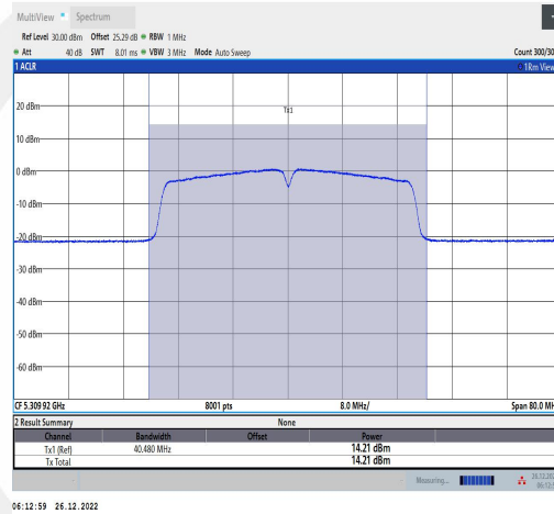
11N40MIMO-Ant2-5310-TPC L-----13.83-91.55-0.38
