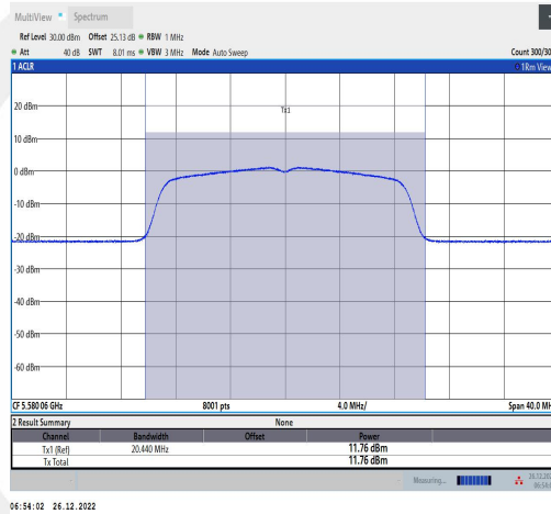
11AC20MIMO-Ant1-5580-TPC L-----11.39-91.89-0.37
