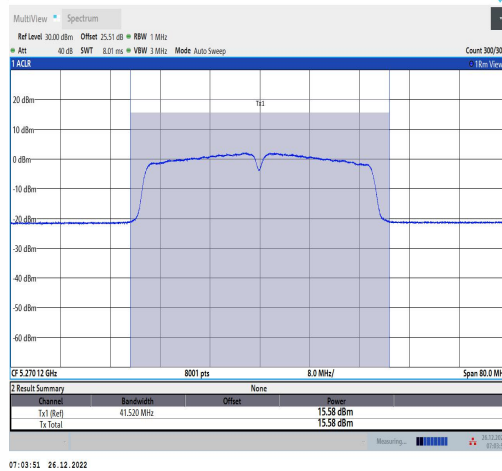
11AC40MIMO-Ant1-5270-TPC L-----14.89-85.37-0.69
