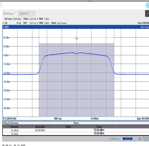
11AC20MIMO-Ant1-5260-TPC L-----13.17-91.89-0.37
