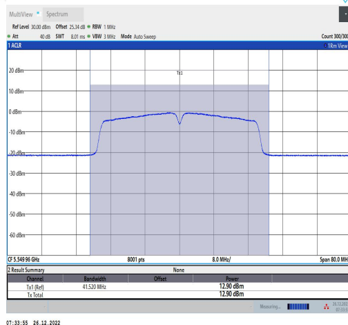
11AC40MIMO-Ant1-5550-TPC L-----12.32-87.50-0.58
