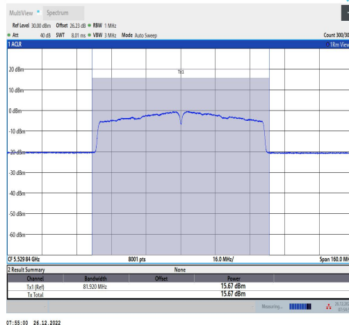
11AC80MIMO-Ant1-5530-TPC L-----14.48-76.00-1.19
