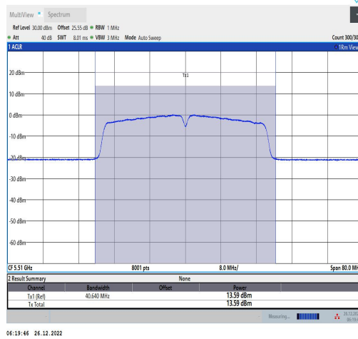
11N40MIMO-Ant2-5510-TPC L-----13.27-92.86-0.32
