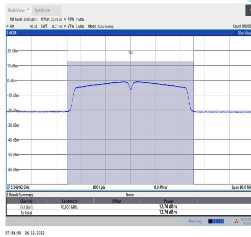
11AC40MIMO-Ant2-5550-TPC L-----12.05-85.37-0.69
