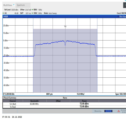
11AC80MIMO-Ant1-5290-TPC L-----14.43-79.17-1.01
