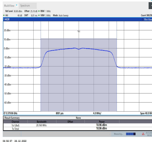
11AC20MIMO-Ant2-5580-TPC L-----10.59-91.89-0.37
