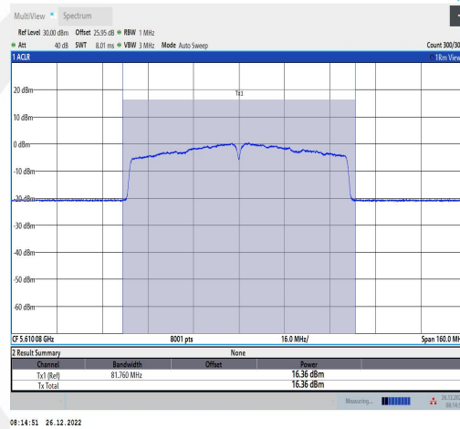
11AC80MIMO-Ant1-5610-TPC L-----15.17-76.00-1.19
