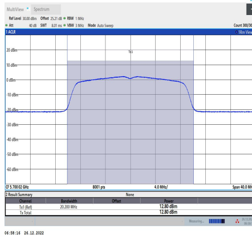
11AC20MIMO-Ant1-5700-TPC L-----12.50-93.24-0.30
