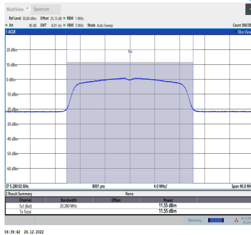
11AC20MIMO-Ant2-5280-TPC L-----11.18-91.89-0.37
