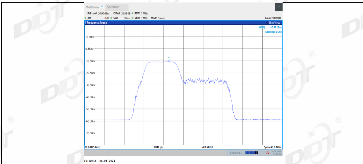
11BE20MIMO Ant1_6895_52+26_2
