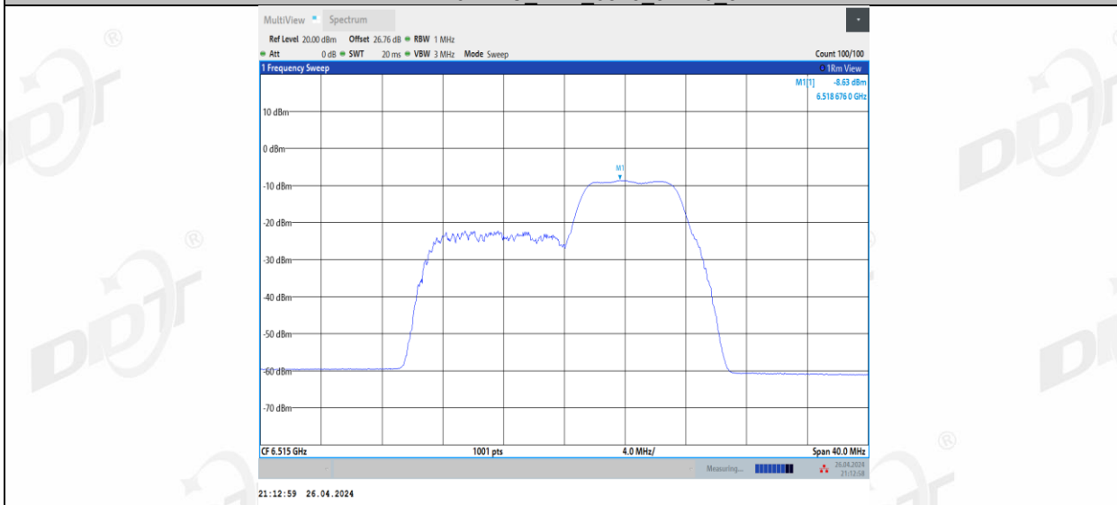
11BE20MIMO Ant2_6515_106+26_1
