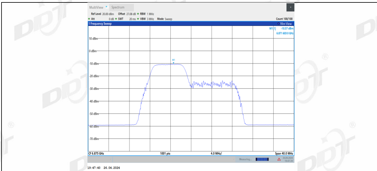
11BE20MIMO Ant1_6875_52+26_2
