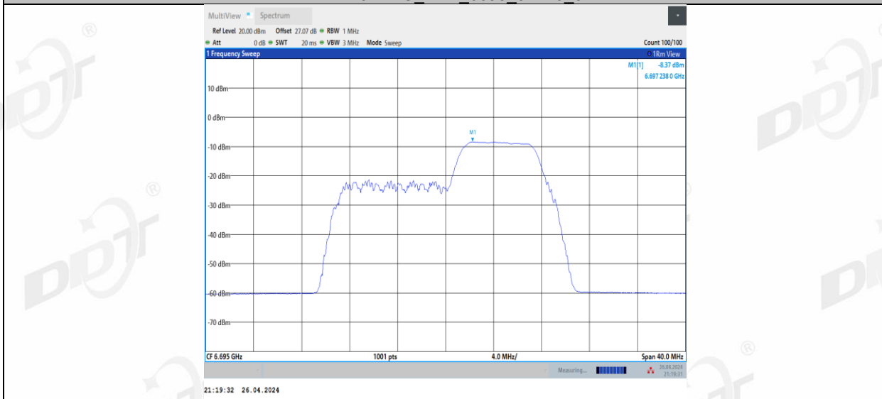
11BE20MIMO Ant2_6695_106+26_1
