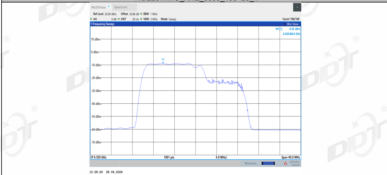
11BE20MIMO Ant2_6535_106+26_2
