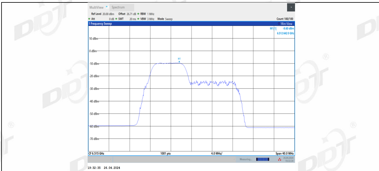
11BE20MIMO Ant1_6515_52+26_2
