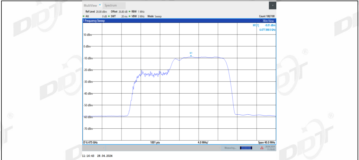
11BE20MIMO Ant3 6475 52+26_1
