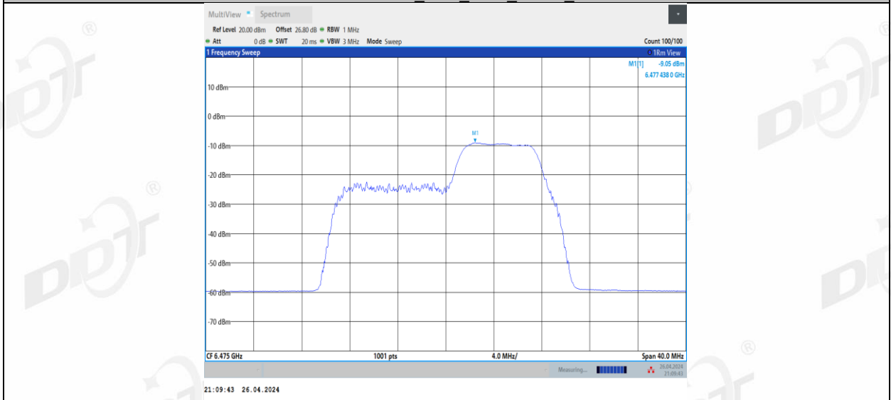
11BE20MIMO Ant2_6475_106+26_1
