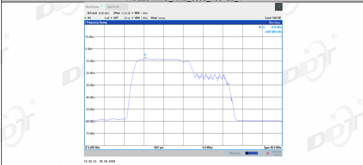
11BE20MIMO Ant2_6695_106+26_2
