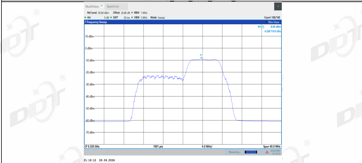
11BE20MIMO Ant2_6535_106+26_1
