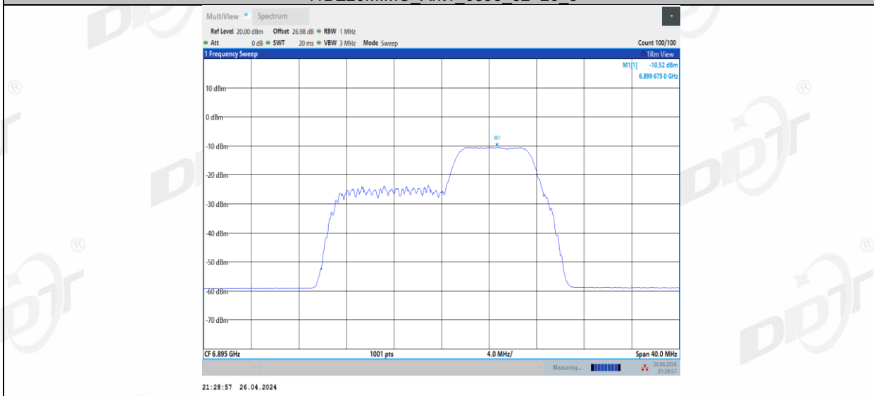
11BE20MIMO Ant1_6895_106+26_1
