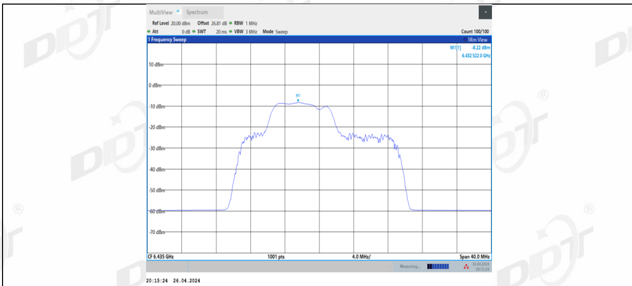
11BE20MIMO Ant2_6435_52+26_3
