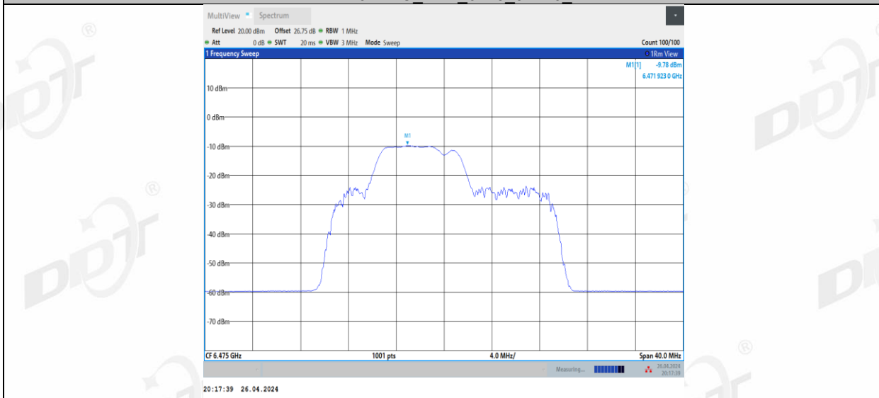
11BE20MIMO Ant1_6475_52+26_3
