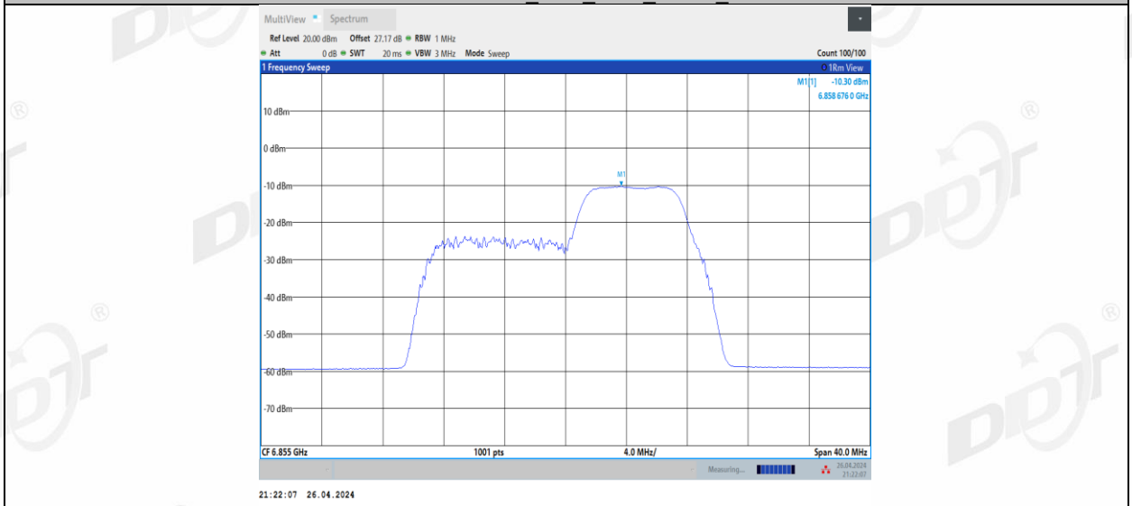
11BE20MIMO Ant1_6855_106+26_1
