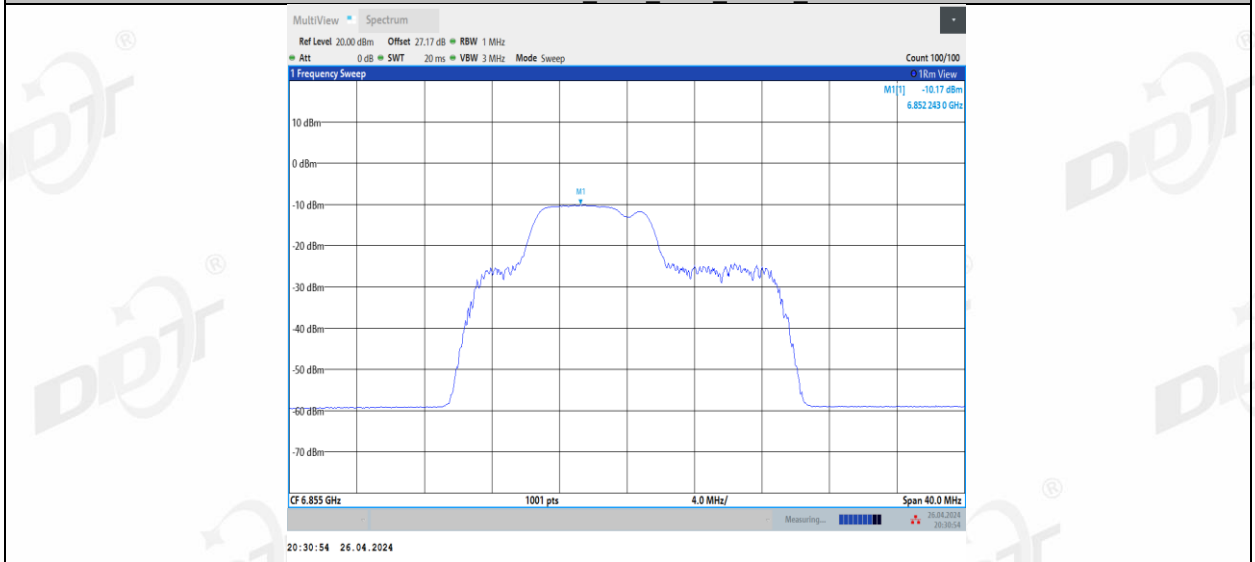
11BE20MIMO Ant1_6855_52+26_3
