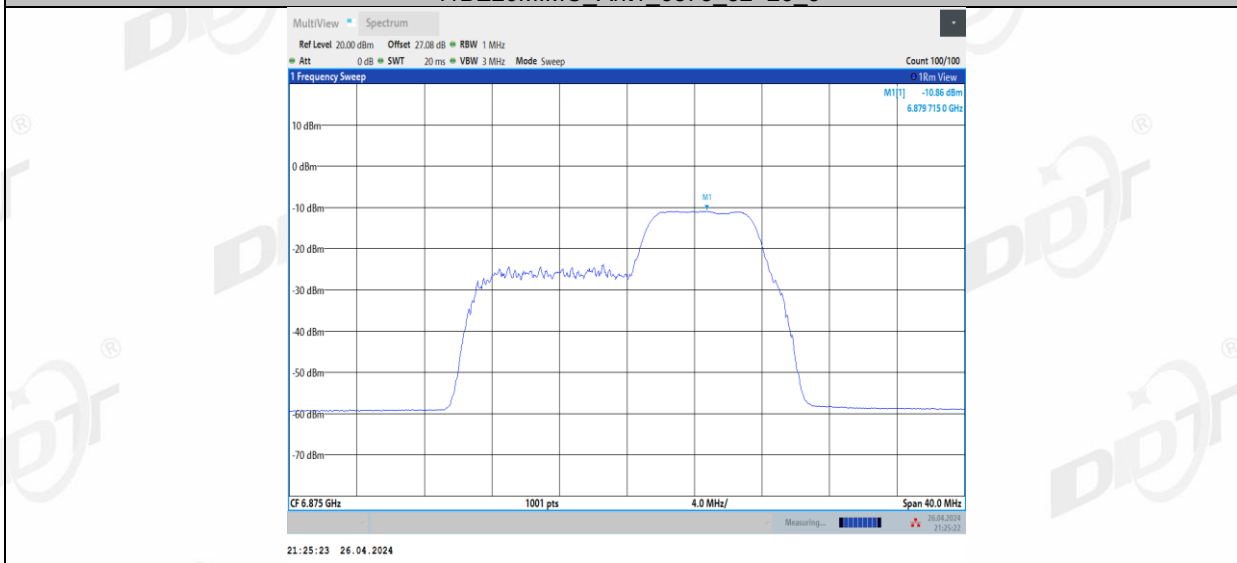
11BE20MIMO Ant1_6875_106+26_1
