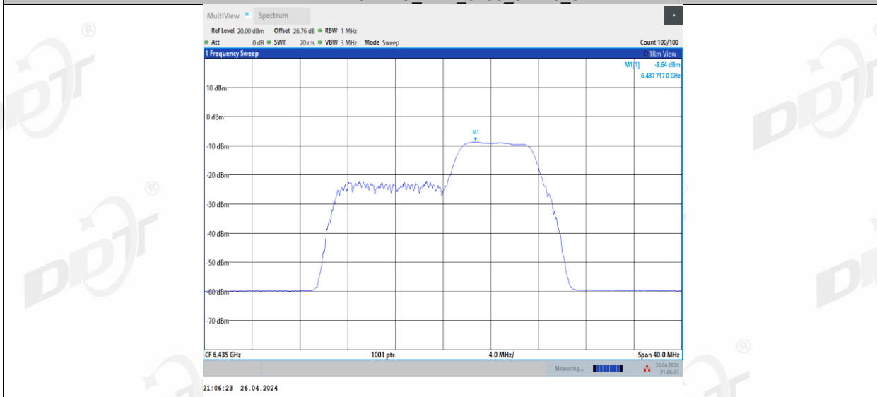
11BE20MIMO Ant2_6435_106+26_1
