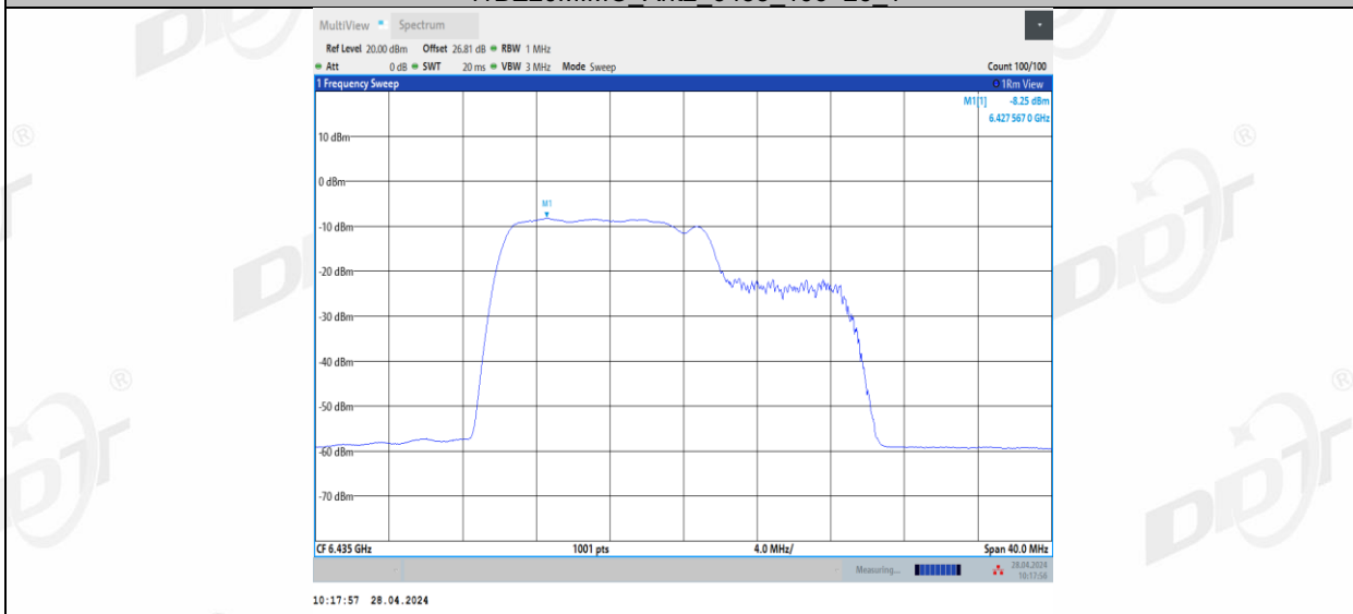
11BE20MIMO Ant2_6435_106+26_2
