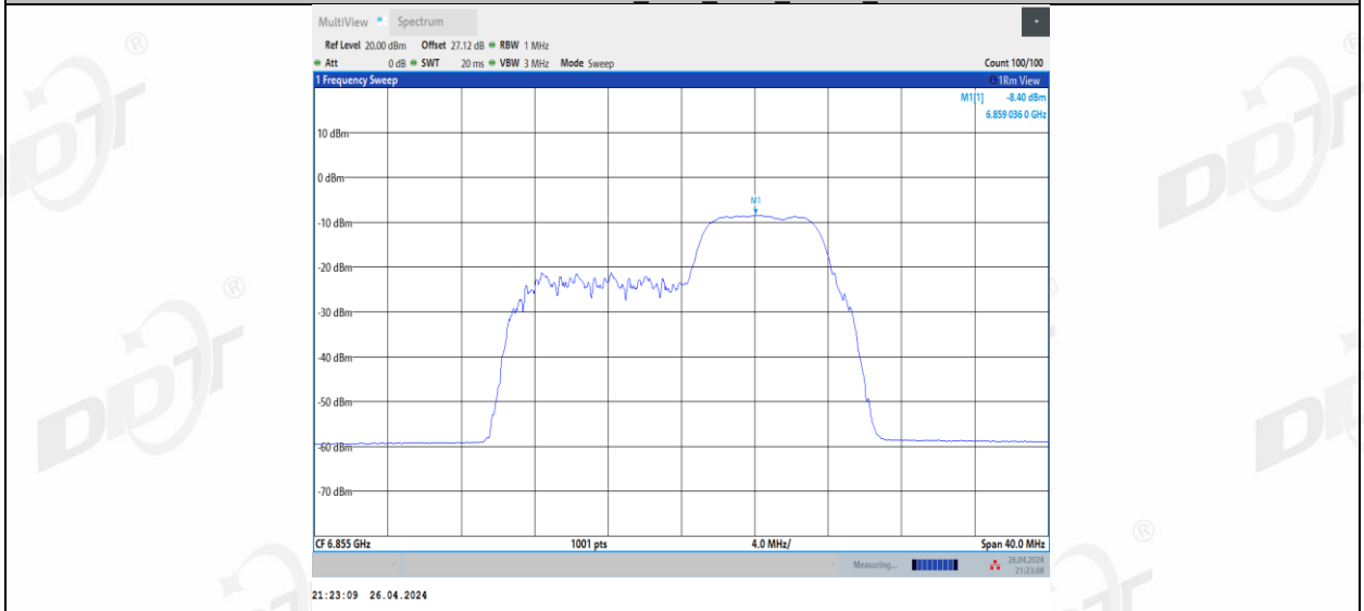
11BE20MIMO Ant2_6855_106+26_1
