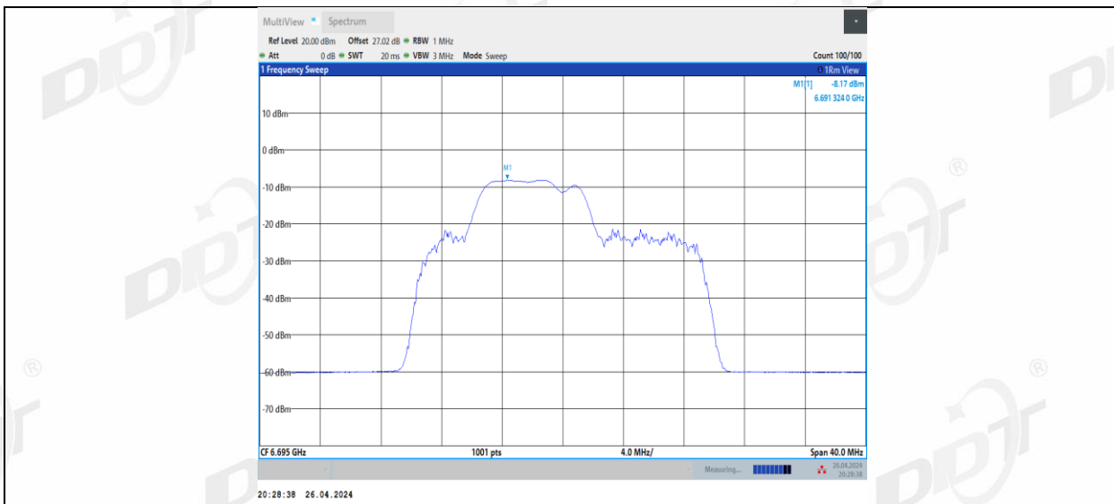
11BE20MIMO Ant2_6695_52+26_3
