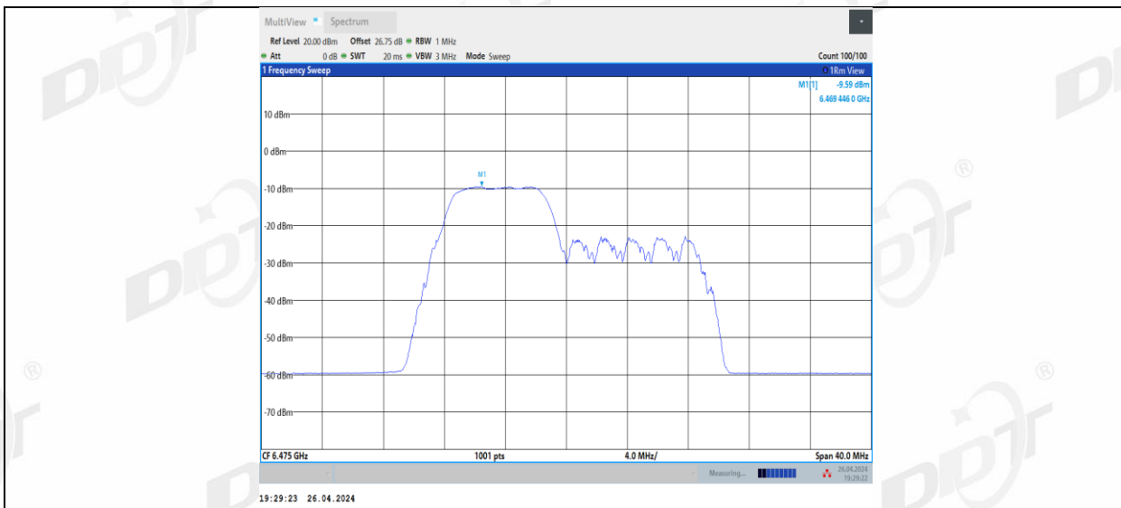
11BE20MIMO Ant1_6475_52+26_2
