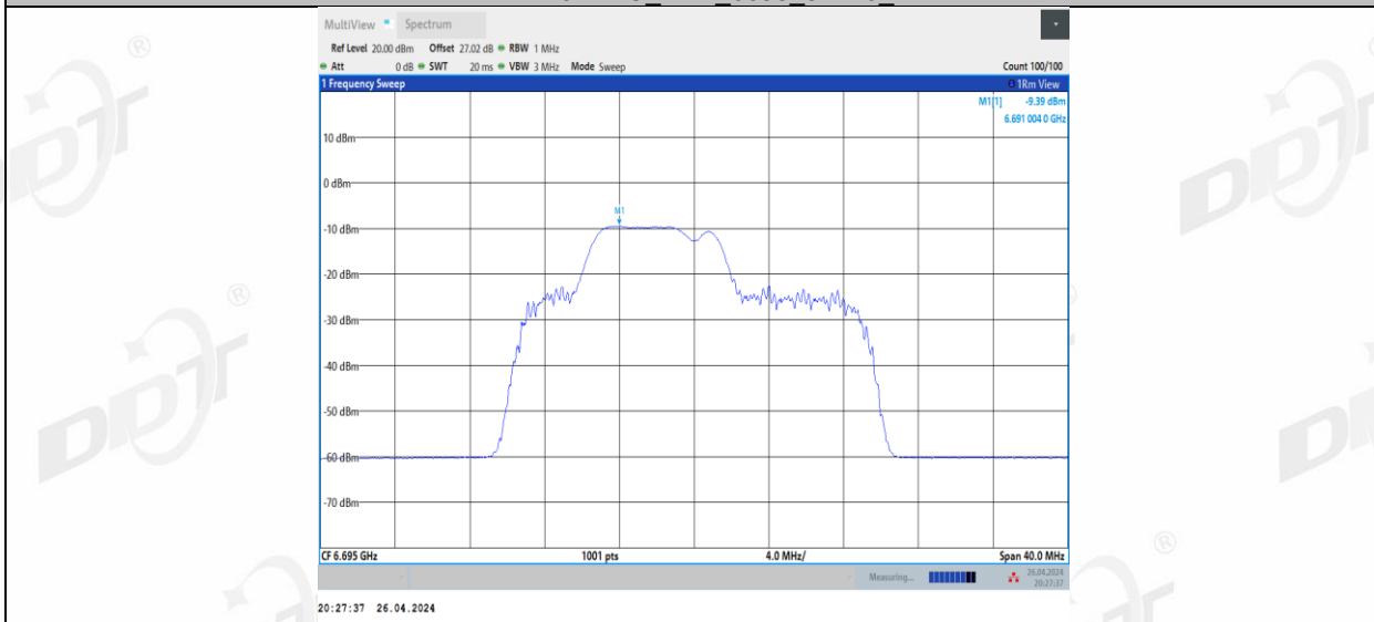
11BE20MIMO Ant1_6695_52+26_3
