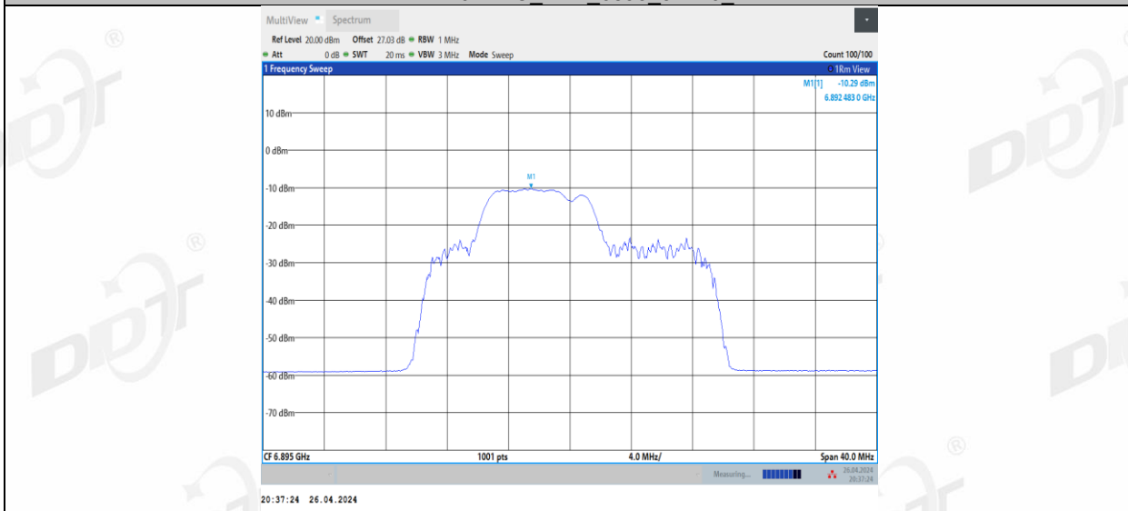
11BE20MIMO Ant1_6895_52+26_3
