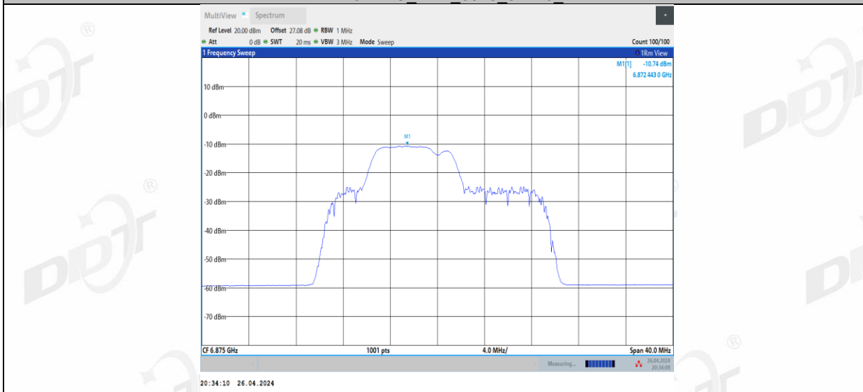
11BE20MIMO Ant1_6875_52+26_3
