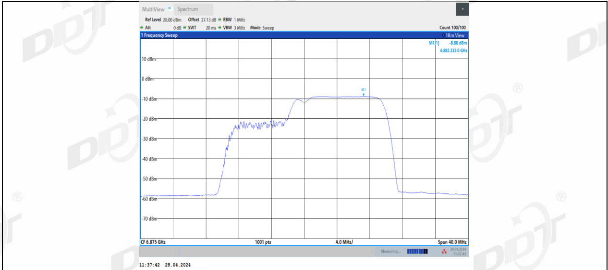
11BE20MIMO Ant3 6875 52+26_1
