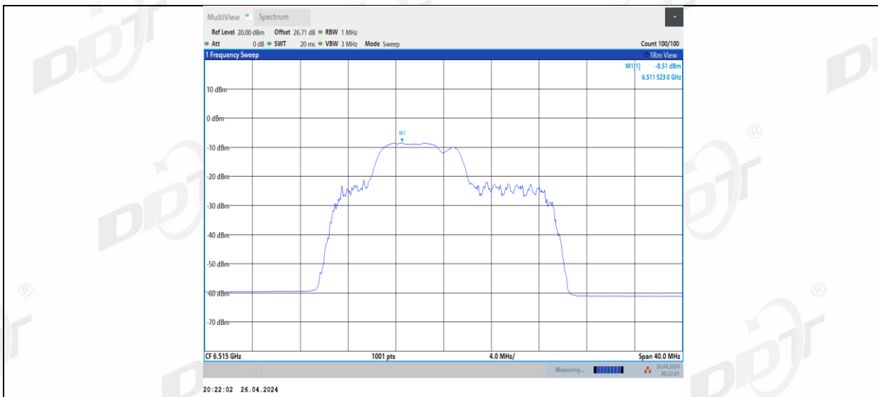
11BE20MIMO Ant2_6515_52+26_3
