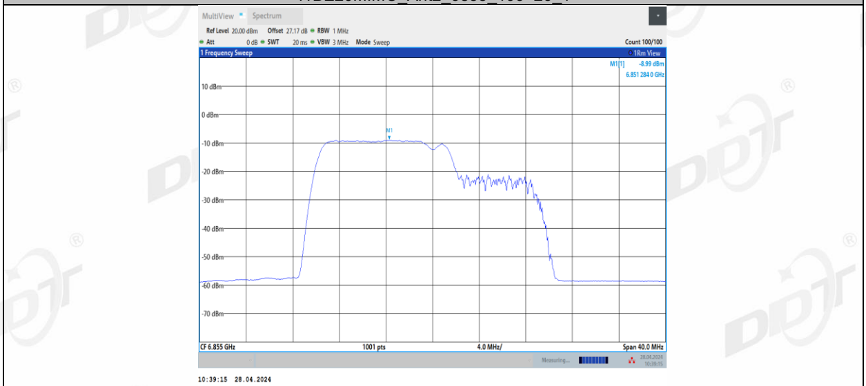
11BE20MIMO Ant2_6855_106+26_2
