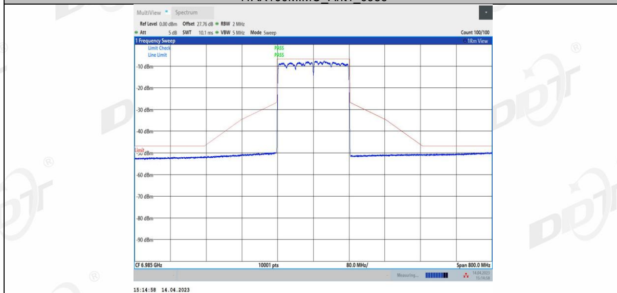
11AX160MIMO Ant2 6985
