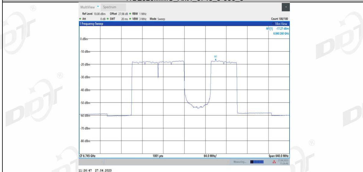
11BE320MIMO Ant4_6745_3*996_4
