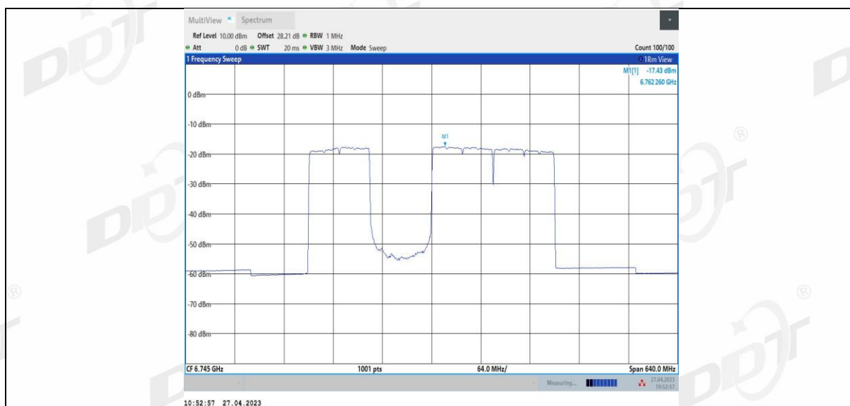
11BE320MIMO Ant1_6745_3*996_3
