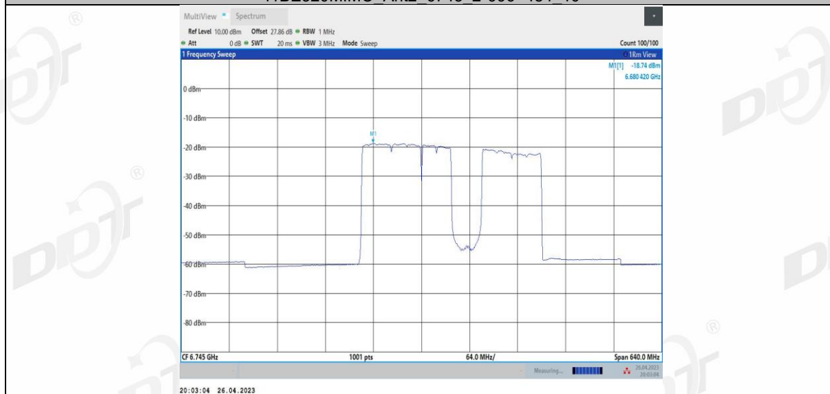
11BE320MIMO Ant2_6745_2*996+484_11
