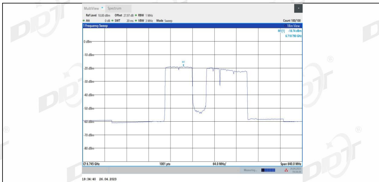
11BE320MIMO Ant2_6745_2*996+484_10
