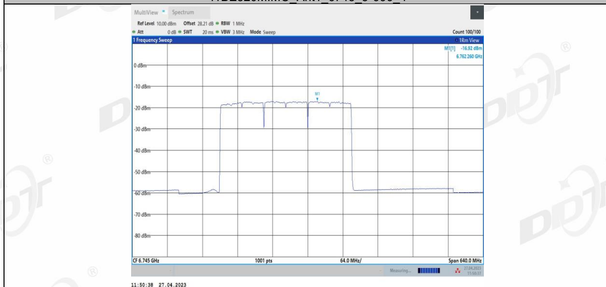
11BE320MIMO Ant1_6745_3*996+484_5
