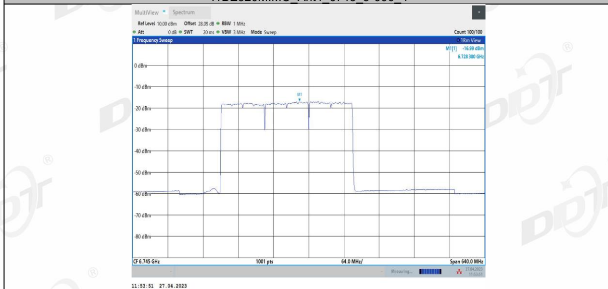
11BE320MIMO Ant4_6745_3*996+484_5
