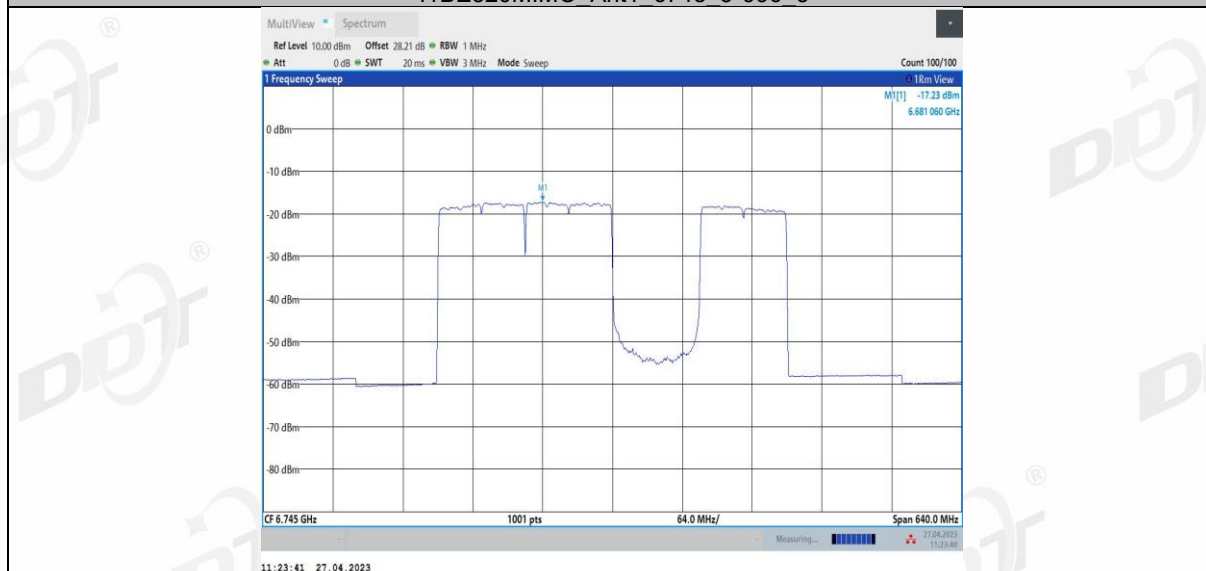
11BE320MIMO Ant1_6745_3*996_4
