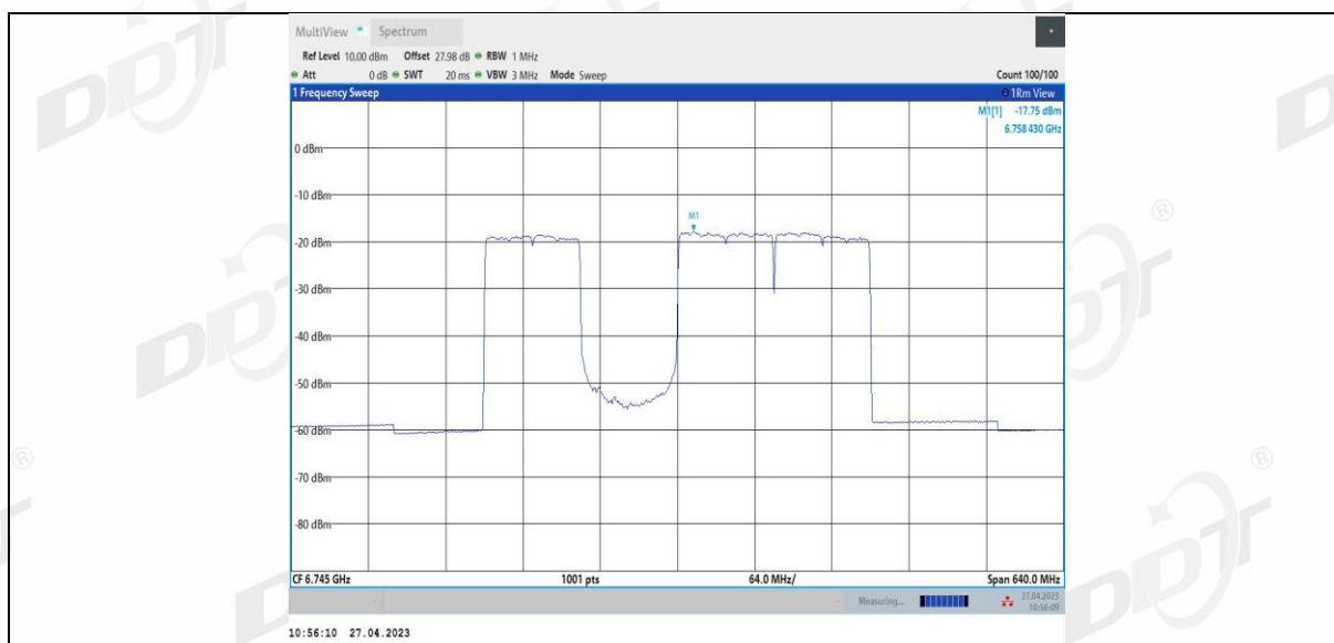
11BE320MIMO Ant4_6745_3*996_3
