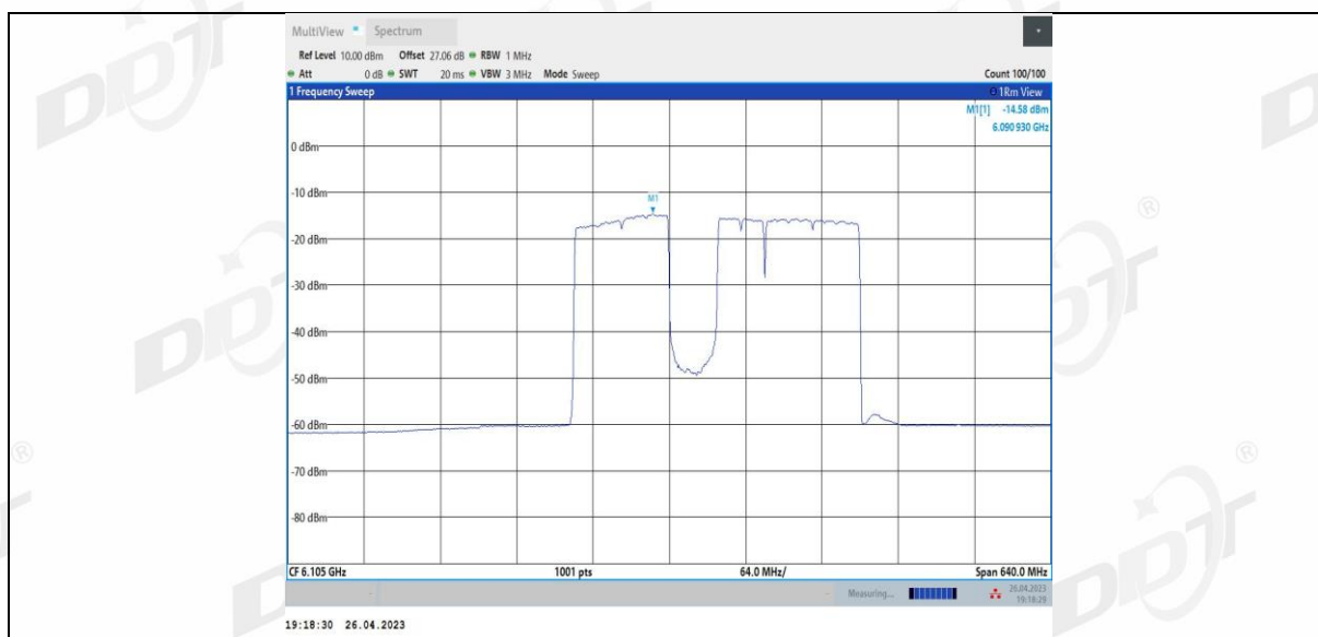
11BE320MIMO Ant2_6105_2*996+484_10
