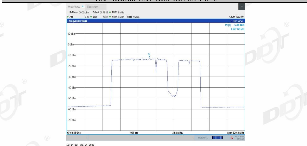
11BE160MIMO Ant4 6985_996+484+242_7
