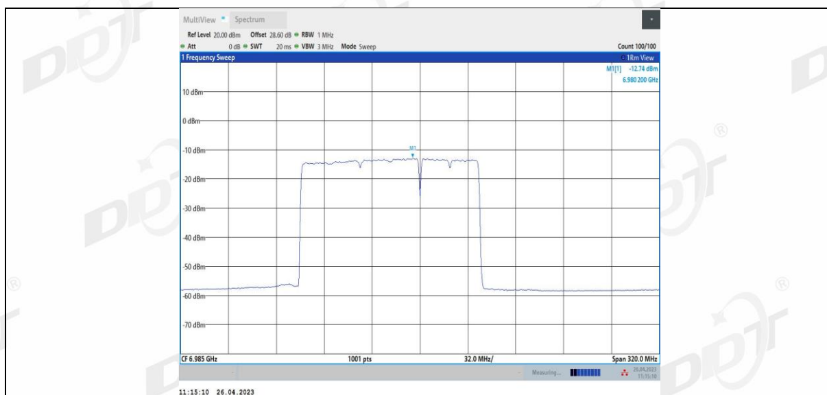
11BE160MIMO Ant1 6985 996+484+242 5
