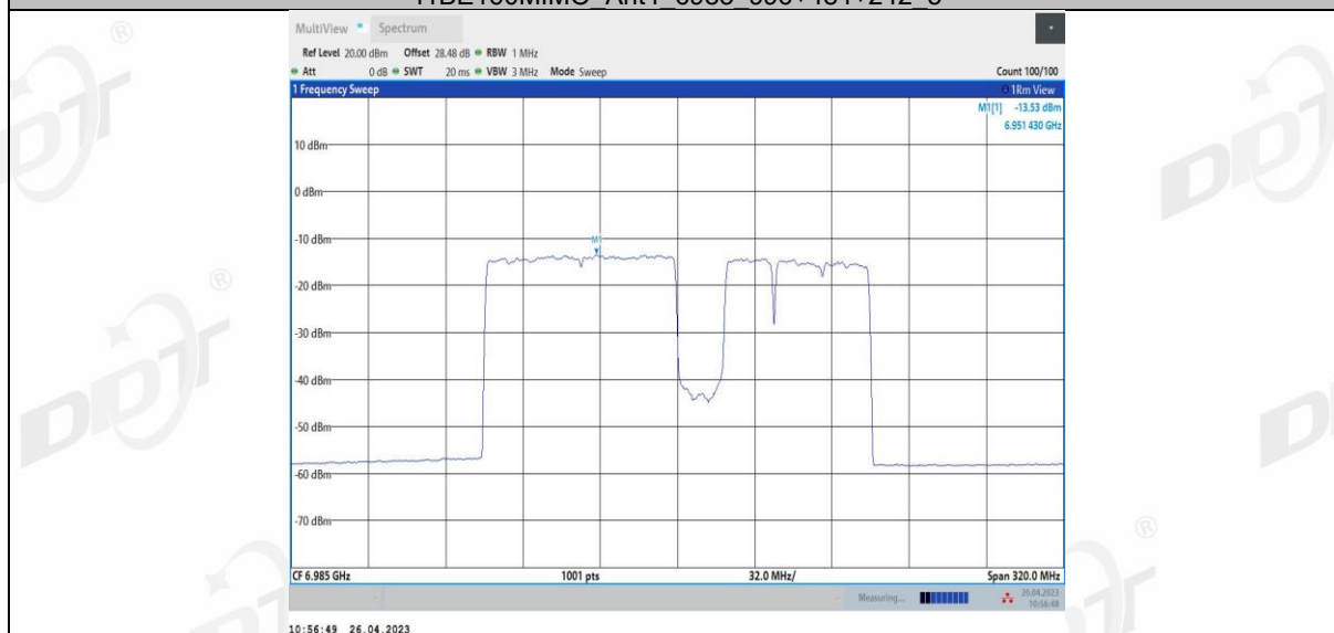
11BE160MIMO Ant4 6985_996+484+242_6
