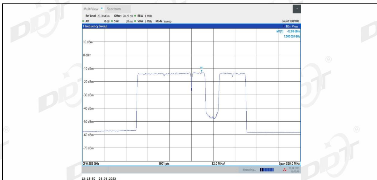
11BE160MIMO Ant3 6985 996+484+242 7
