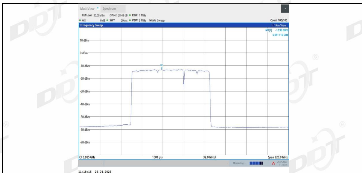
11BE160MIMO Ant4 6985_996+484+242_5
