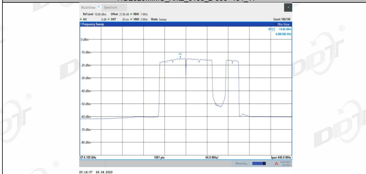
11BE320MIMO Ant2_6105_2*996+484_12
