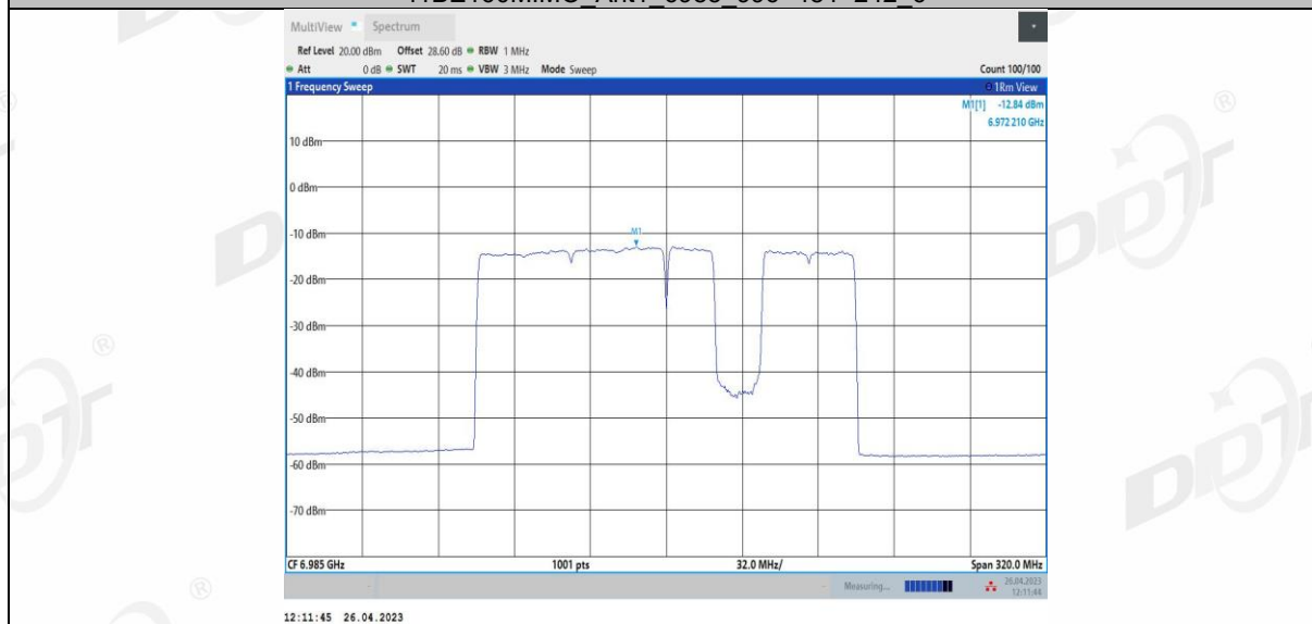
11BE160MIMO Ant1 6985 996+484+242 7
