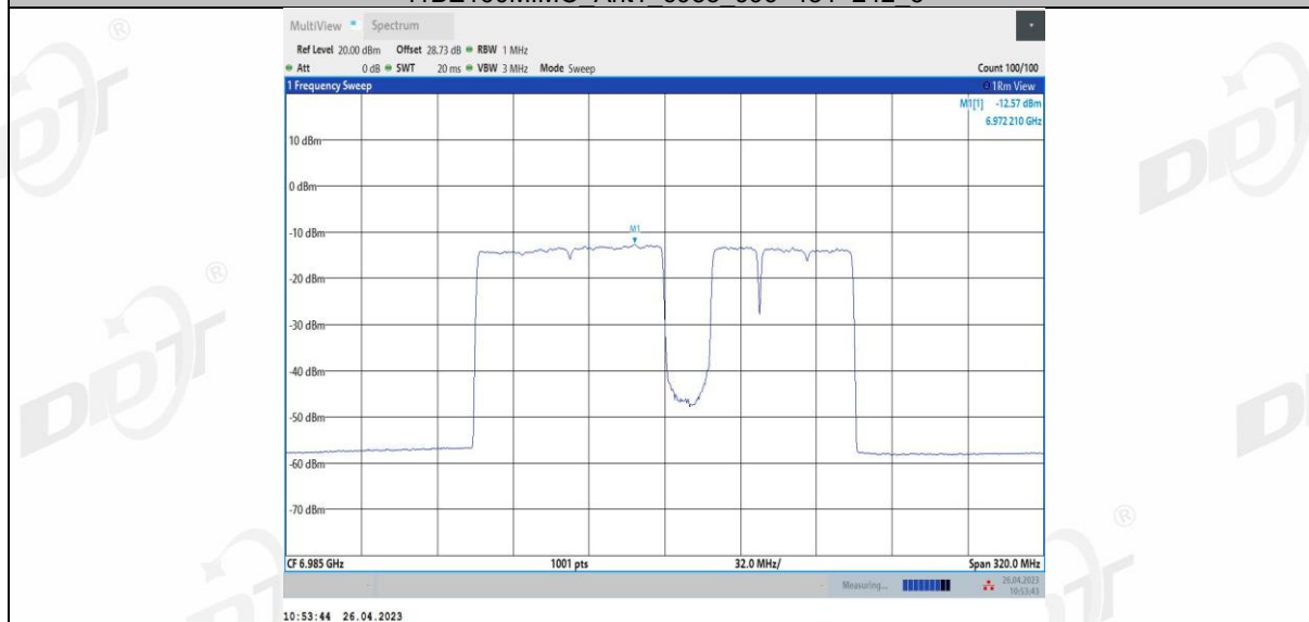
11BE160MIMO Ant1 6985 996+484+242 6
