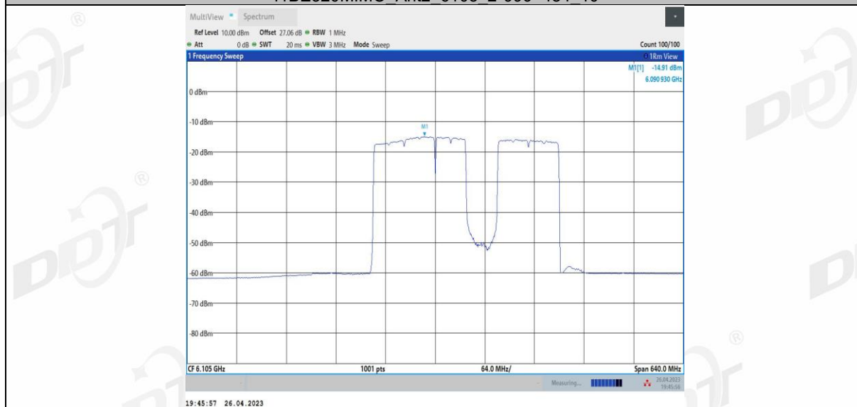
11BE320MIMO Ant2_6105_2*996+484_11
