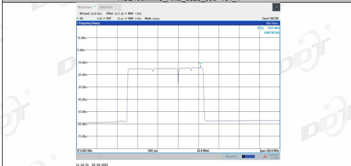
11BE160MIMO Ant3 6825 996+484+242_5
