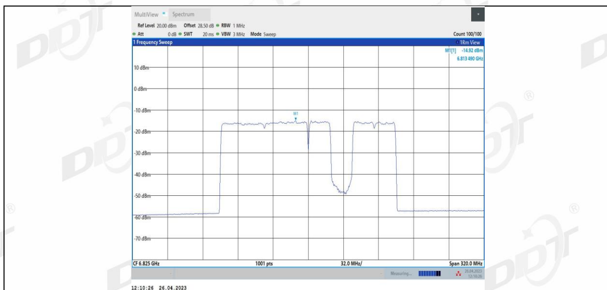
11BE160MIMO Ant4 6825_996+484+242_7
