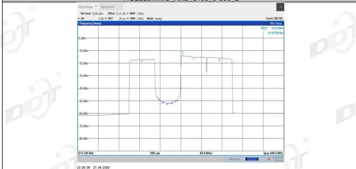
11BE320MIMO Ant3_6105_3*996_3
