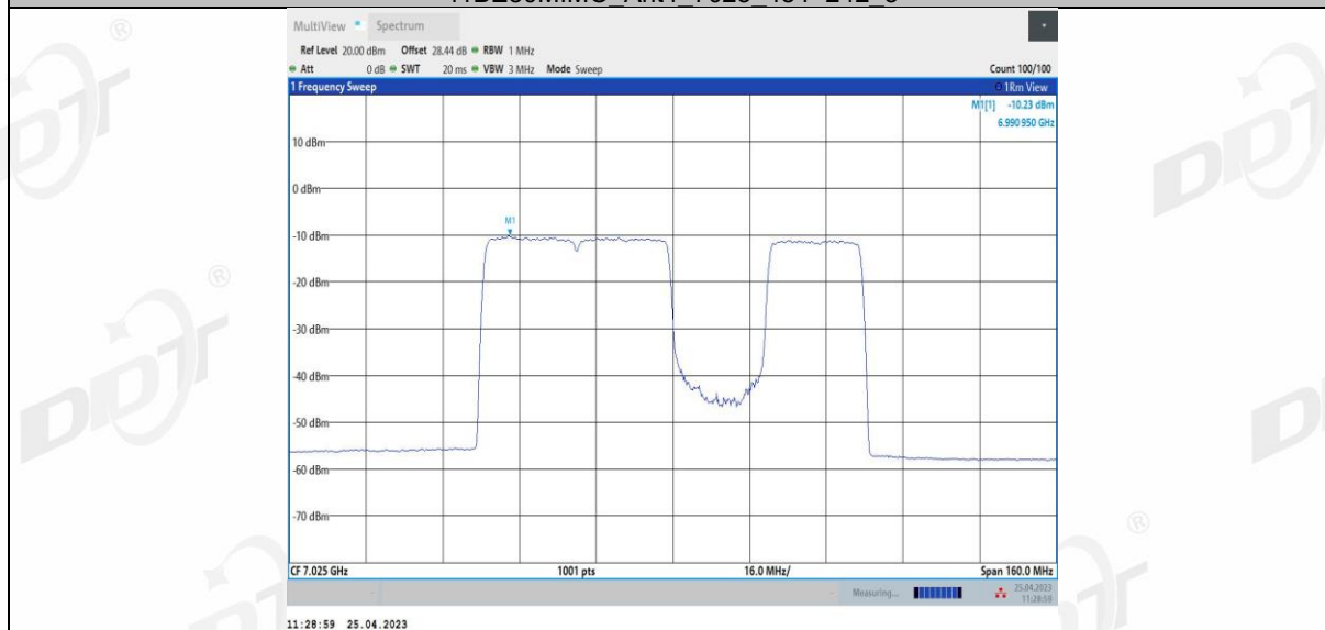
11BE80MIMO Ant4_7025_484+242_4
