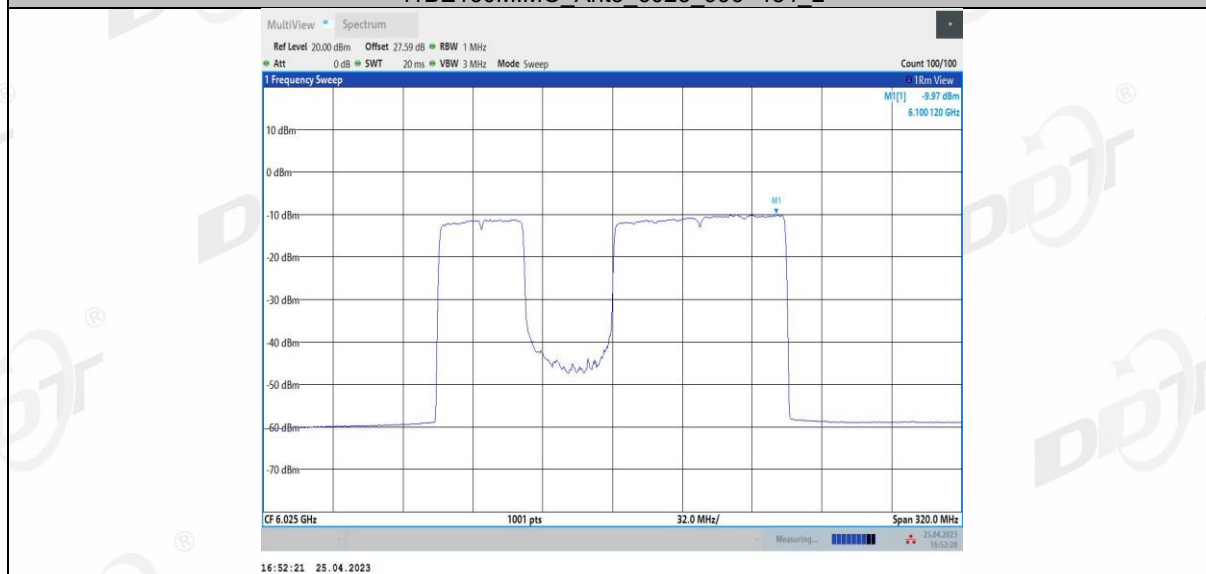
11BE160MIMO Ant3_6025_996+484_3
