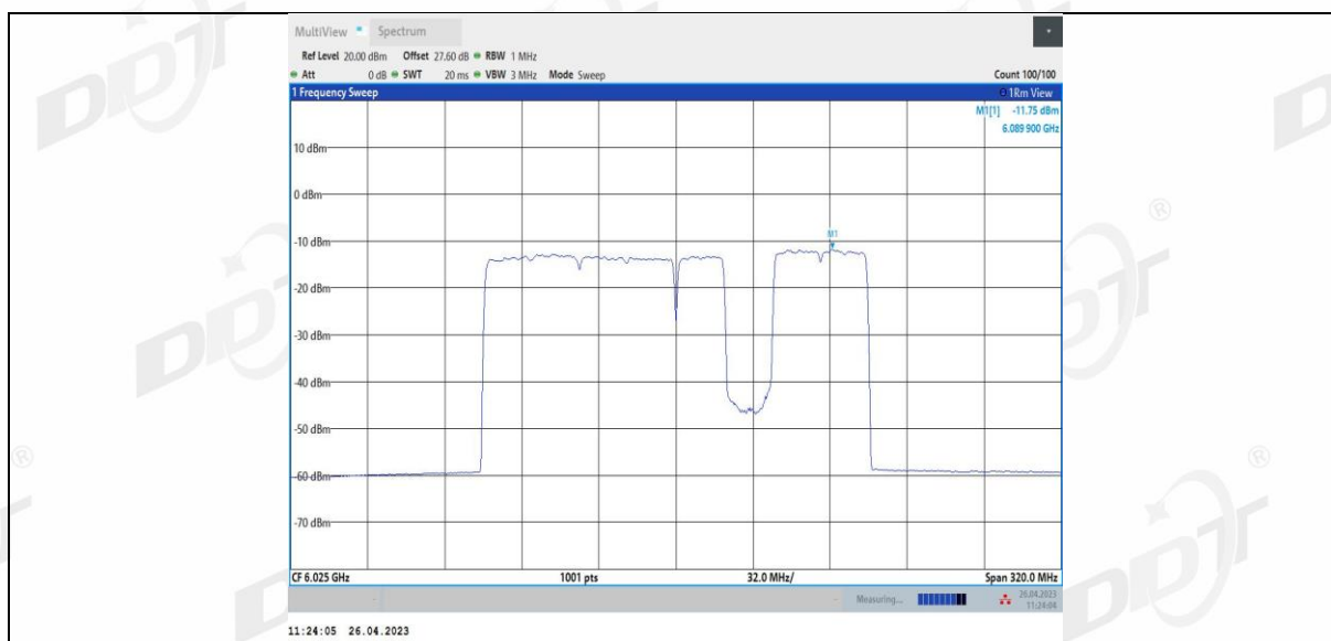
11BE160MIMO Ant3 6025_996+484+242_7
