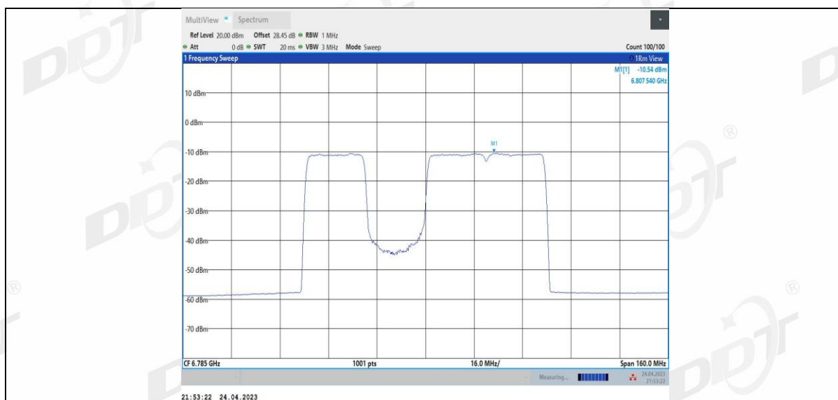
11BE80MIMO Ant4 6785 484+242_3
