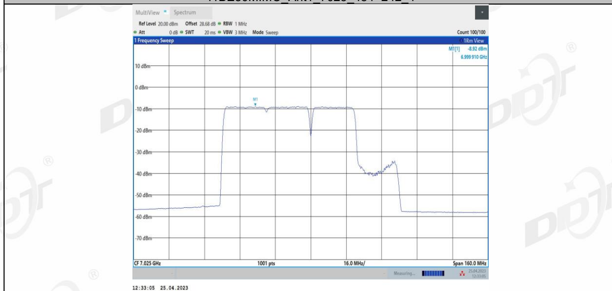
11BE80MIMO Ant2 7025 484+242_1
