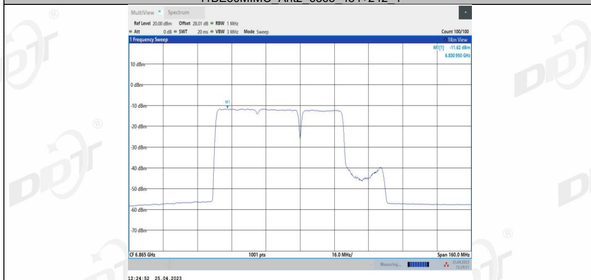
11BE80MIMO Ant3 6865 484+242 1
