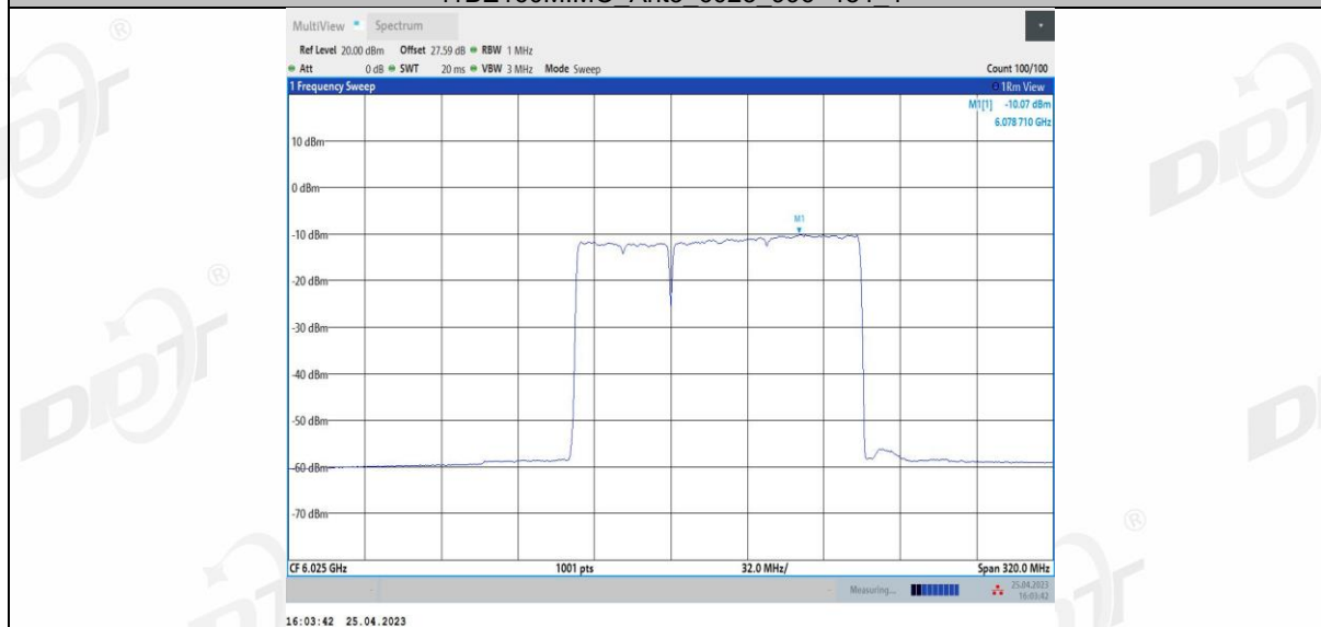
11BE160MIMO Ant3_6025_996+484_2
