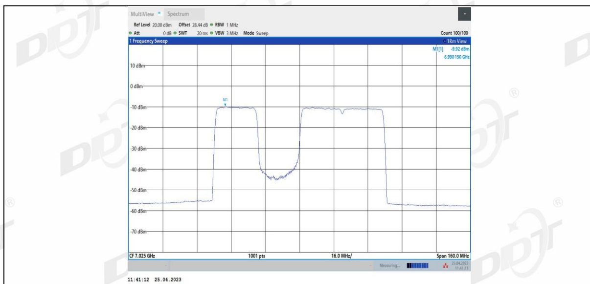
11BE80MIMO Ant4_7025_484+242_3
