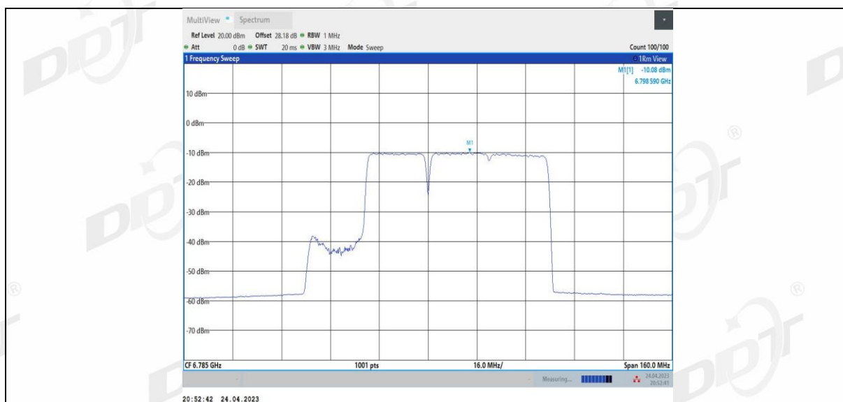
11BE80MIMO Ant2 6785 484+242 2
