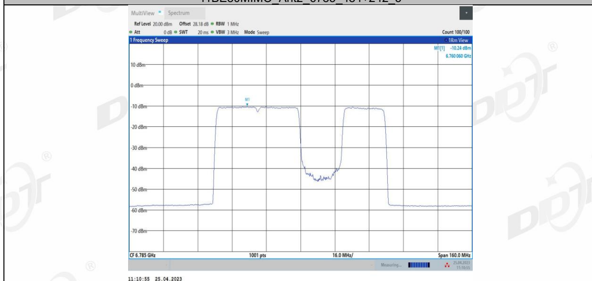
11BE80MIMO Ant2 6785 484+242 4
