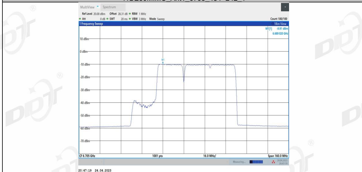
11BE80MIMO Ant1_6705_484+242_2
