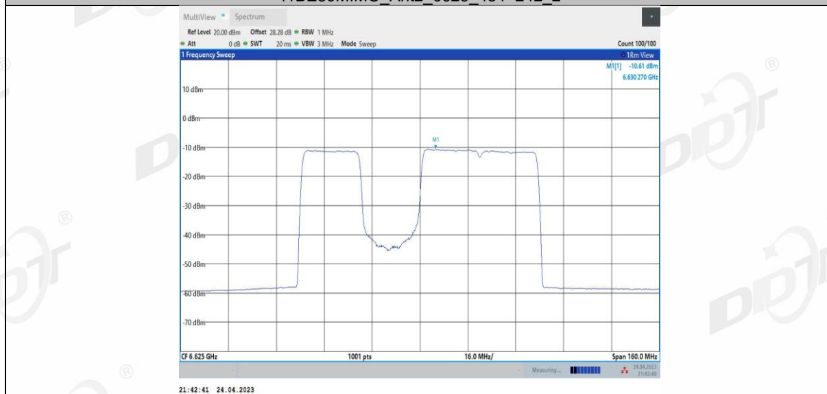
11BE80MIMO Ant2 6625 484+242 3
