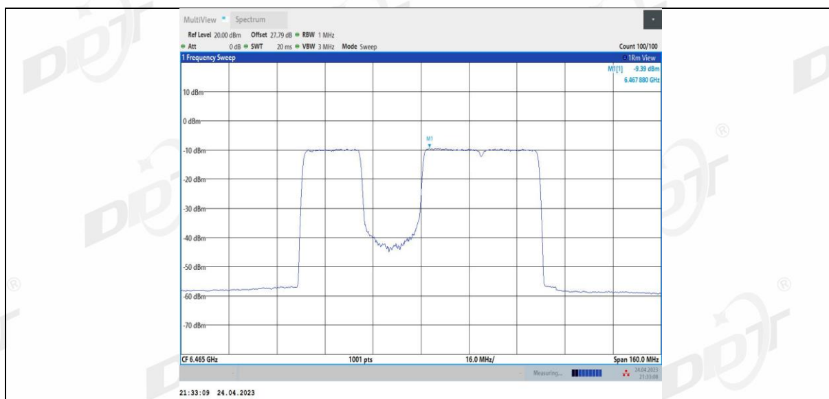
11BE80MIMO Ant2 6465 484+242_3
