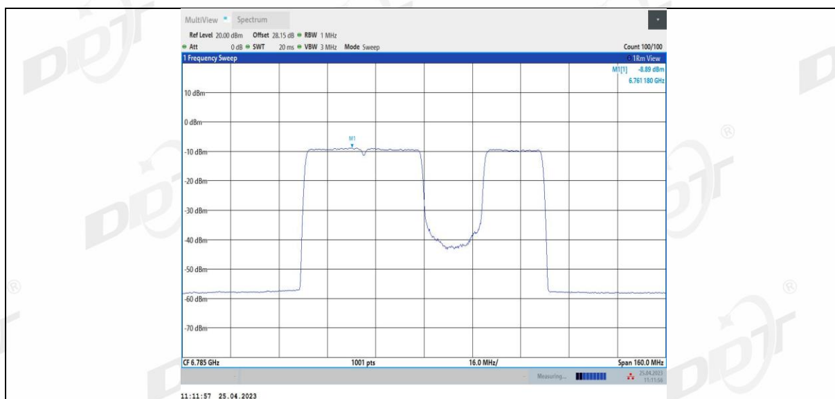
11BE80MIMO Ant3 6785 484+242 4
