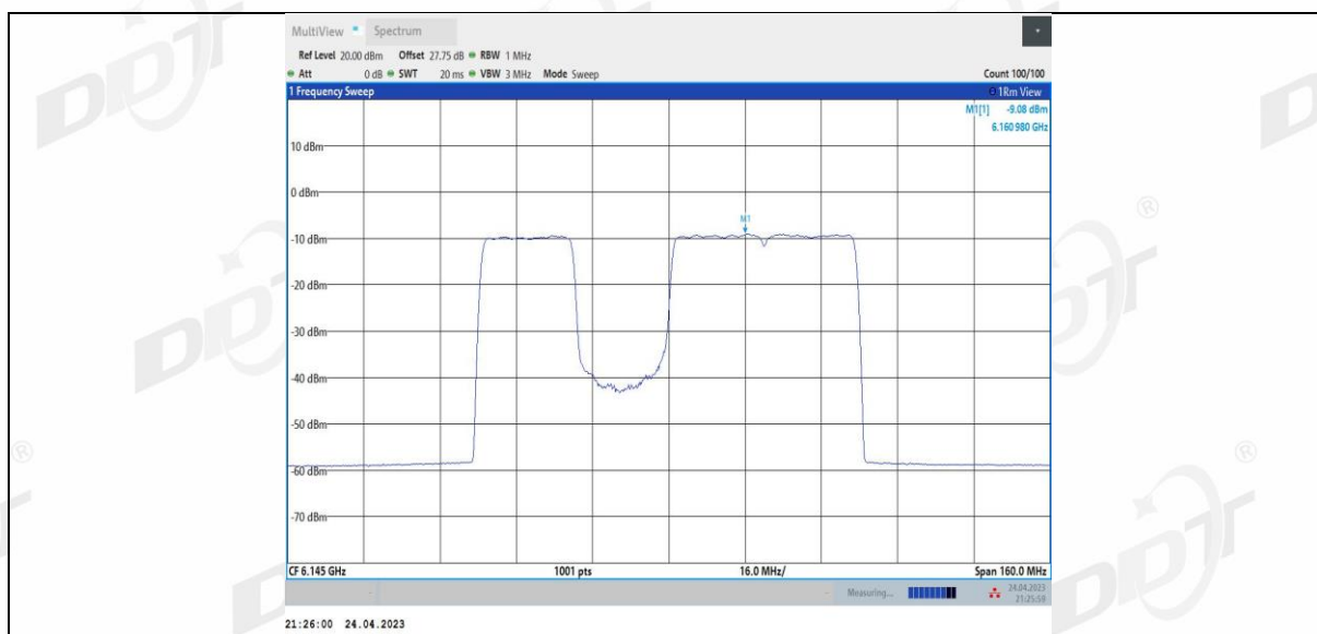
11BE80MIMO Ant4 6145 484+242_3
