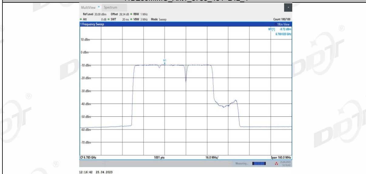
11BE80MIMO Ant2 6785 484+242_1
