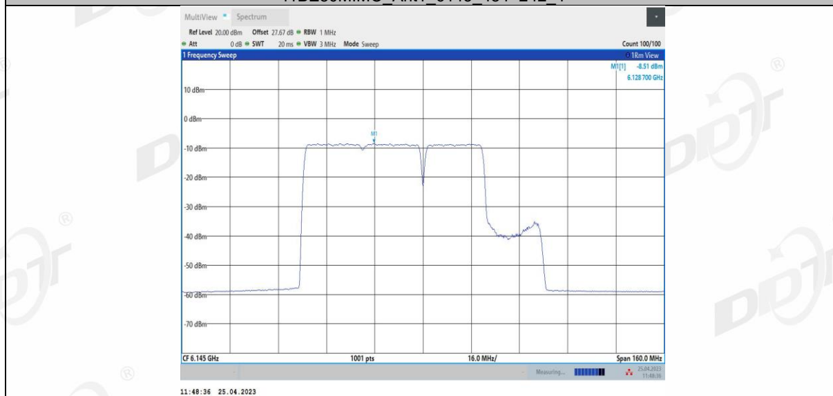
11BE80MIMO Ant2 6145 484+242_1
