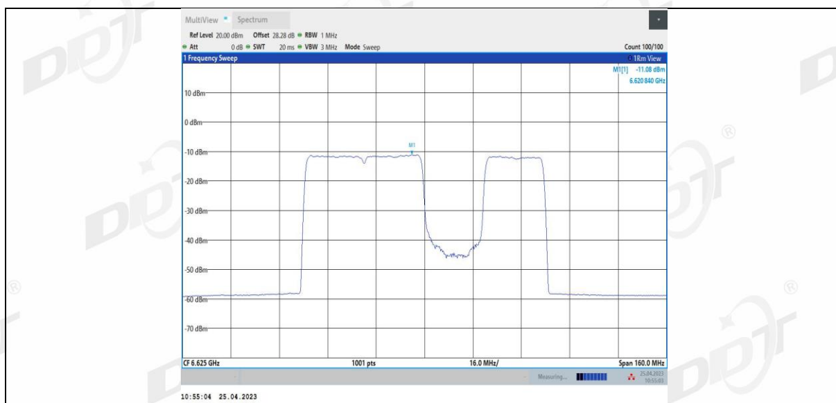
11BE80MIMO Ant2 6625 484+242 4
