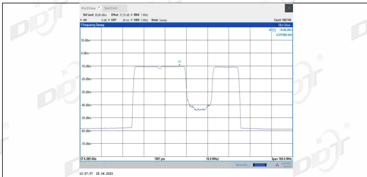
11BE80MIMO Ant2 6385 484+242 4
