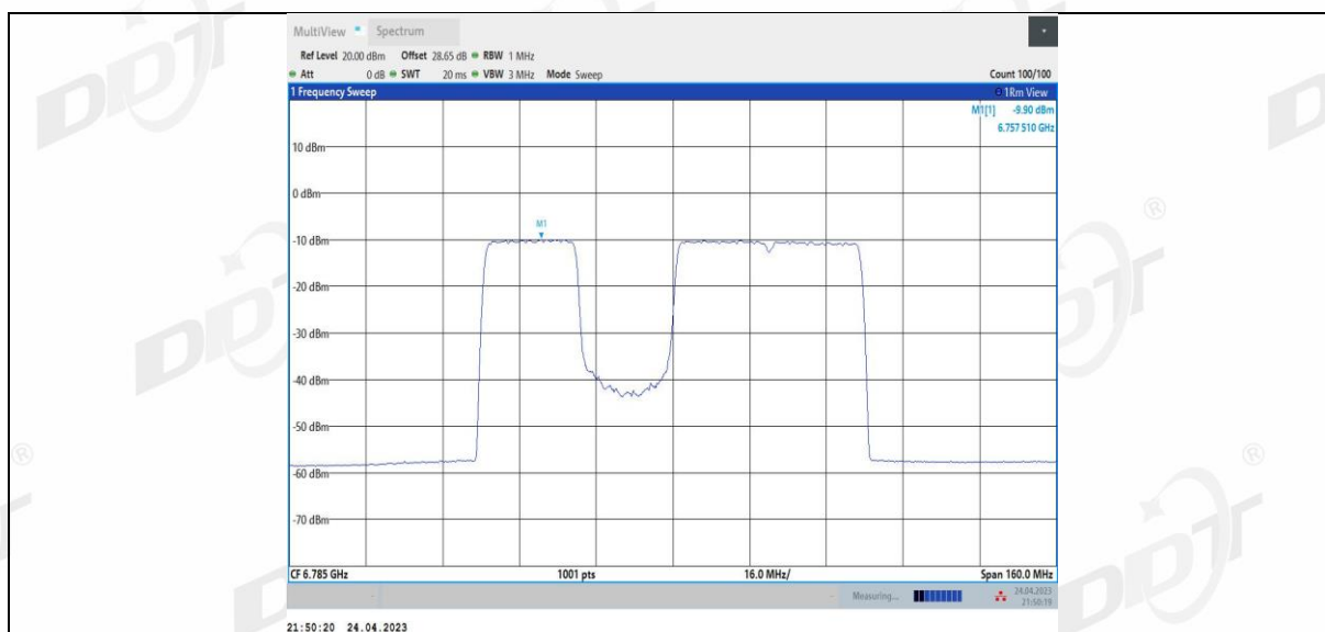
11BE80MIMO Ant1 6785 484+242_3
