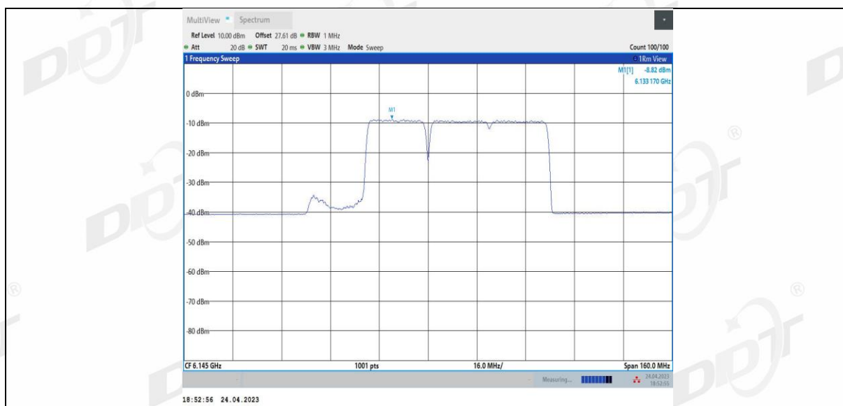
11BE80MIMO Ant2 6145 484+242 2
