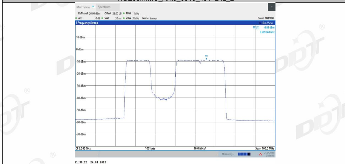
11BE80MIMO Ant3 6545 484+242 3
