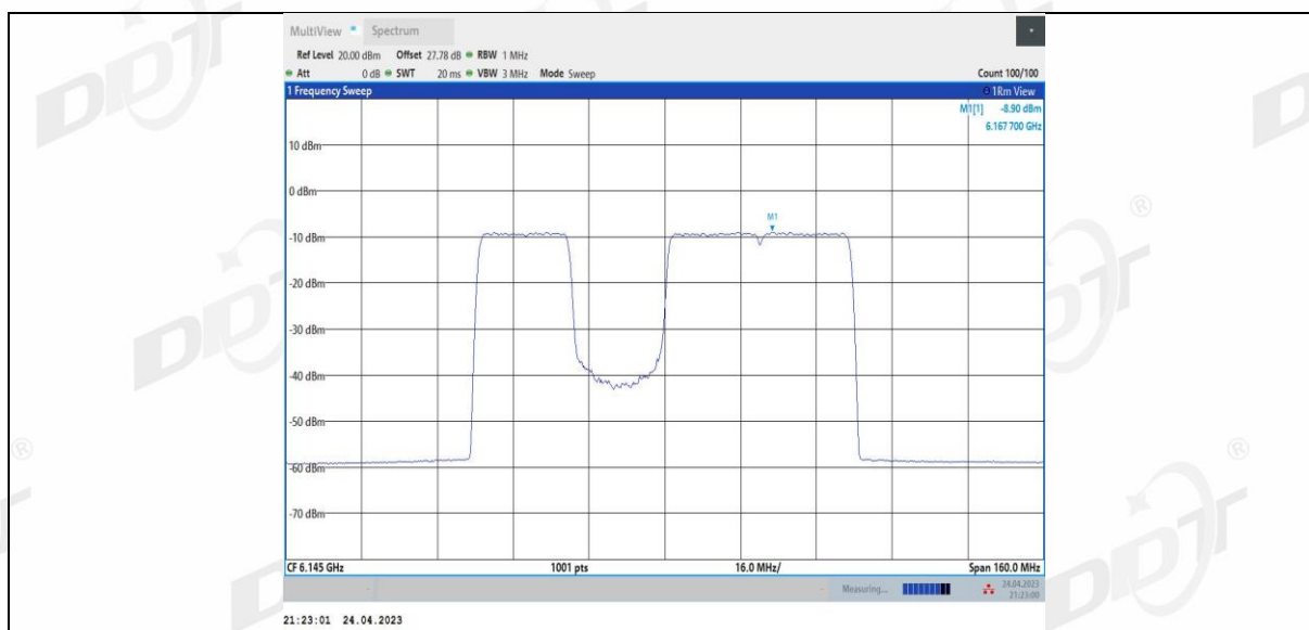
11BE80MIMO Ant1 6145 484+242_3
