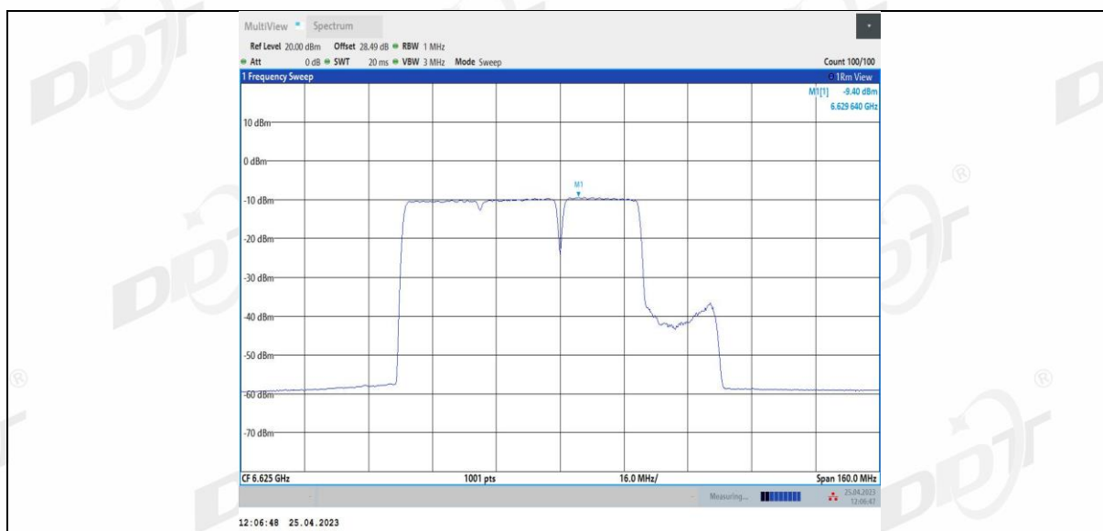
11BE80MIMO Ant2 6625 484+242 1
