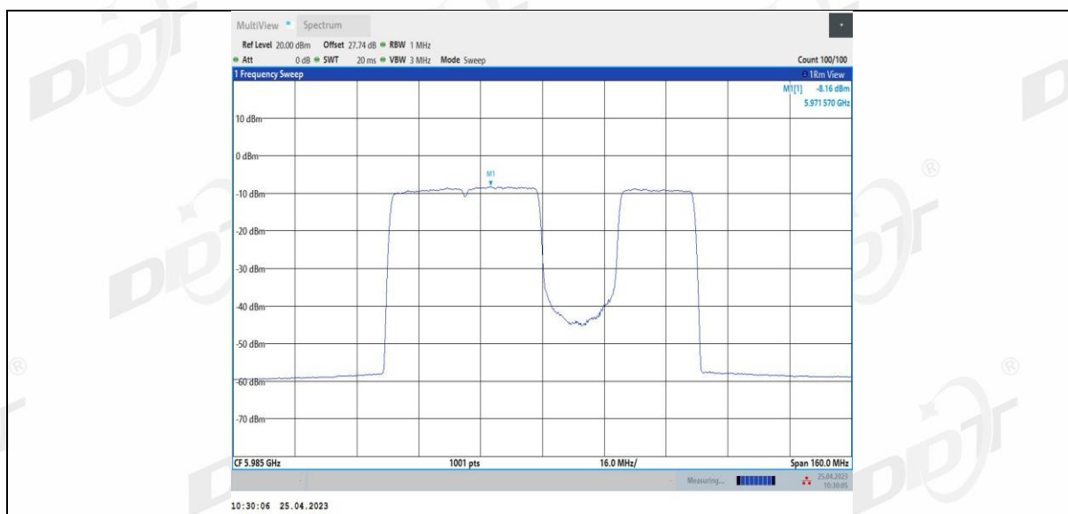
11BE80MIMO Ant4 5985 484+242 4
