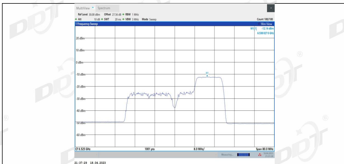
11BE40MIMO Ant3 6525 106+26 3
