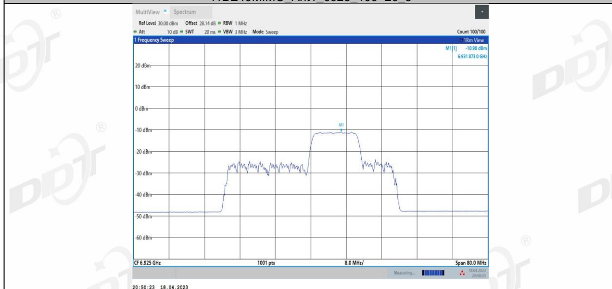
11BE40MIMO Ant1_6925_106+26_4
