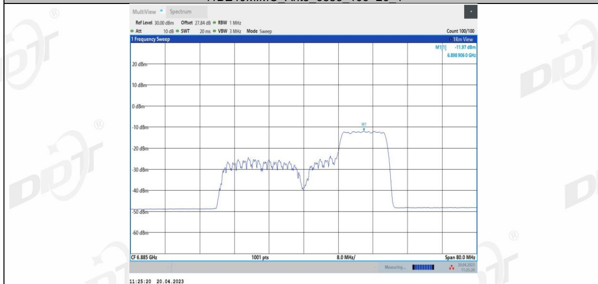
11BE40MIMO Ant4 6885 106+26 3
