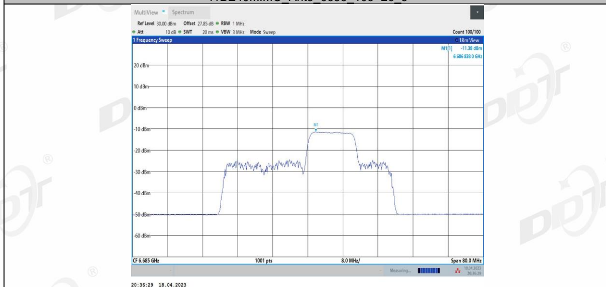
11BE40MIMO Ant3 6685 106+26 4
