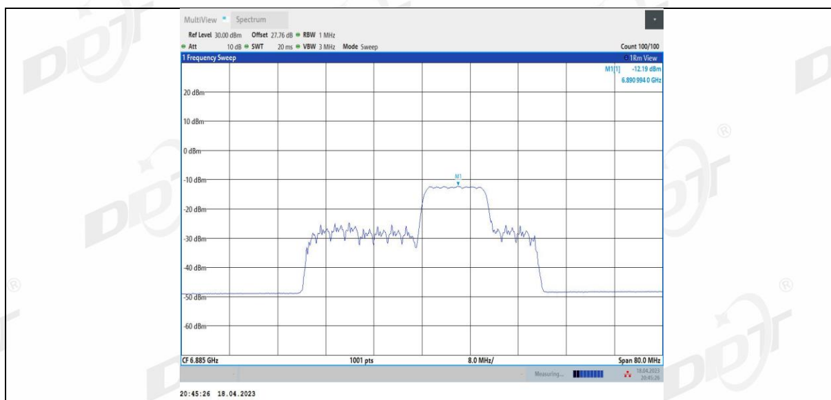
11BE40MIMO Ant3 6885 106+26 4
