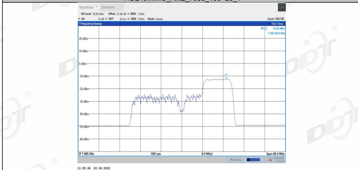
11BE40MIMO Ant3 7085 106+26 3
