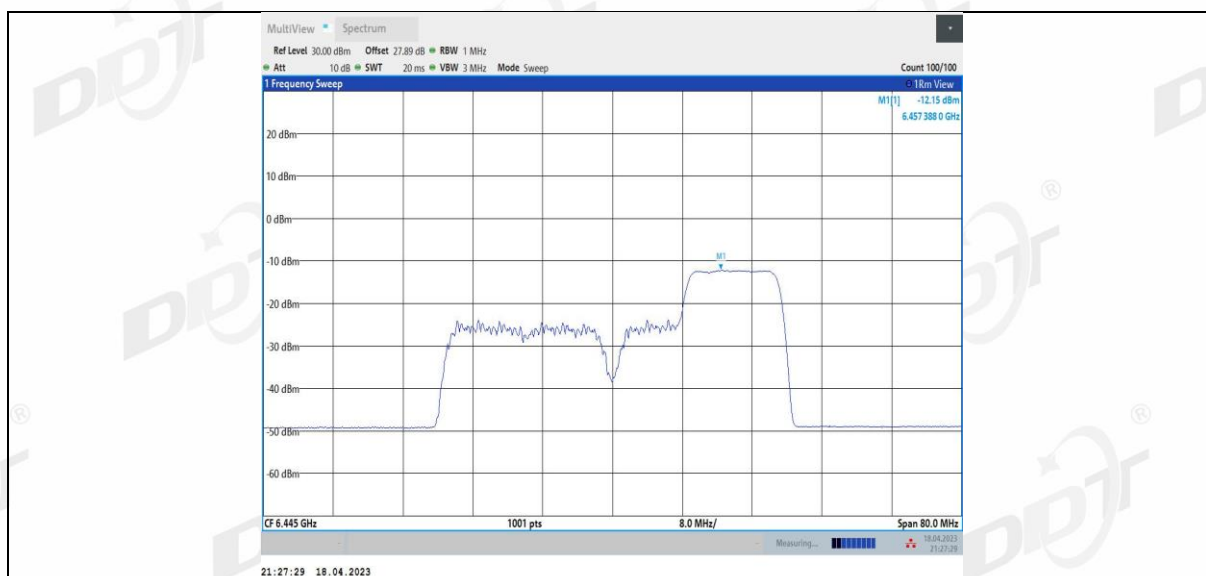
11BE40MIMO Ant2 6445 106+26 3
