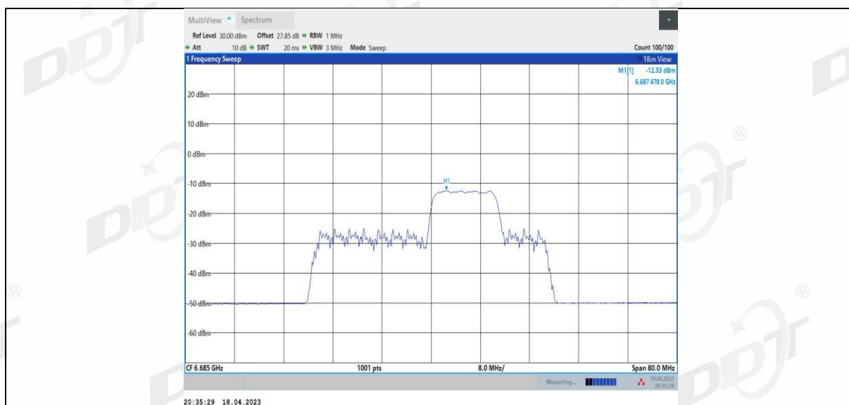
11BE40MIMO Ant2 6685 106+26 4
