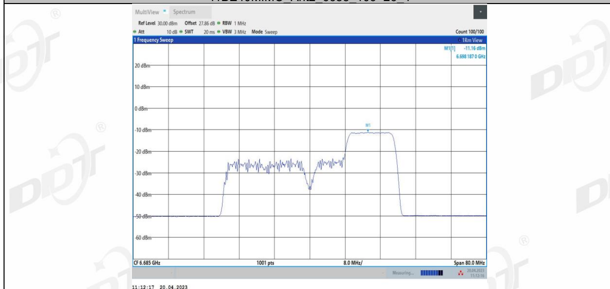
11BE40MIMO Ant3 6685 106+26 3
