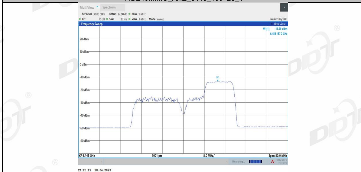
11BE40MIMO Ant3 6445 106+26 3
