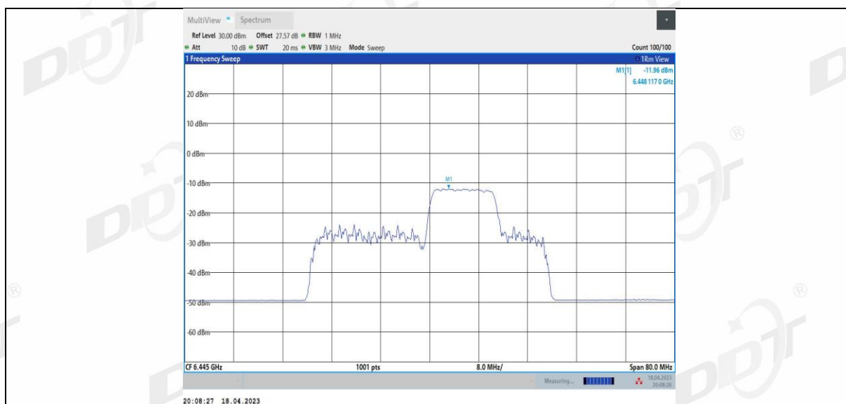
11BE40MIMO Ant3 6445 106+26 4
