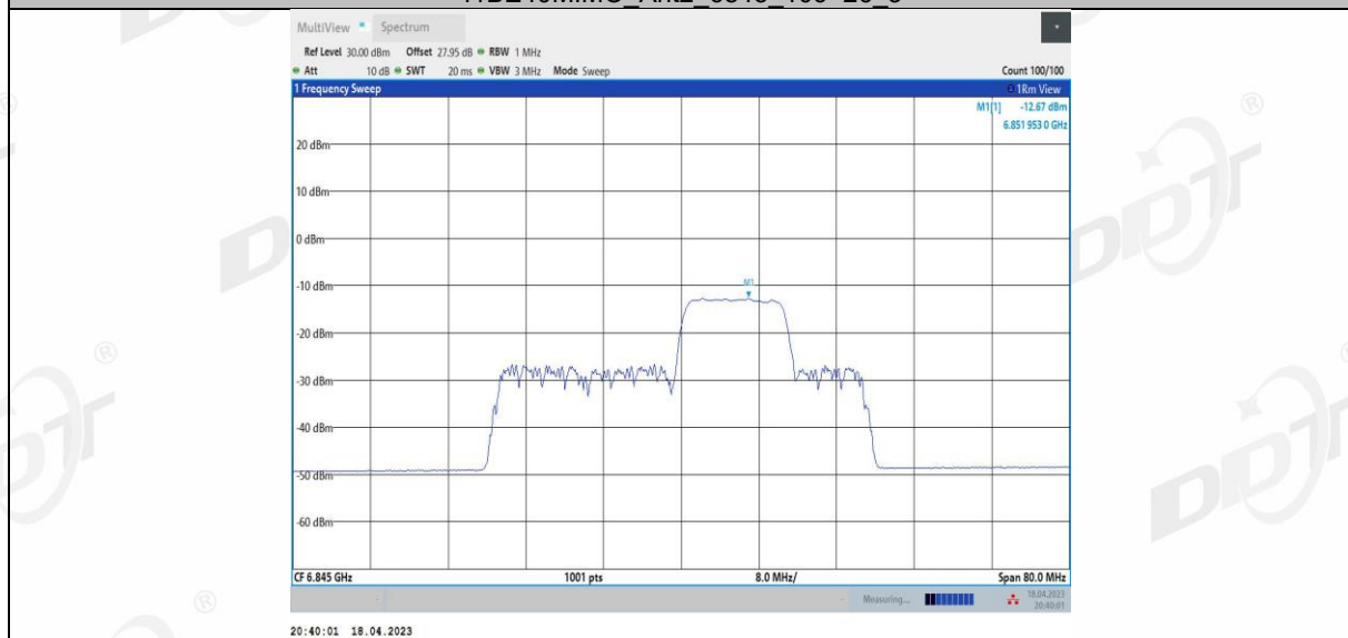
11BE40MIMO Ant2 6845 106+26 4
