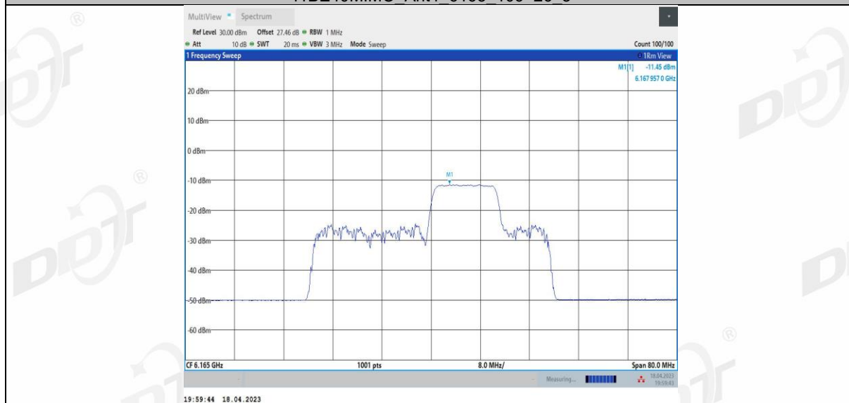
11BE40MIMO Ant4 6165 106+26 4
