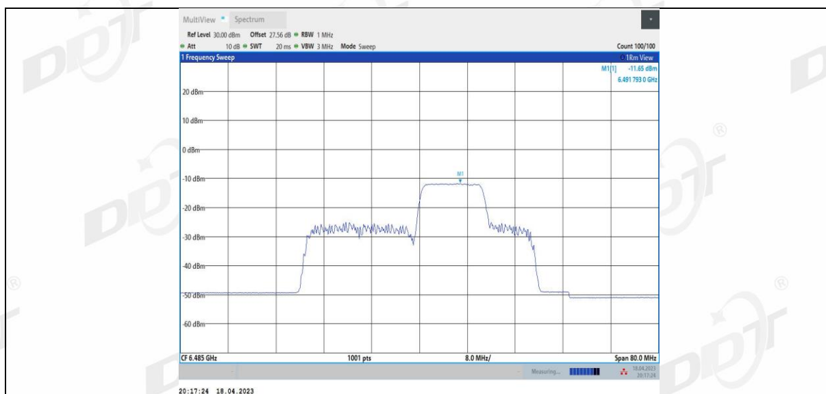
11BE40MIMO Ant2 6485 106+26 4
