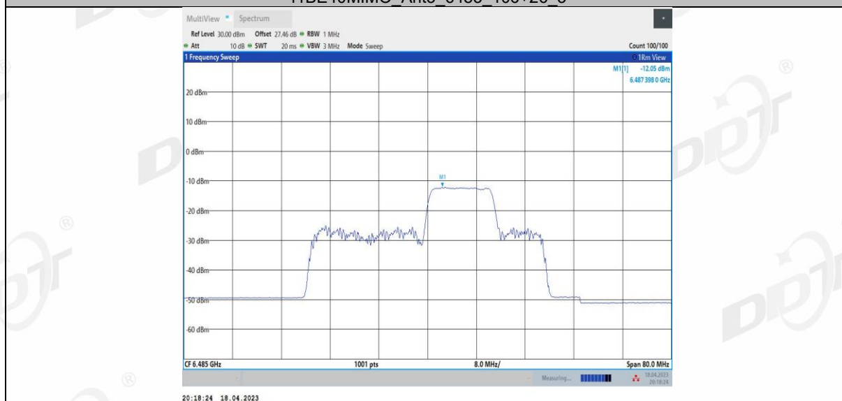
11BE40MIMO Ant3 6485 106+26 4
