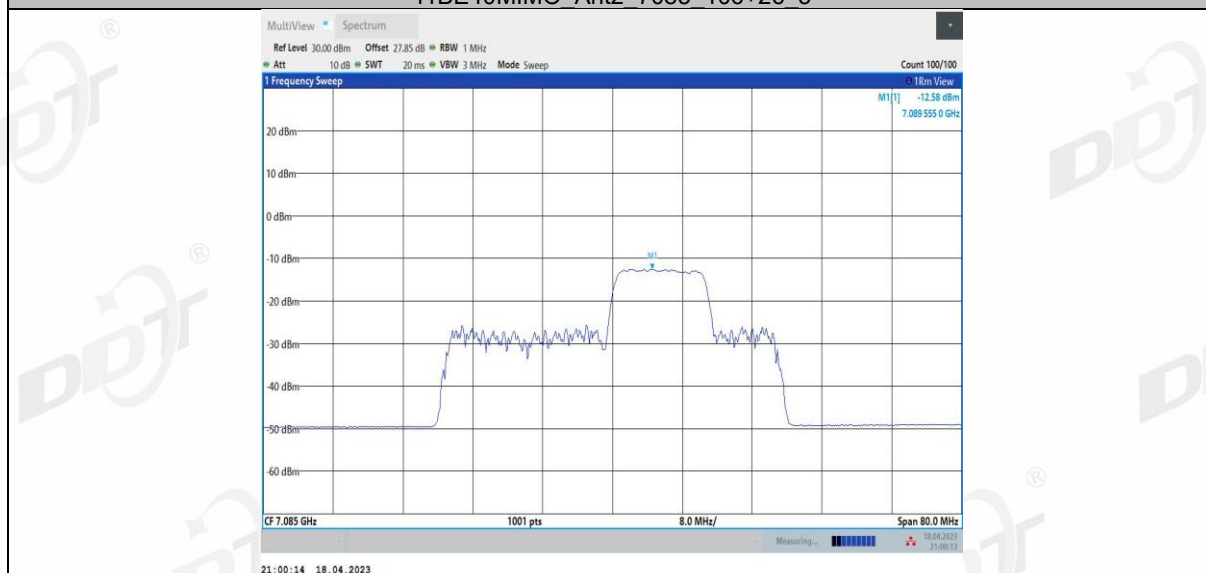
11BE40MIMO Ant2 7085 106+26 4
