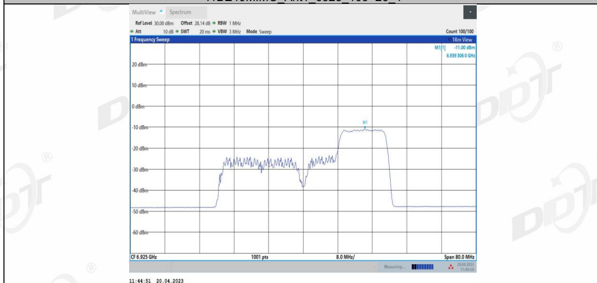
11BE40MIMO Ant2_6925_106+26_3
