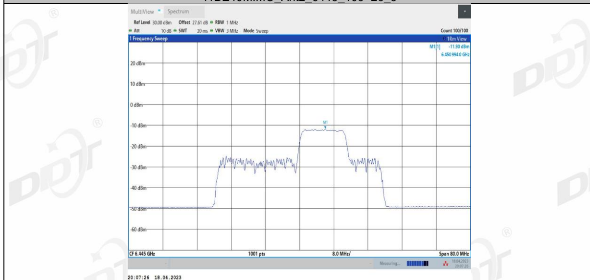
11BE40MIMO Ant2 6445 106+26 4
