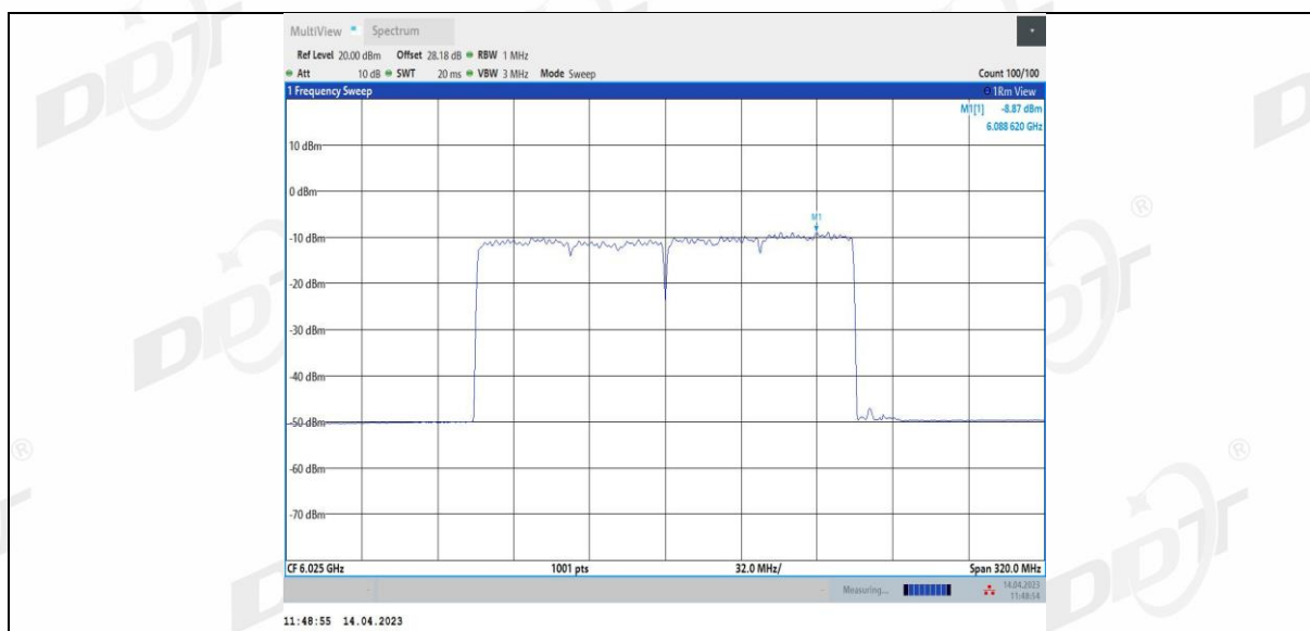
11AX160MIMO Ant3 6025
