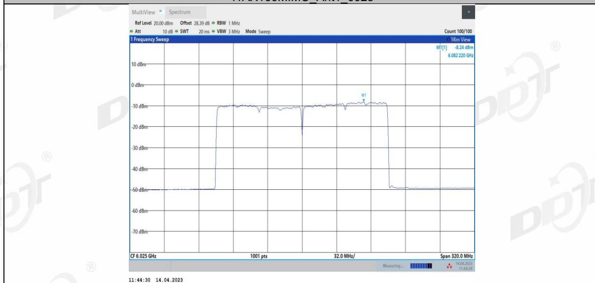
11AX160MIMO Ant2_6025
