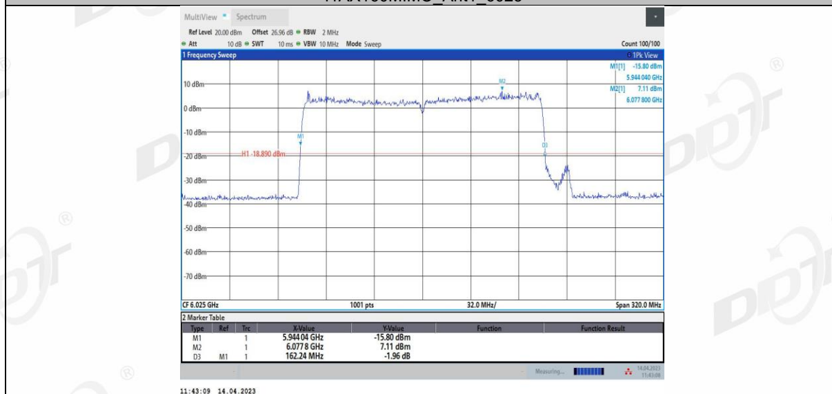
11AX160MIMO Ant2 6025
