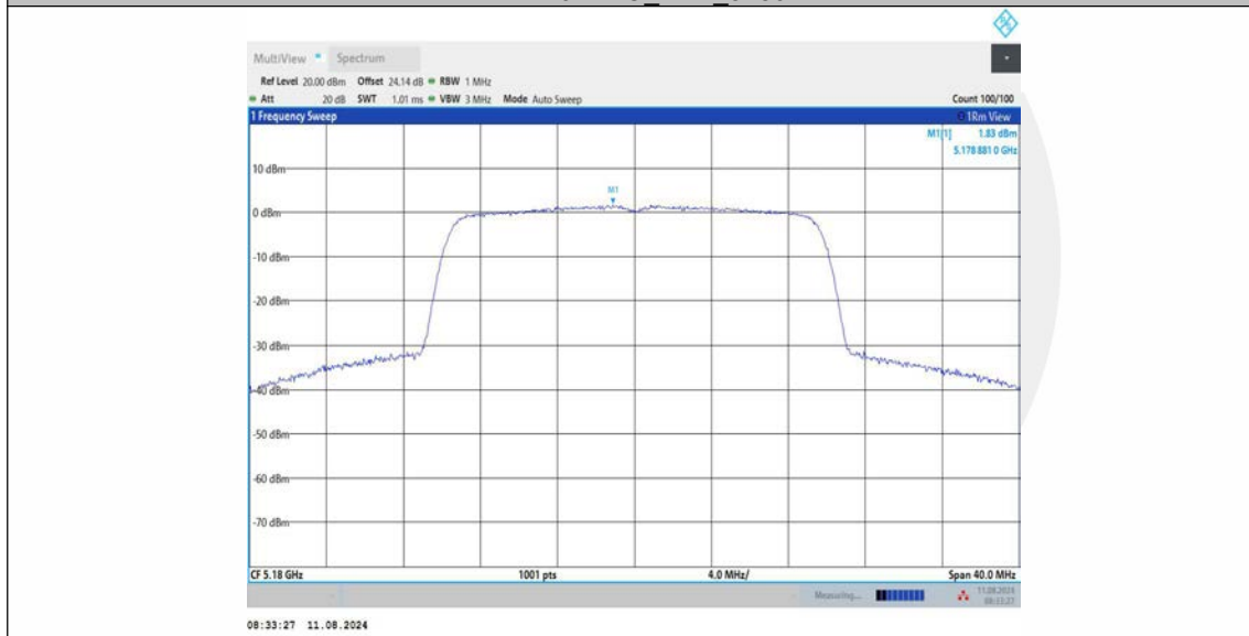
11AX20MIMO Ant3_5180
