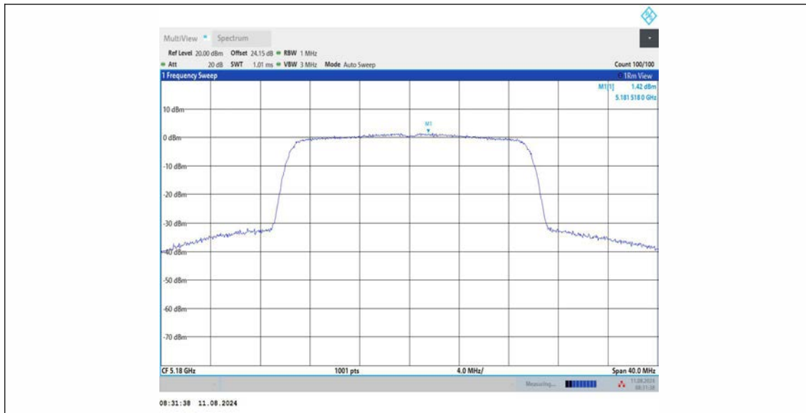
11AX20MIMO Ant2_5180
