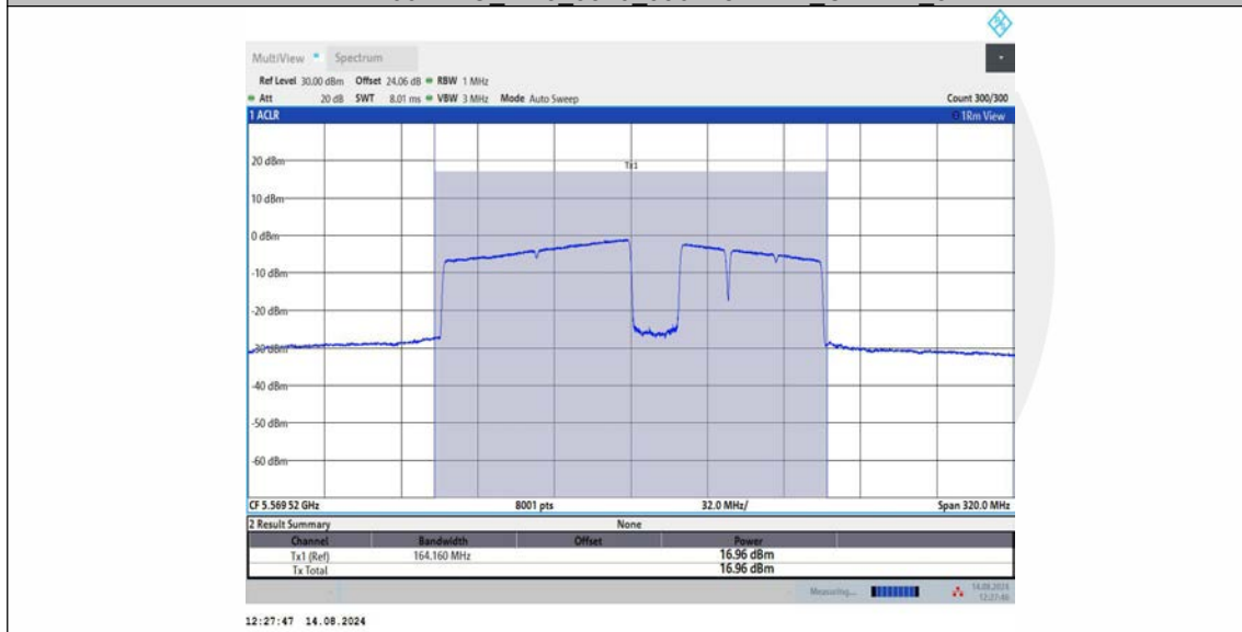
11BE160MIMO_Ant3_5570_996+484+242_OFDMA_6
