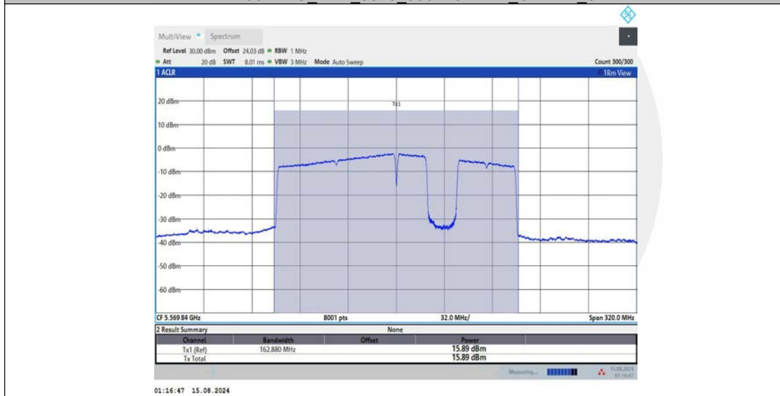
11BE160MIMO_Ant1_5570_996+484+242_OFDMA_7
