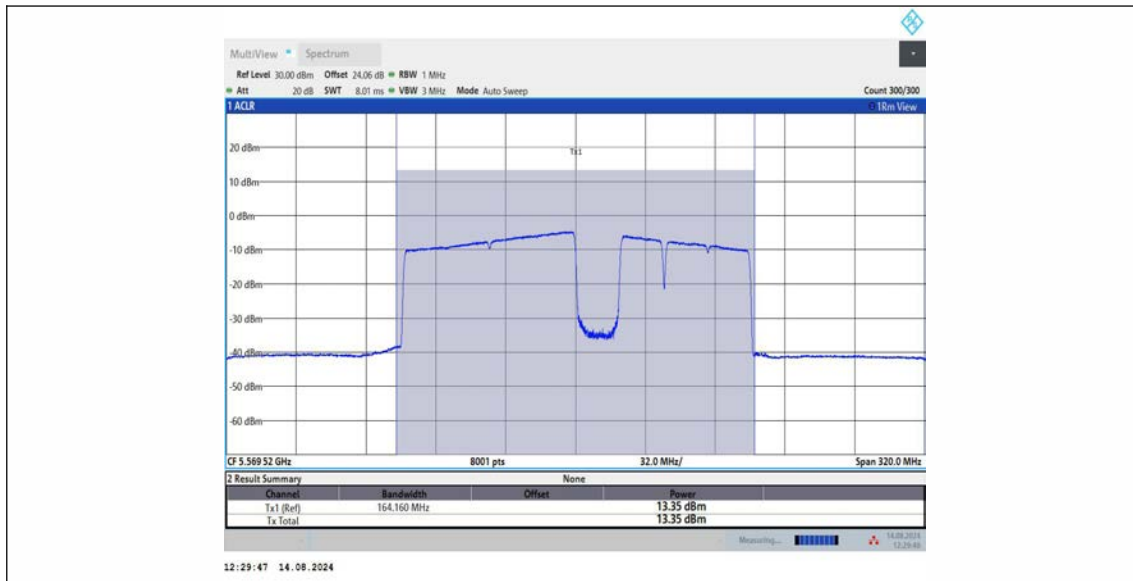
11BE160MIMO_Ant3_5570_996+484+242_OFDMA_5
