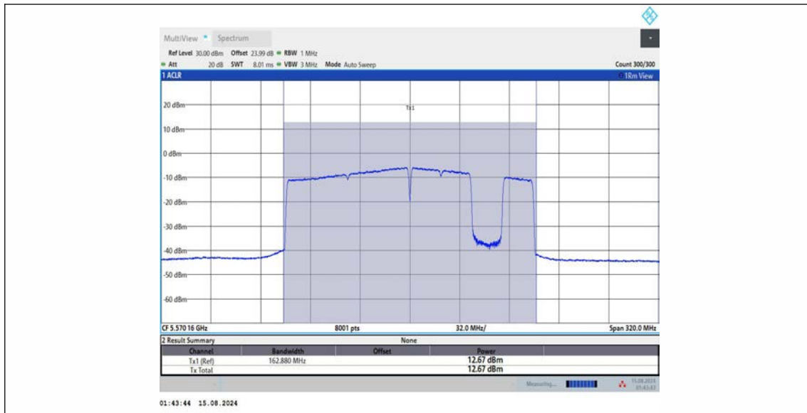
11BE160MIMO_Ant1_5570_996+484+242_OFDMA_7
