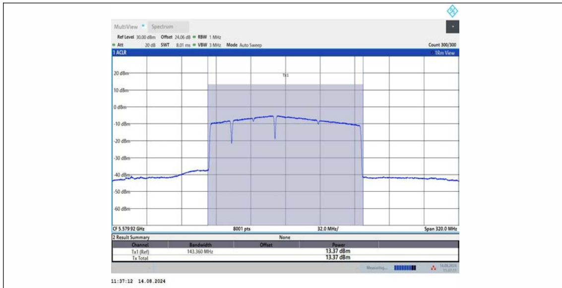
11BE160MIMO_Ant3_5570_996+484+242_OFDMA_1
