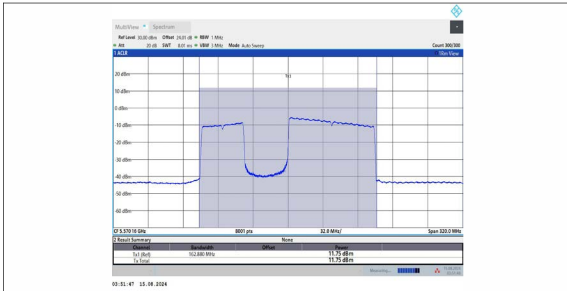
11BE160MIMO Ant2 5570 996+484 OFDMA 2
