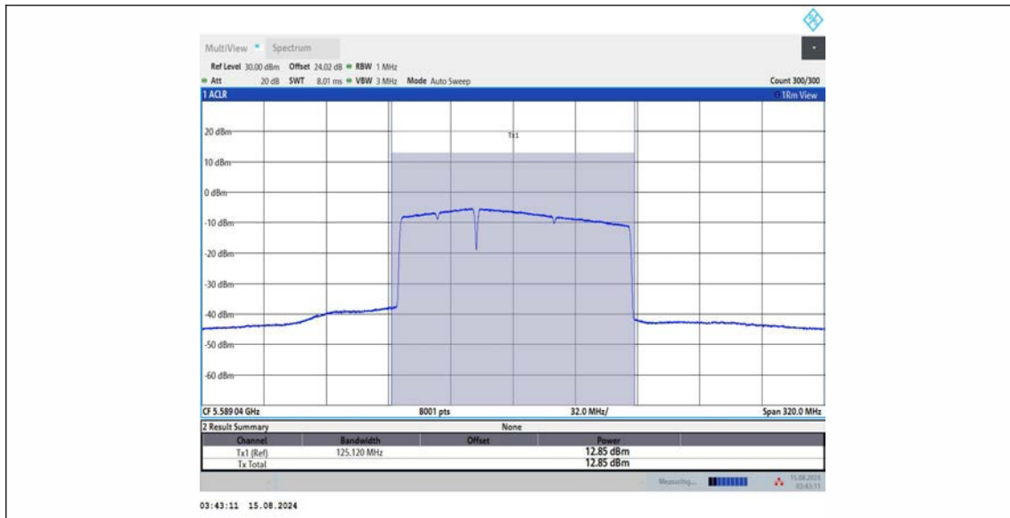
11BE160MIMO Ant3 5570 996+484 OFDMA 1
