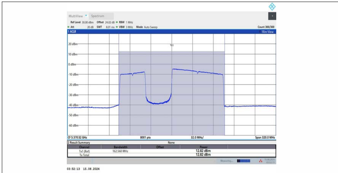
11BE160MIMO Ant3 5570 996+484 OFDMA 2
