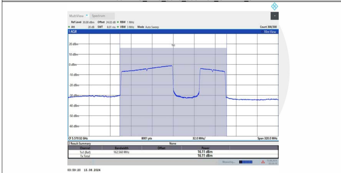
11BE160MIMO Ant3 5570 996+484 OFDMA 4
