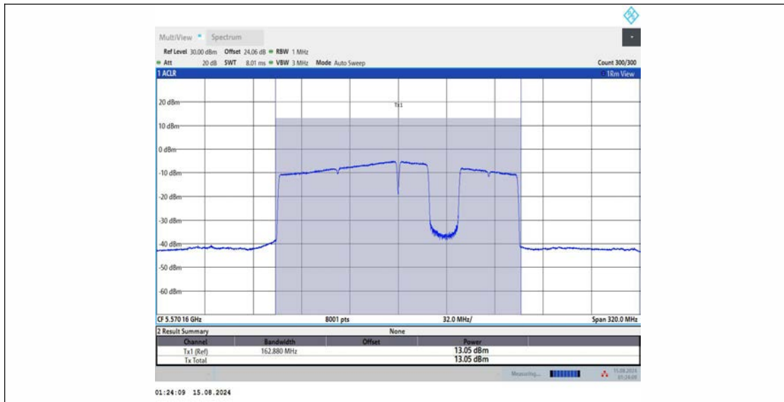
11BE160MIMO_Ant3_5570_996+484+242_OFDMA_6
