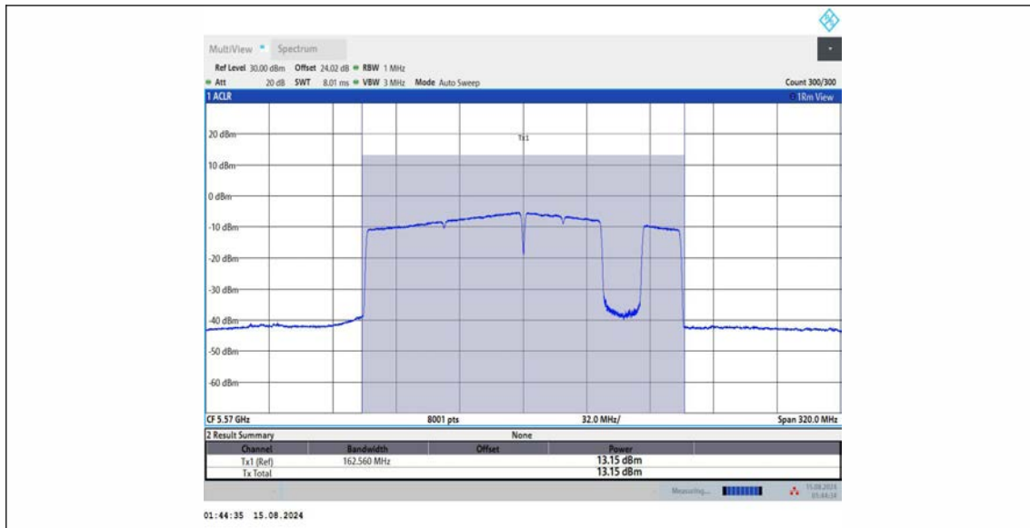
11BE160MIMO_Ant3_5570_996+484+242_OFDMA_7
