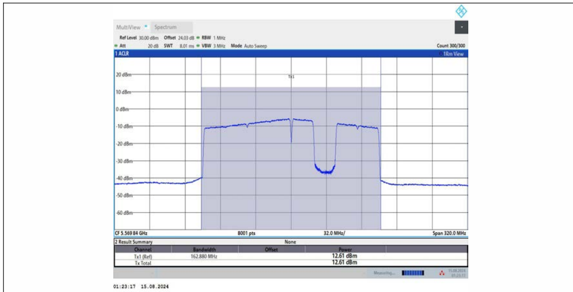
11BE160MIMO_Ant1_5570_996+484+242_OFDMA_6
