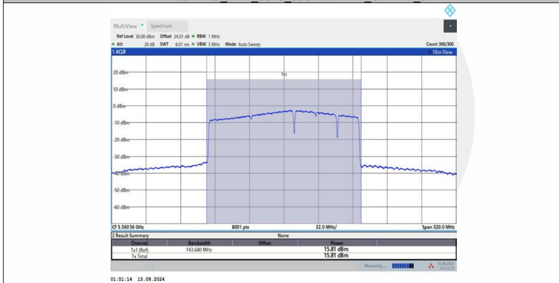
11BE160MIMO_Ant3_5570_996+484_OFDMA_1
