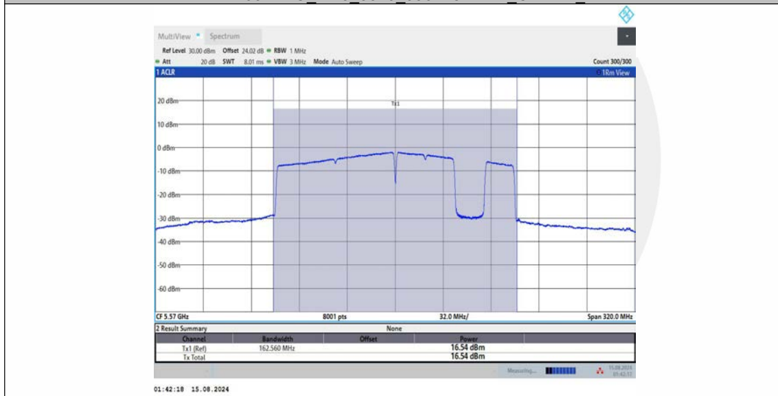
11BE160MIMO_Ant3_5570_996+484+242_OFDMA_8
