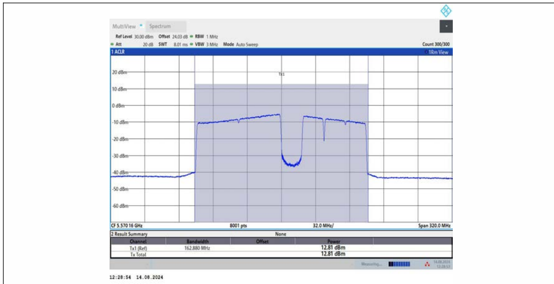
11BE160MIMO_Ant1_5570_996+484+242_OFDMA_5
