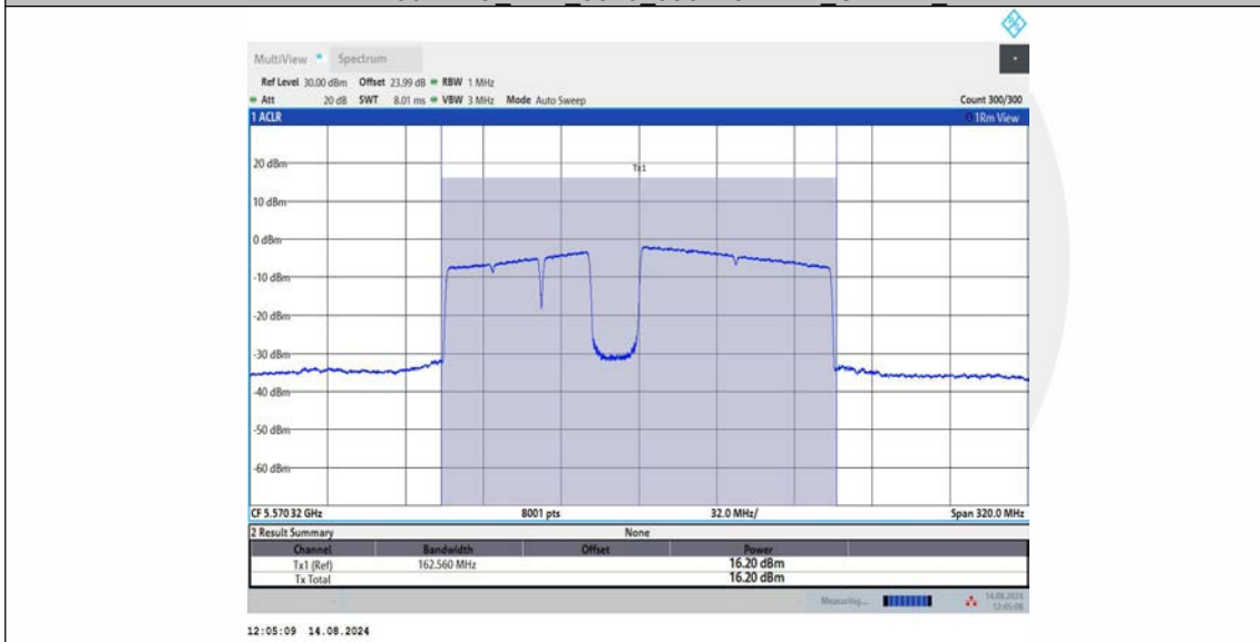
11BE160MIMO_Ant1_5570_996+484+242_OFDMA_5
