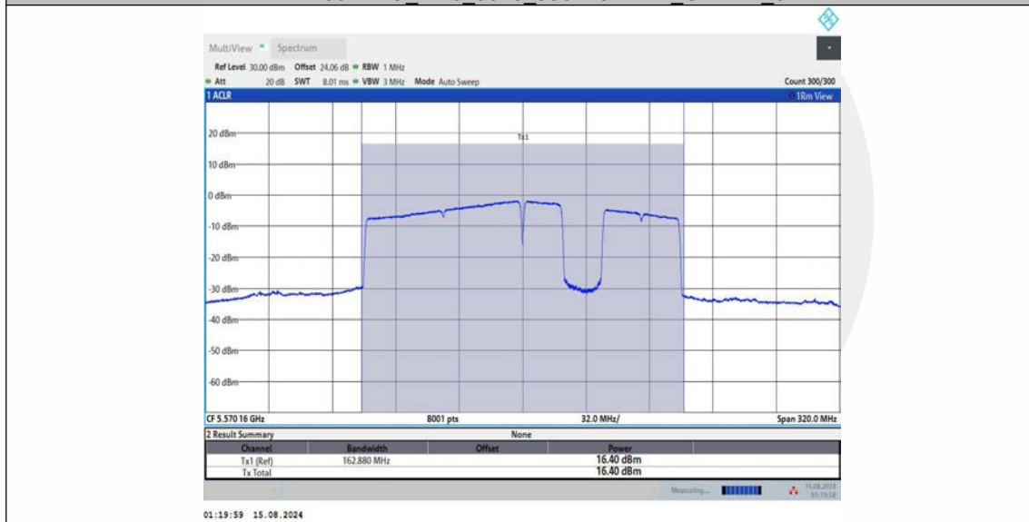
11BE160MIMO_Ant3_5570_996+484+242_OFDMA_7
