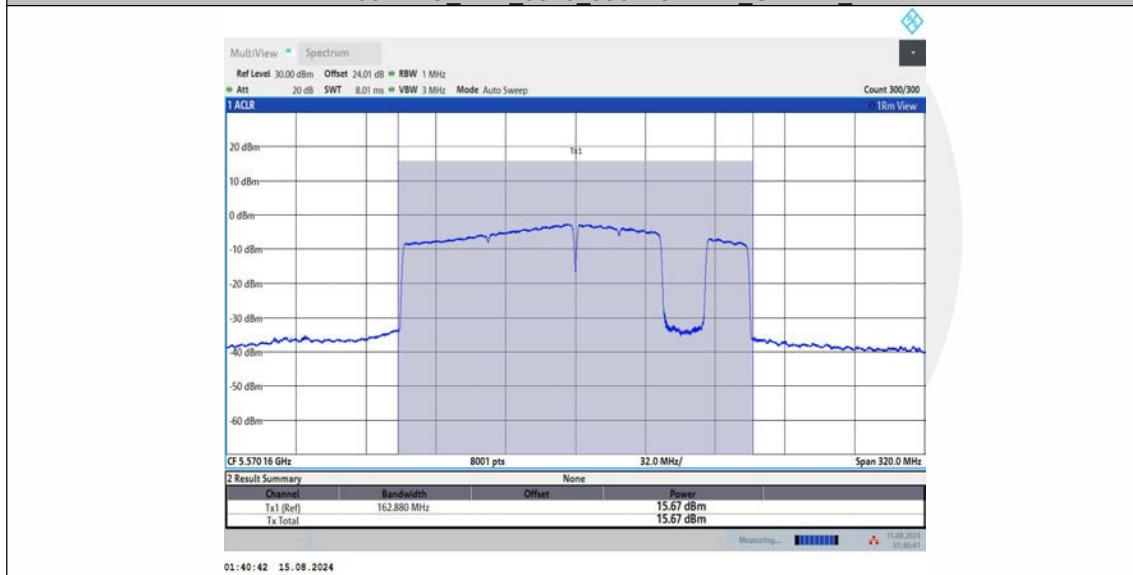
11BE160MIMO_Ant2_5570_996+484+242_OFDMA_8
