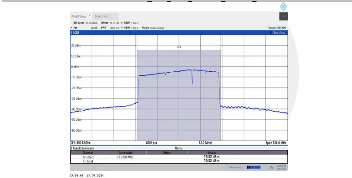
11BE160MIMO Ant2 5570 996+484+242 OFDMA 1
