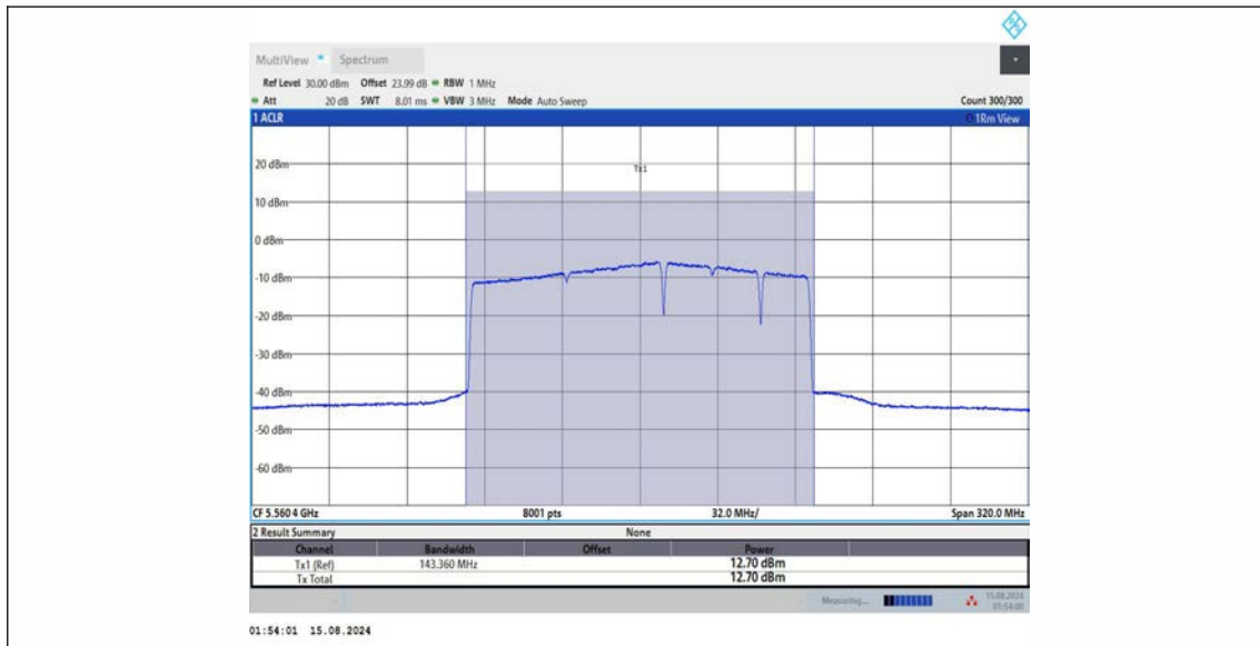
11BE160MIMO_Ant1_5570_996+484+242_OFDMA_8
