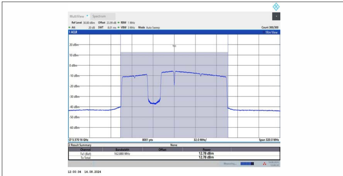
11BE160MIMO_Ant1_5570_996+484+242_OFDMA_3
