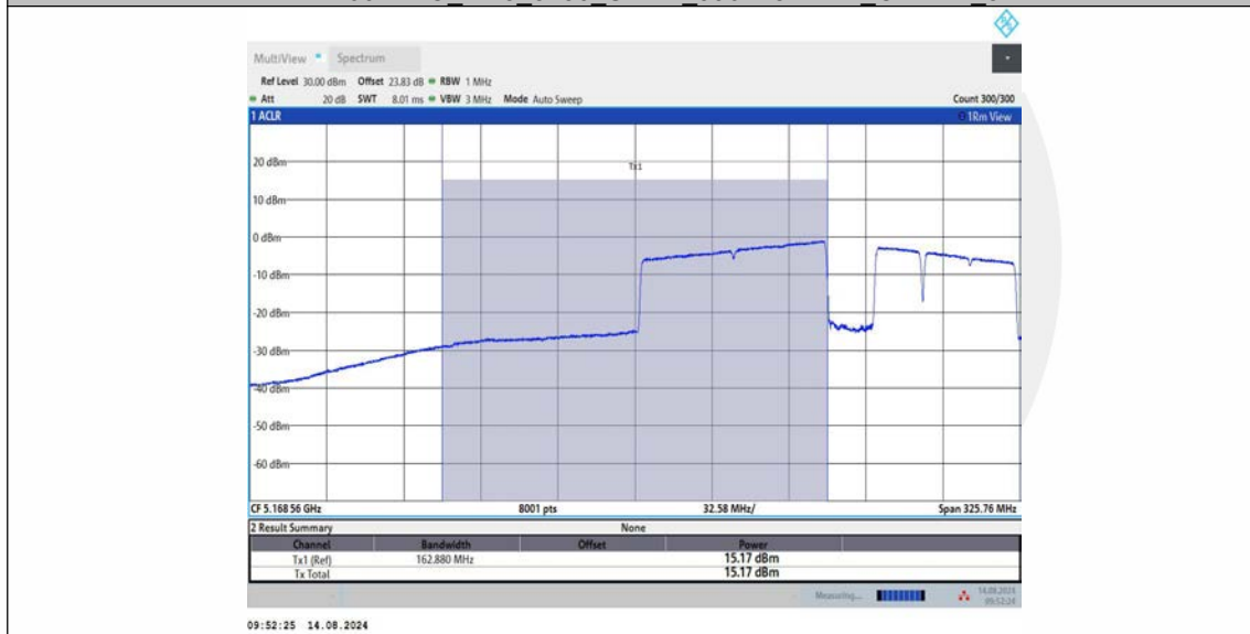
11BE160MIMO_Ant3_5250_UNII-1_996+484+242_OFDMA_6
