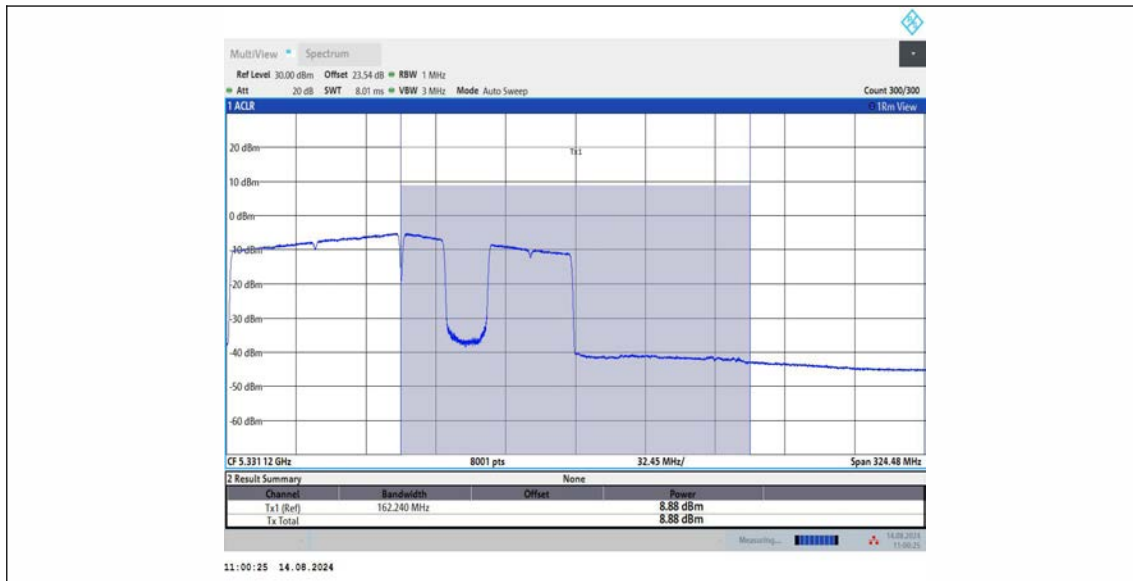
11BE160MIMO_Ant3_5250_UNII-2A_996+484+242_OFDMA_6
