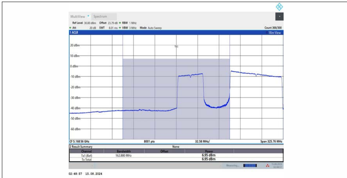
11BE160MIMO_Ant3_5250_UNII-1_996+484_OFDMA_2
