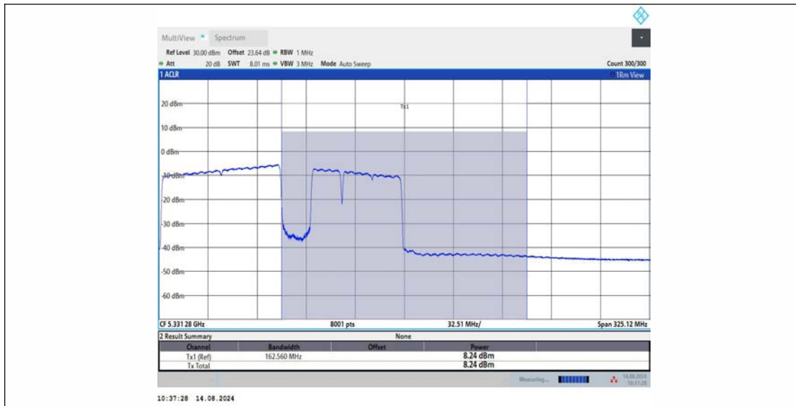
11BE160MIMO_Ant2_5250_UNII-2A_996+484+242_OFDMA_5
