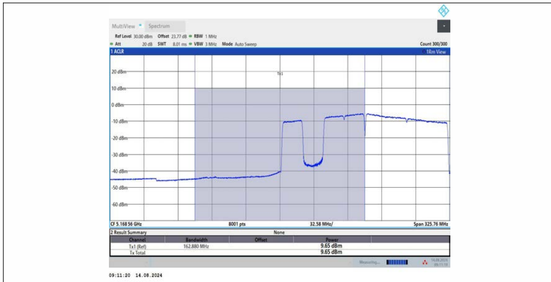
11BE160MIMO_Ant1_5250_UNII-1_996+484+242_OFDMA_2
