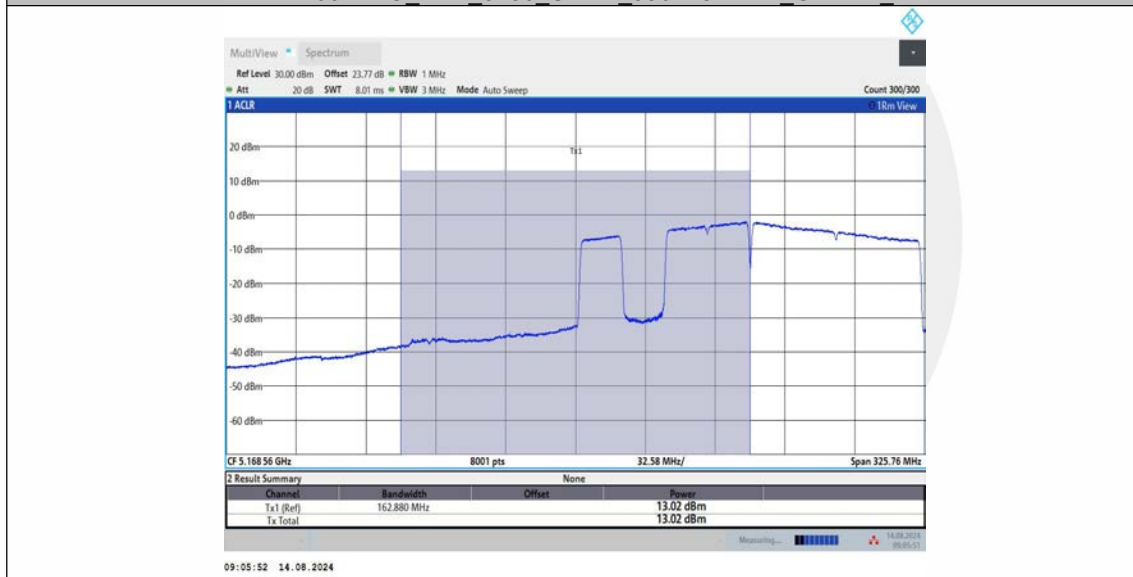
11BE160MIMO_Ant1_5250_UNII-1_996+484+242_OFDMA_3
