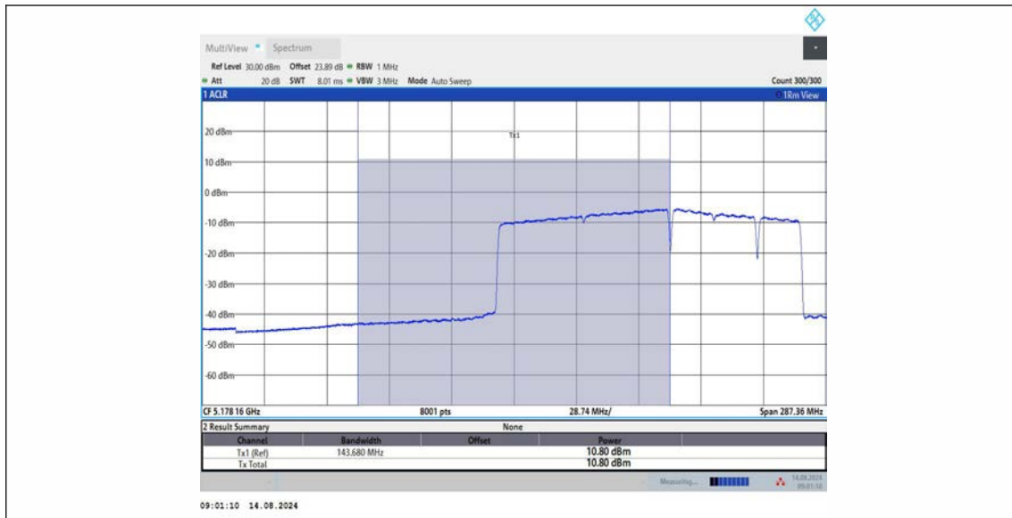
11BE160MIMO_Ant2_5250_UNII-1_996+484+242_OFDMA_8
