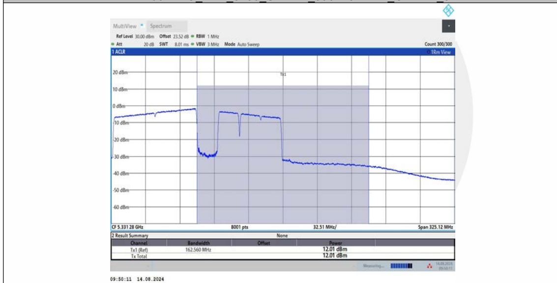
11BE160MIMO Ant1 5250 UNII-2A 996+484+242 OFDMA 6
