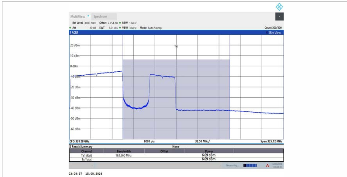
11BE160MIMO Ant3 5250 UNII-2A 996+484 OFDMA 3
