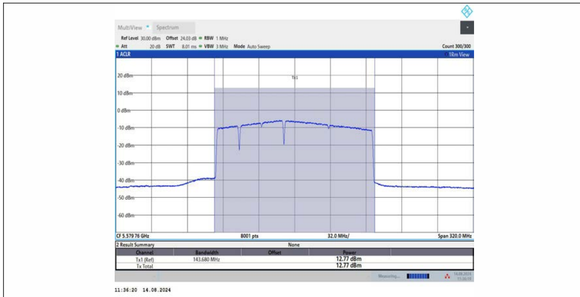
11BE160MIMO_Ant1_5570_996+484+242_OFDMA_1
