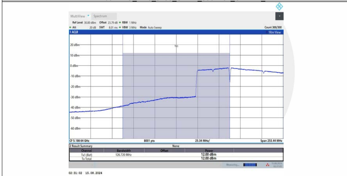
11BE160MIMO_Ant3_5250_UNII-1_996+484_OFDMA_2
