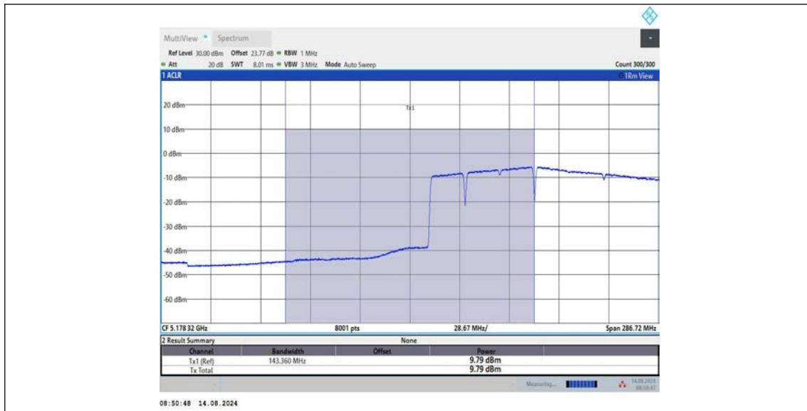
11BE160MIMO_Ant1_5250_UNII-1_996+484+242_OFDMA_1
