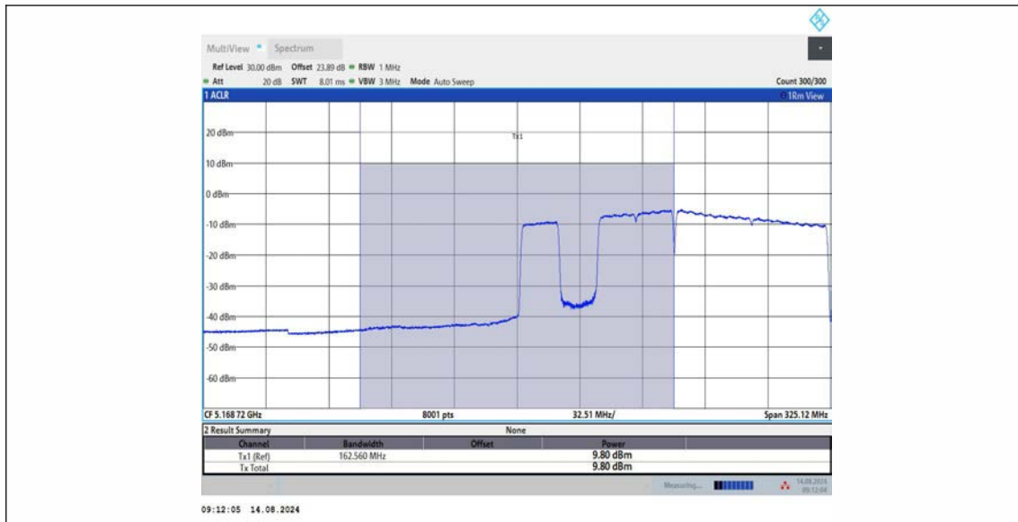
11BE160MIMO_Ant2_5250_UNII-1_996+484+242_OFDMA_2
