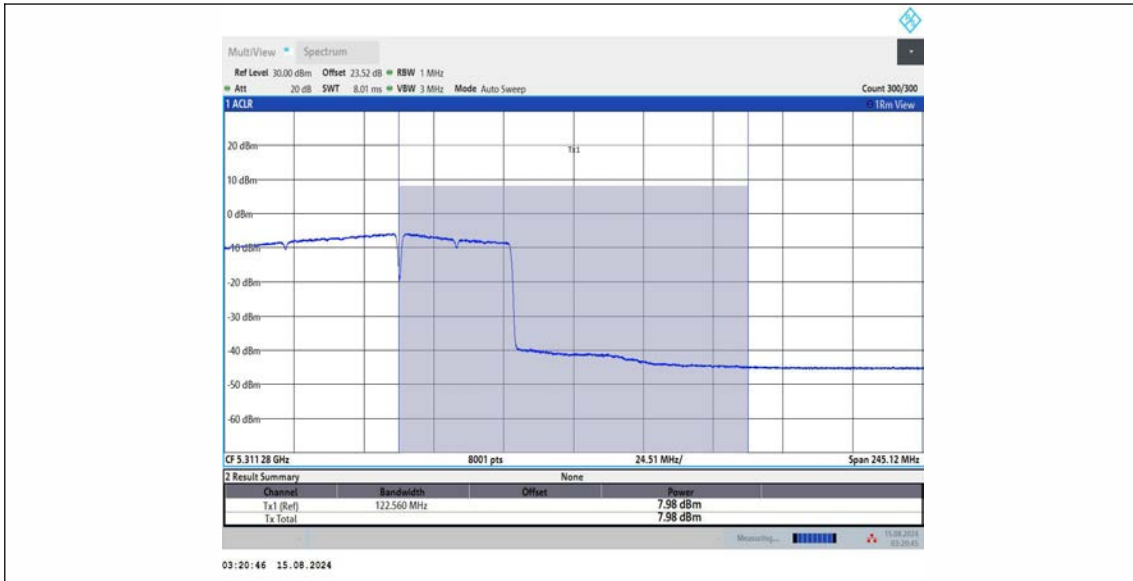
11BE160MIMO Ant1_5250_UNII-2A_996+484_OFDMA_4
