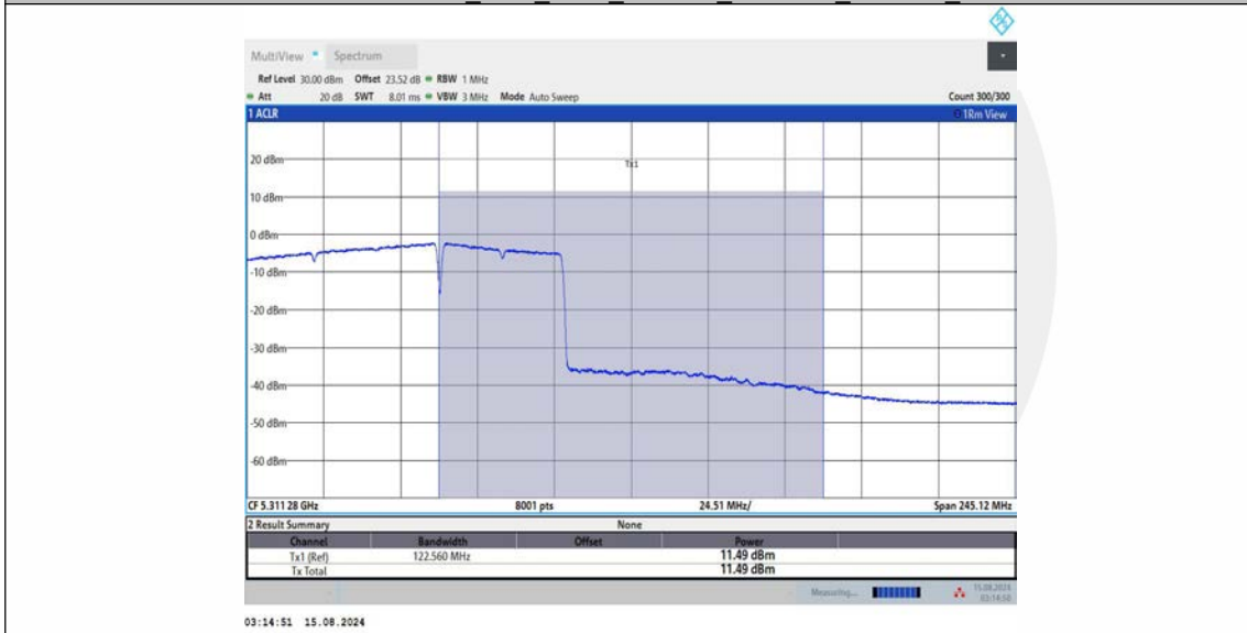
11BE160MIMO Ant1_5250_UNII-2A_996+484+242_OFDMA_1
