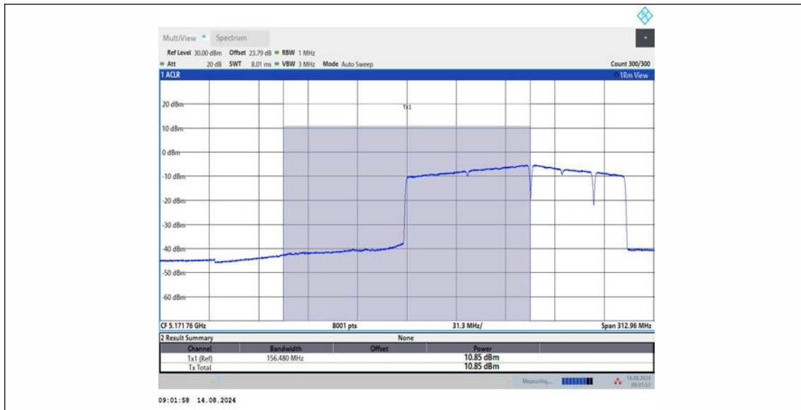
11BE160MIMO_Ant3_5250_UNII-1_996+484+242_OFDMA_8
