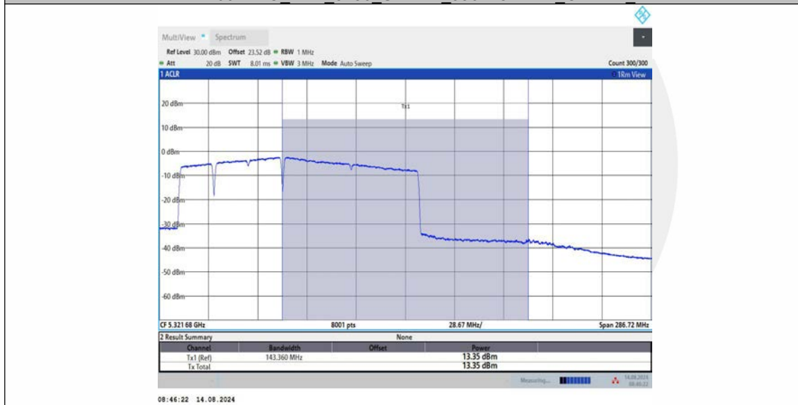
11BE160MIMO Ant1 5250 UNII-2A 996+484+242 OFDMA 2
