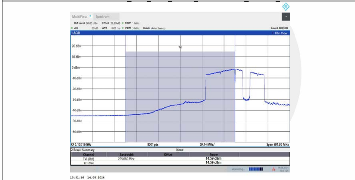
11BE160MIMO_Ant2_5250_UNII-1_996+484+242_OFDMA_7
