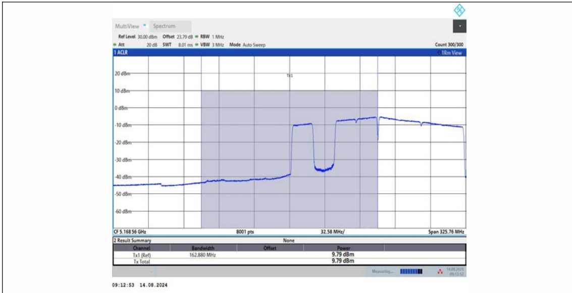
11BE160MIMO_Ant3_5250_UNII-1_996+484+242_OFDMA_2
