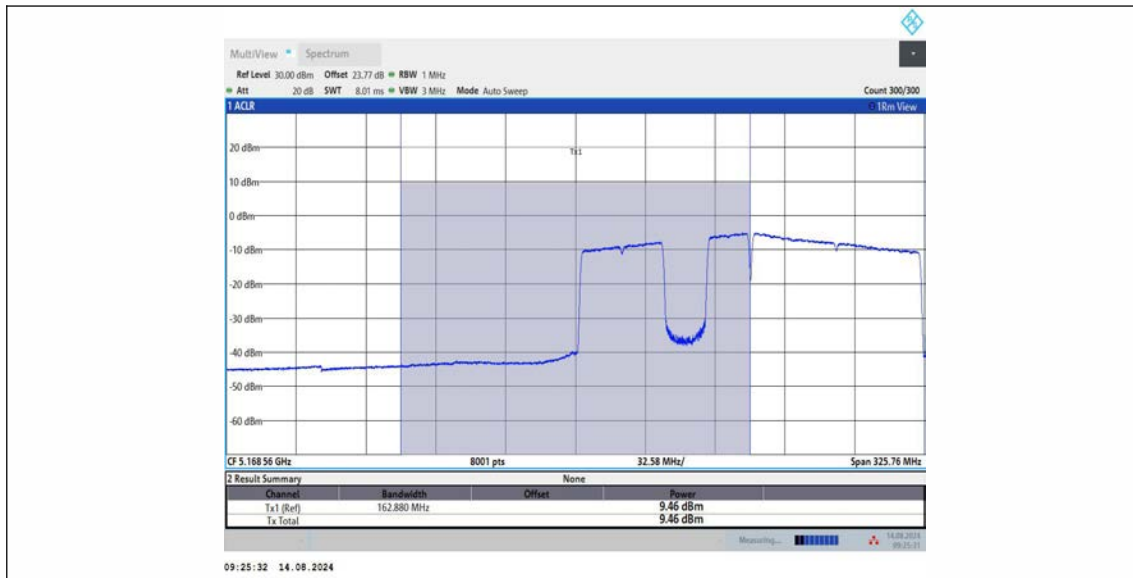
11BE160MIMO_Ant1_5250_UNII-1_996+484+242_OFDMA_3
