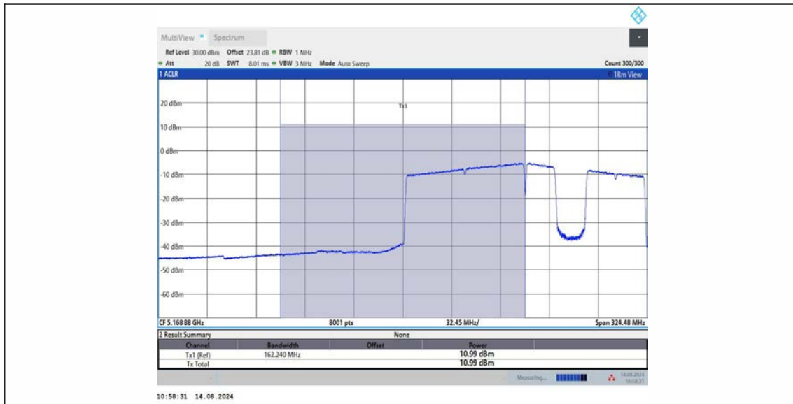
11BE160MIMO_Ant1_5250_UNII-1_996+484+242_OFDMA_6
