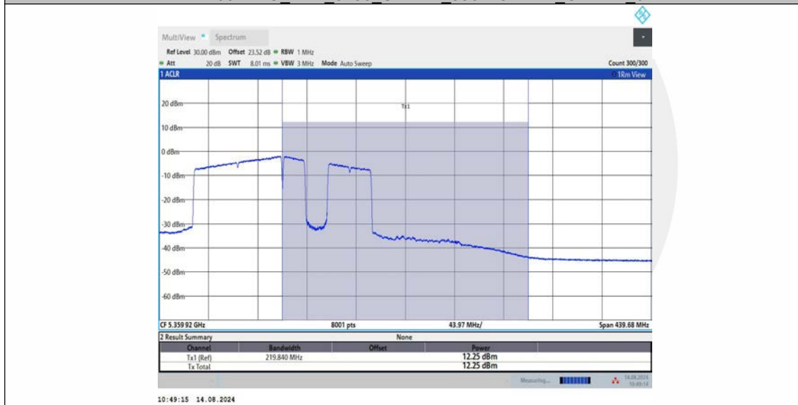
11BE160MIMO Ant1 5250 UNII-2A 996+484+242 OFDMA 7
