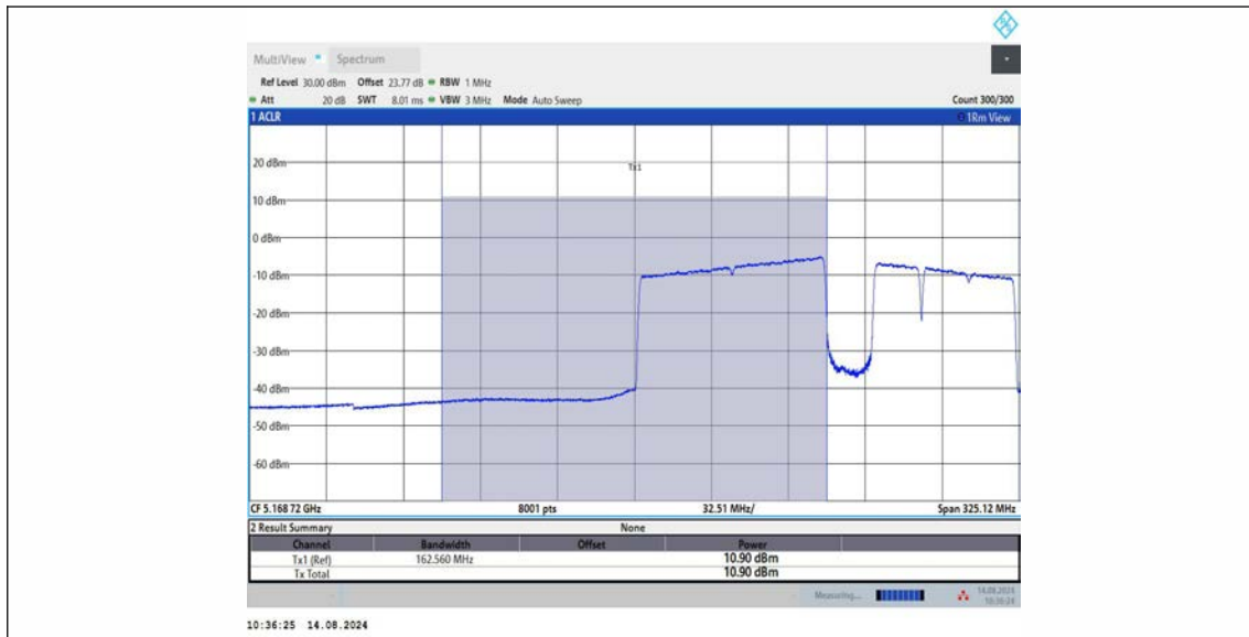
11BE160MIMO_Ant1_5250_UNII-1_996+484+242_OFDMA_5
