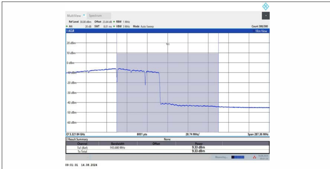
11BE160MIMO_Ant2_5250_UNII-2A_996+484+242_OFDMA_8
