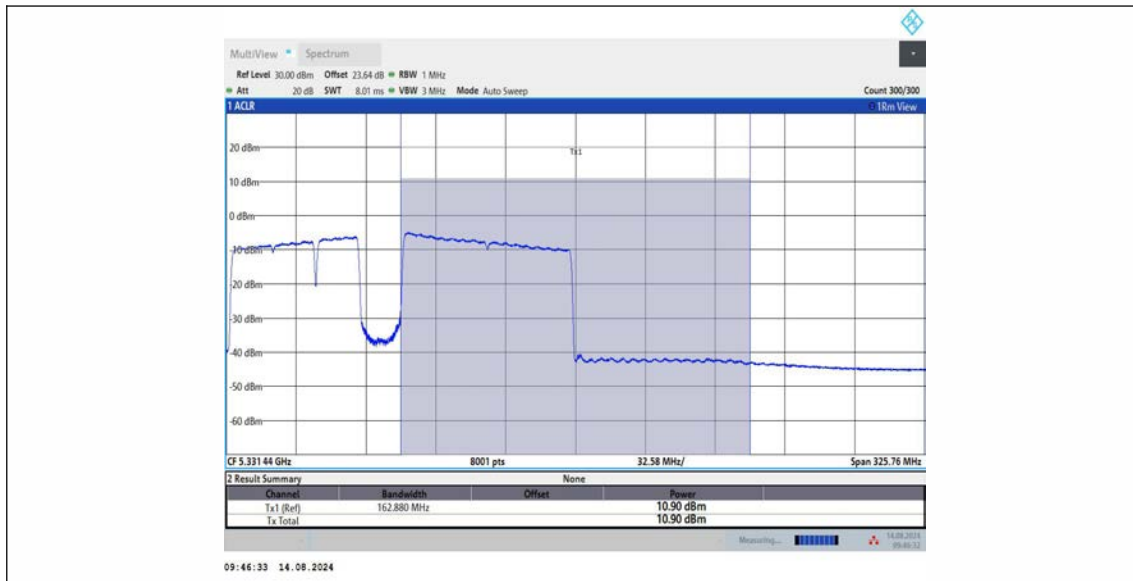
11BE160MIMO Ant2 5250 UNII-2A 996+484+242 OFDMA 4
