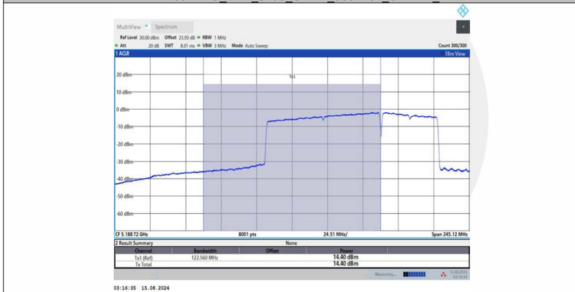
11BE160MIMO Ant2 5250 UNII-1 996+484+242 OFDMA 1
