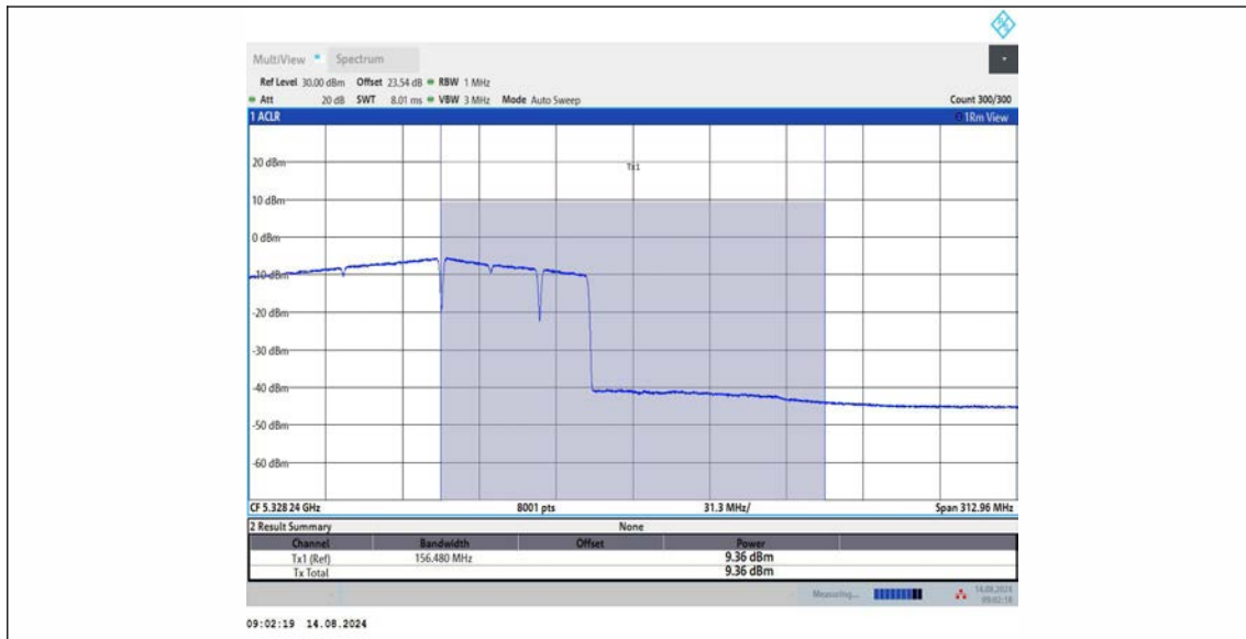
11BE160MIMO_Ant3_5250_UNII-2A_996+484+242_OFDMA_8
