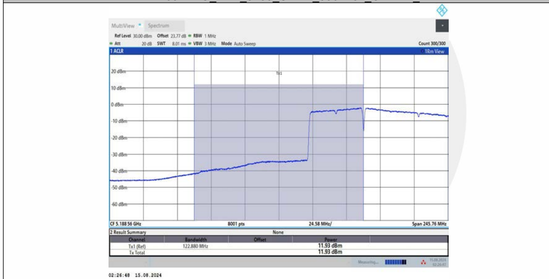
11BE160MIMO_Ant1_5250_UNII-1_996+484_OFDMA_2
