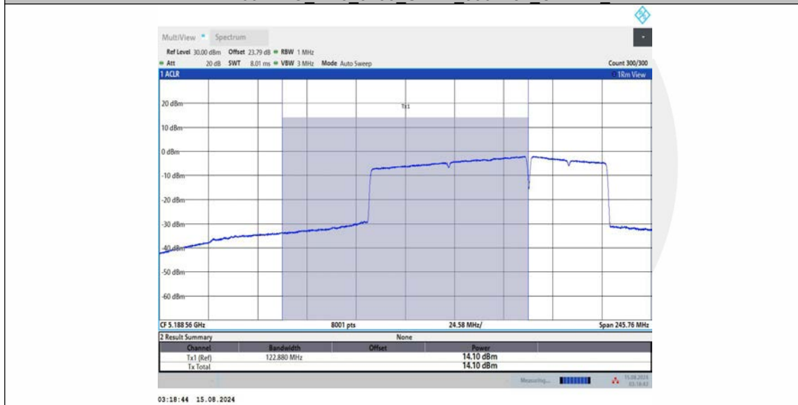
11BE160MIMO_Ant3_5250_UNII-1_996+484+242_OFDMA_1
