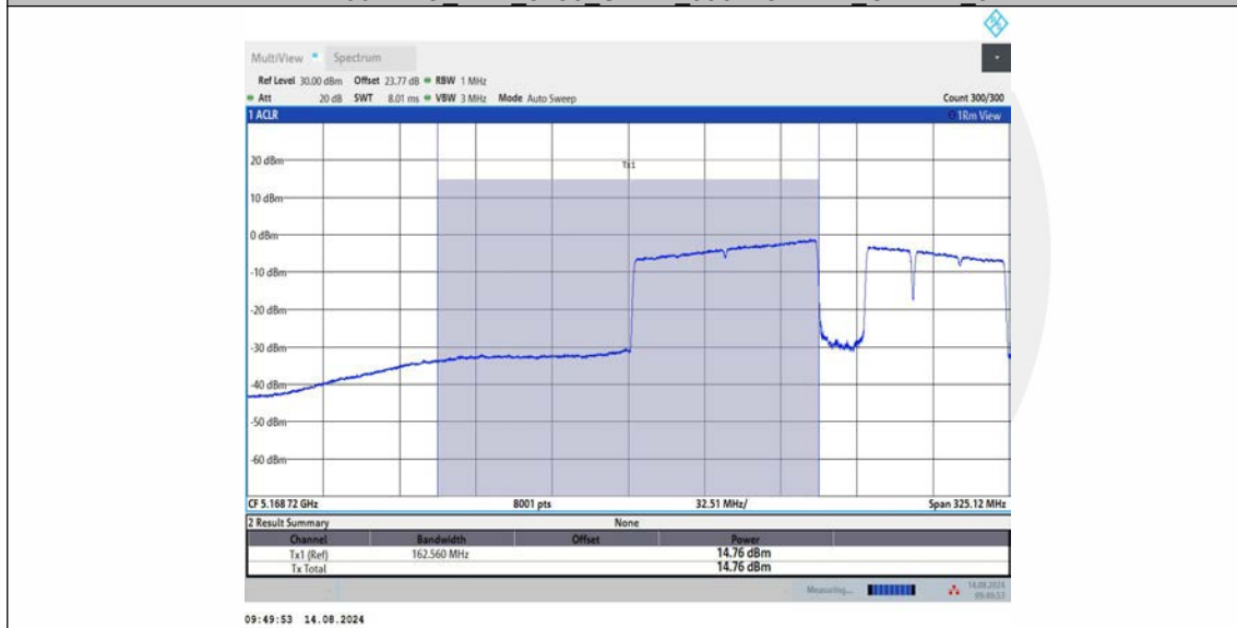
11BE160MIMO_Ant1_5250_UNII-1_996+484+242_OFDMA_6
