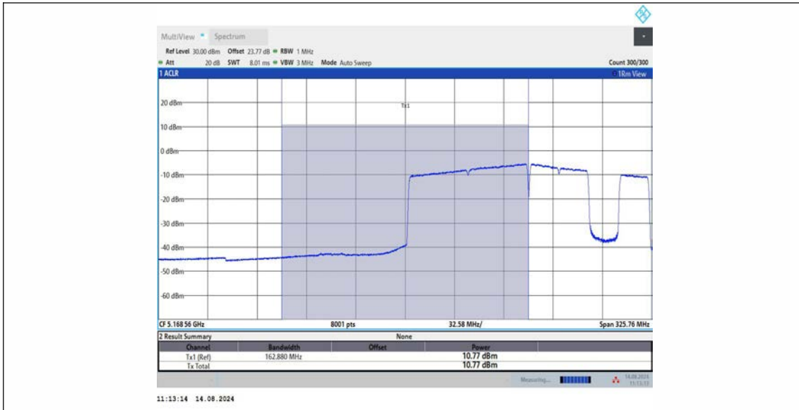
11BE160MIMO_Ant1_5250_UNII-1_996+484+242_OFDMA_7
