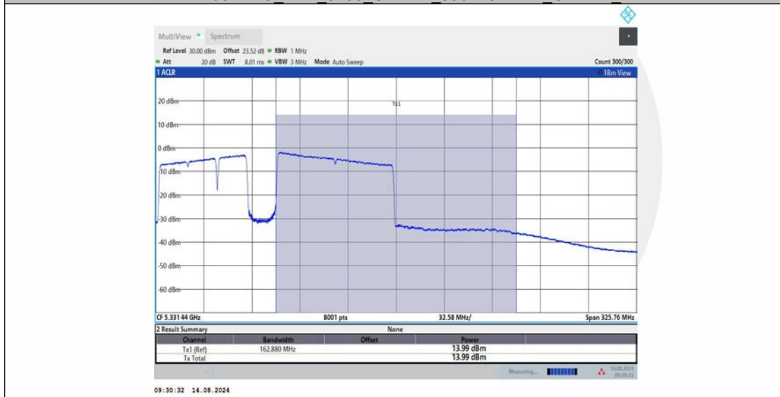
11BE160MIMO Ant1 5250 UNII-2A 996+484+242 OFDMA 5
