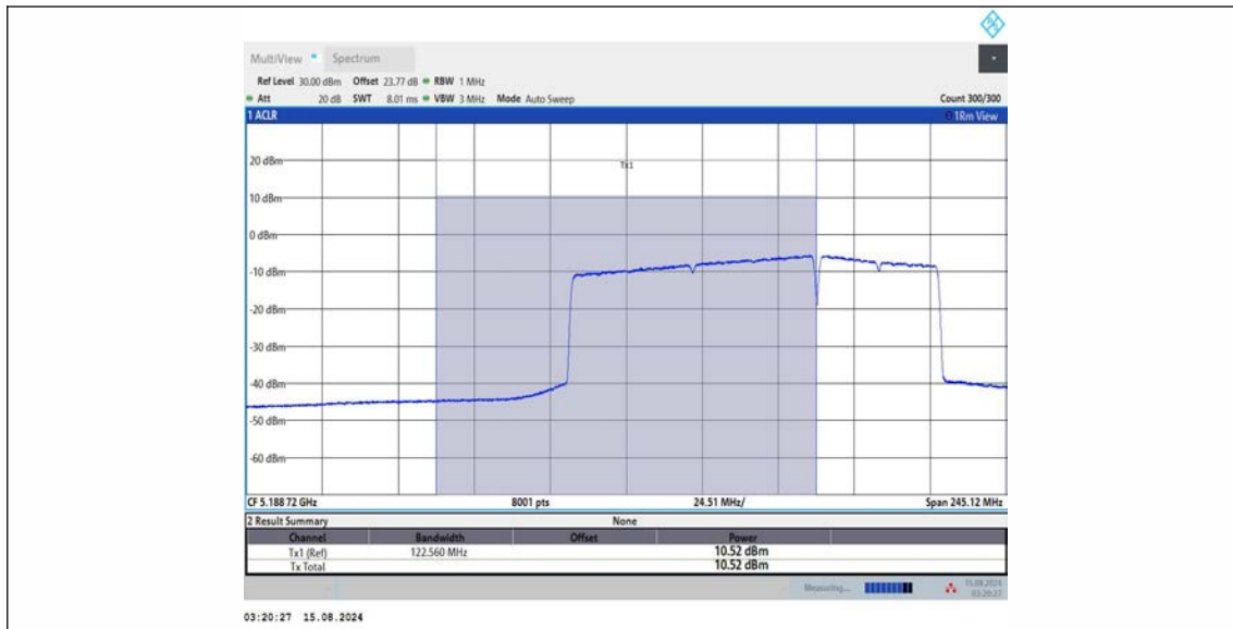
11BE160MIMO_Ant1_5250_UNII-1_996+484_OFDMA_4
