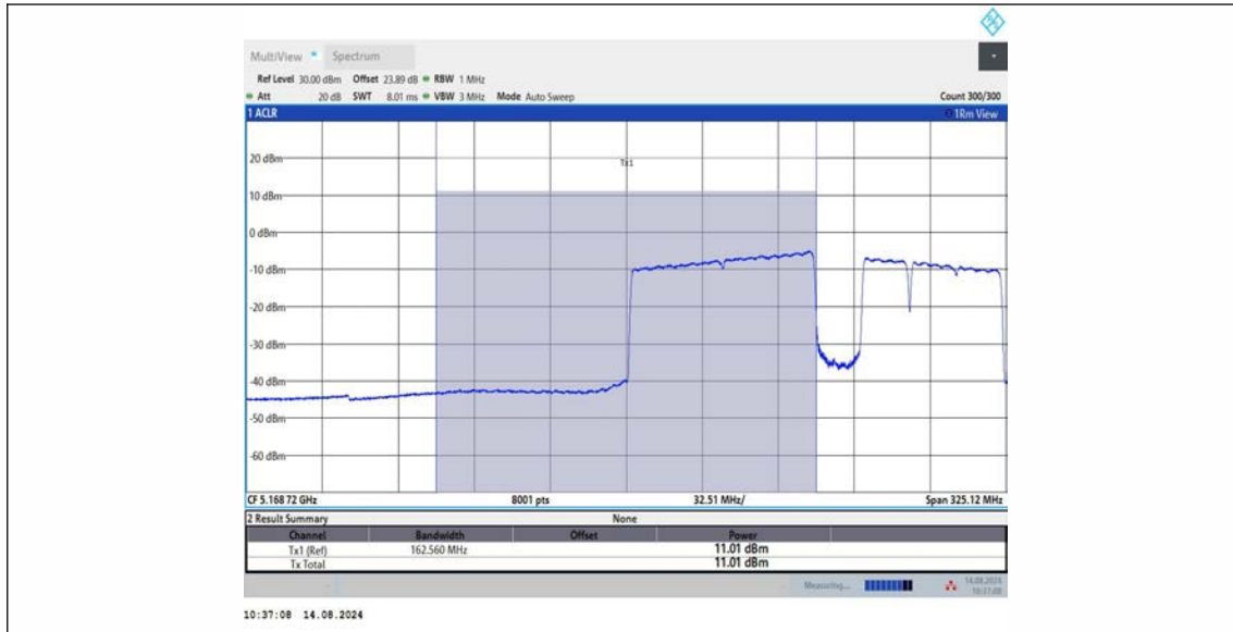
11BE160MIMO_Ant2_5250_UNII-1_996+484+242_OFDMA_5
