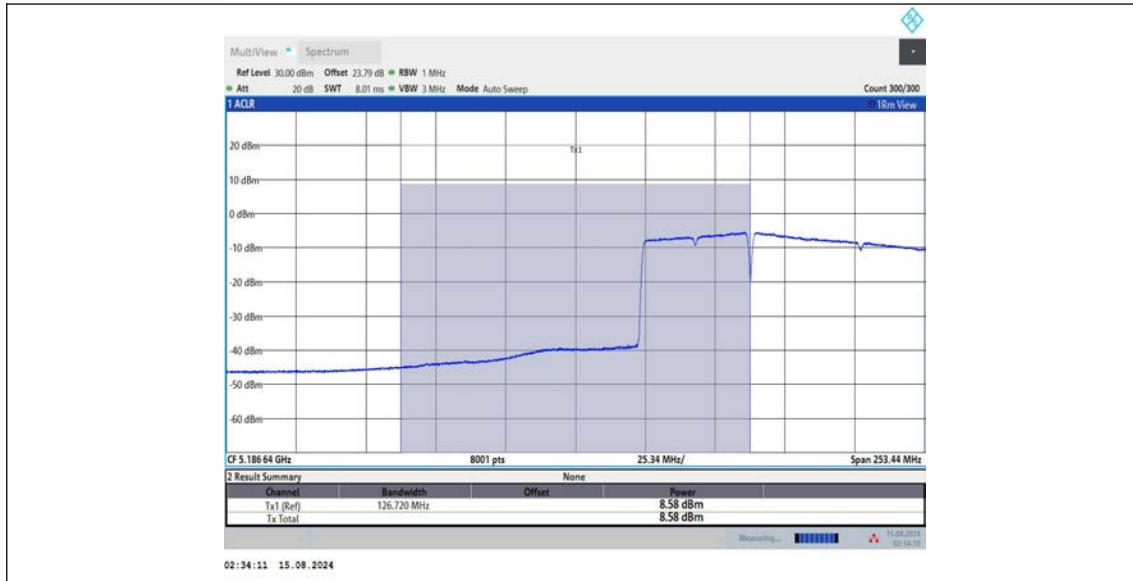
11BE160MIMO_Ant3_5250_UNII-1_996+484_OFDMA_1
