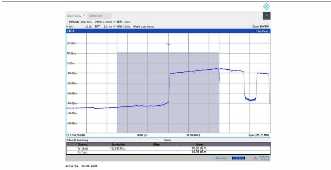
11BE160MIMO_Ant2_5250_UNII-1_996+484+242_OFDMA_7
