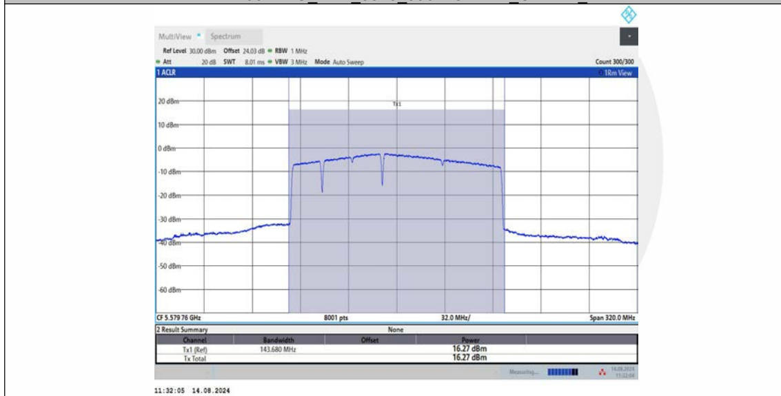
11BE160MIMO_Ant1_5570_996+484+242_OFDMA_2
