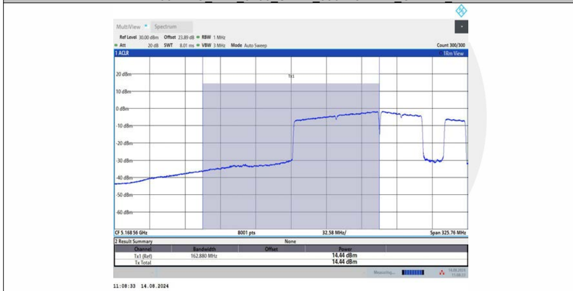
11BE160MIMO_Ant2_5250_UNII-1_996+484+242_OFDMA_8
