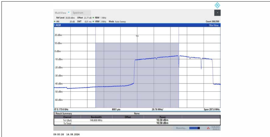
11BE160MIMO_Ant1_5250_UNII-1_996+484+242_OFDMA_8
