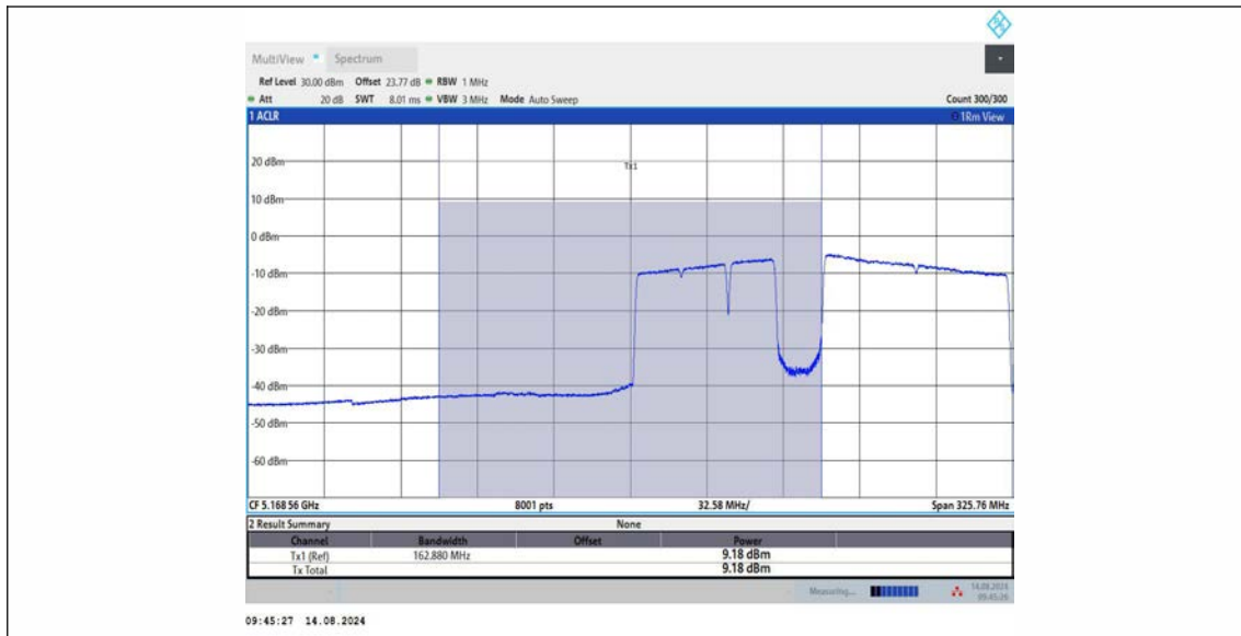
11BE160MIMO_Ant1_5250_UNII-1_996+484+242_OFDMA_4
