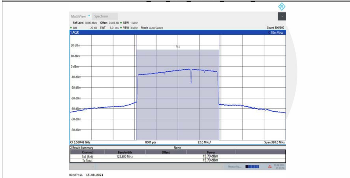
11BE160MIMO Ant1 5570 996+484+242 OFDMA 1
