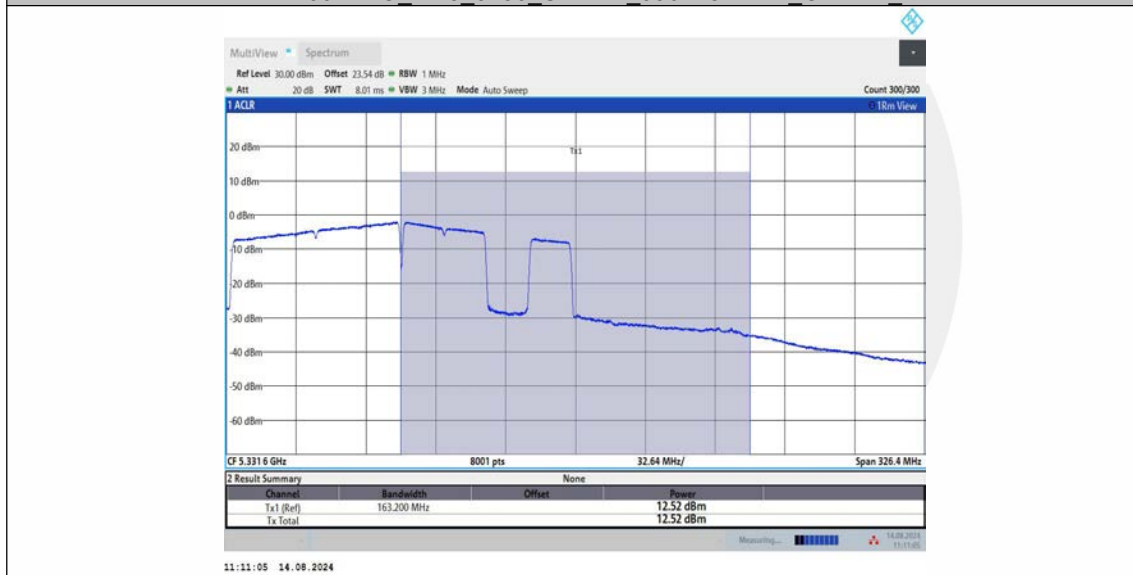
11BE160MIMO Ant3 5250 UNII-2A 996+484+242 OFDMA 8
