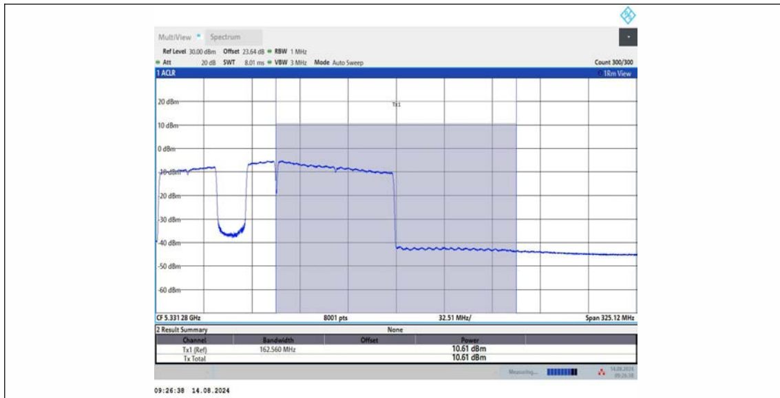
11BE160MIMO Ant2 5250 UNII-2A 996+484+242 OFDMA 3
