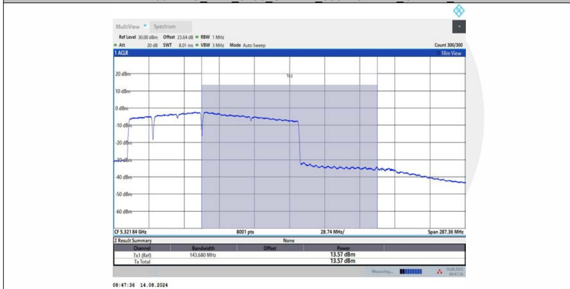
11BE160MIMO_Ant2_5250_UNII-2A_996+484+242_OFDMA_2
