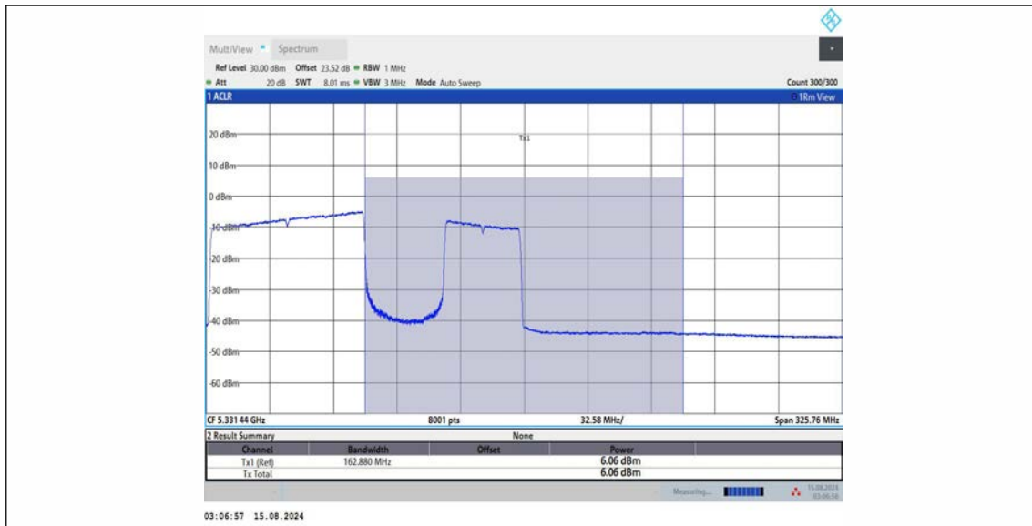
11BE160MIMO Ant1_5250_UNII-2A_996+484_OFDMA_3
