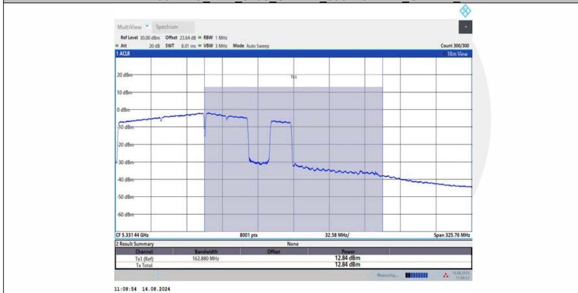
11BE160MIMO Ant2 5250 UNII-2A 996+484+242 OFDMA 8
