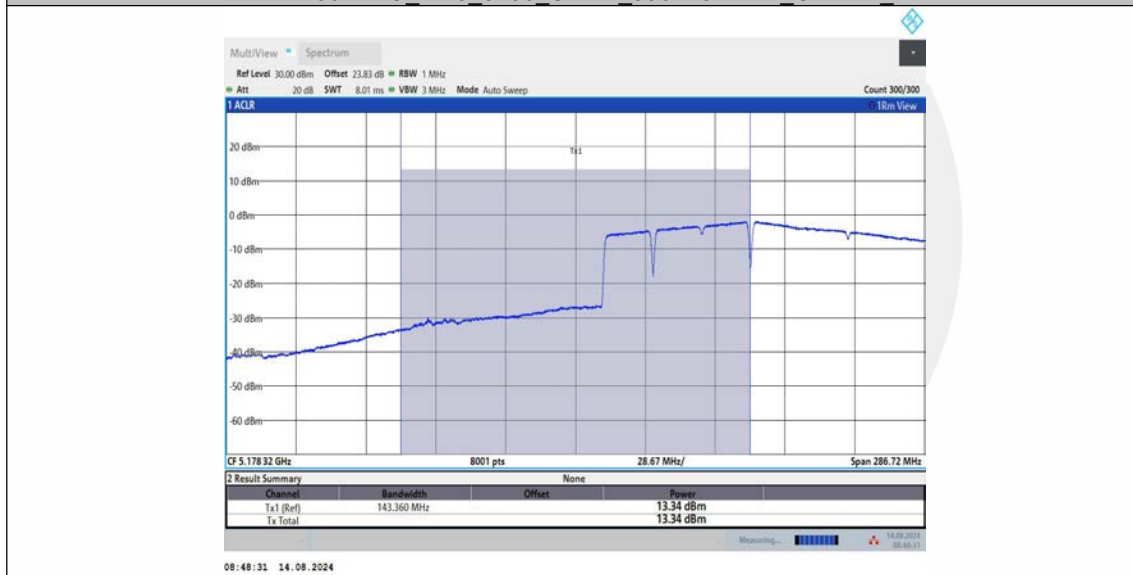
11BE160MIMO_Ant3_5250_UNII-1_996+484+242_OFDMA_2
