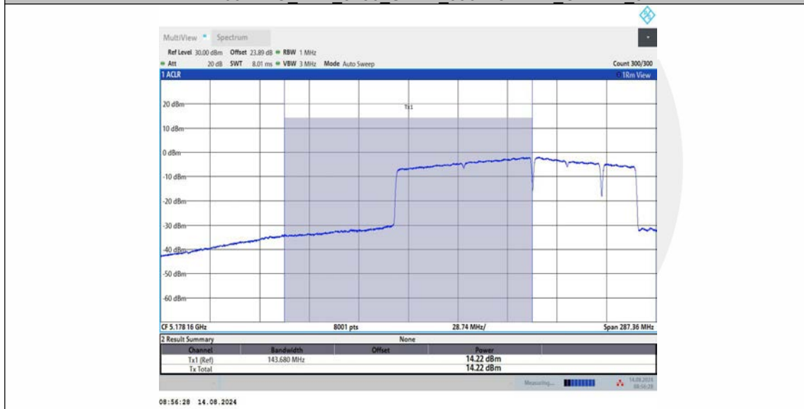
11BE160MIMO Ant3 5250 UNII-1 996+484 OFDMA 1
