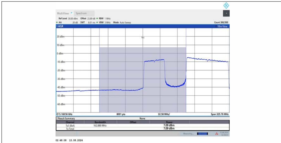
11BE160MIMO_Ant2_5250_UNII-1_996+484_OFDMA_2
