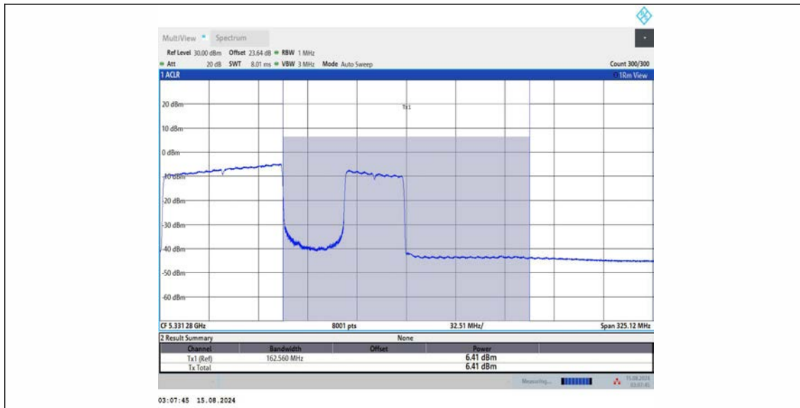
11BE160MIMO_Ant2_5250_UNII-2A_996+484_OFDMA_3
