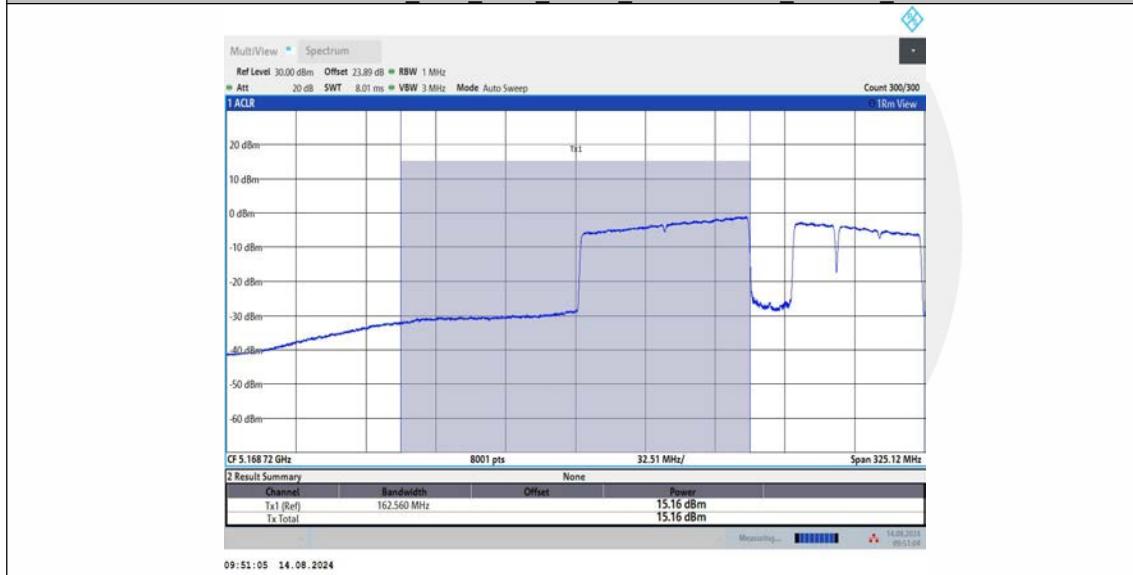
11BE160MIMO_Ant2_5250_UNII-1_996+484+242_OFDMA_6
