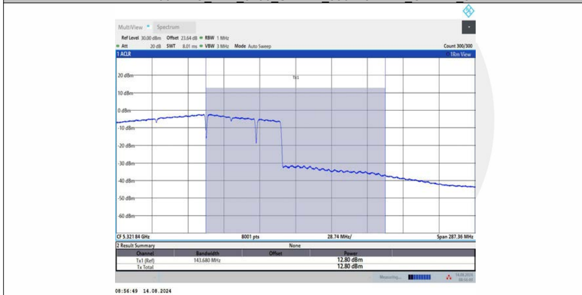
11BE160MIMO_Ant3_5250_UNII-2A_996+484_OFDMA_1
