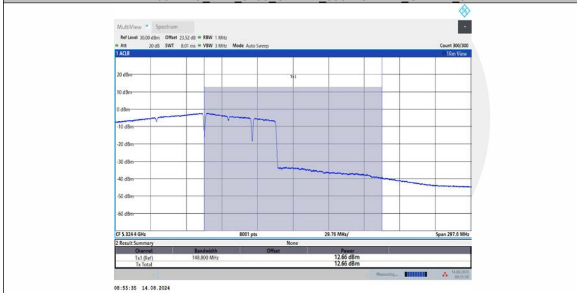
11BE160MIMO_Ant2 5250 UNII-2A 996+484 OFDMA 1
