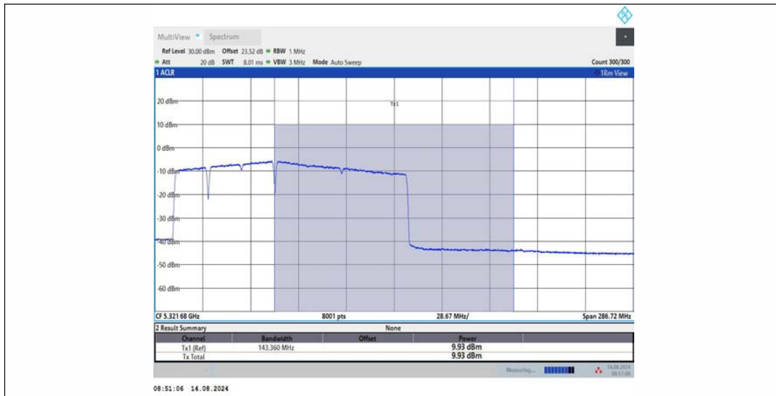
11BE160MIMO Ant1 5250 UNII-2A 996+484+242 OFDMA 1
