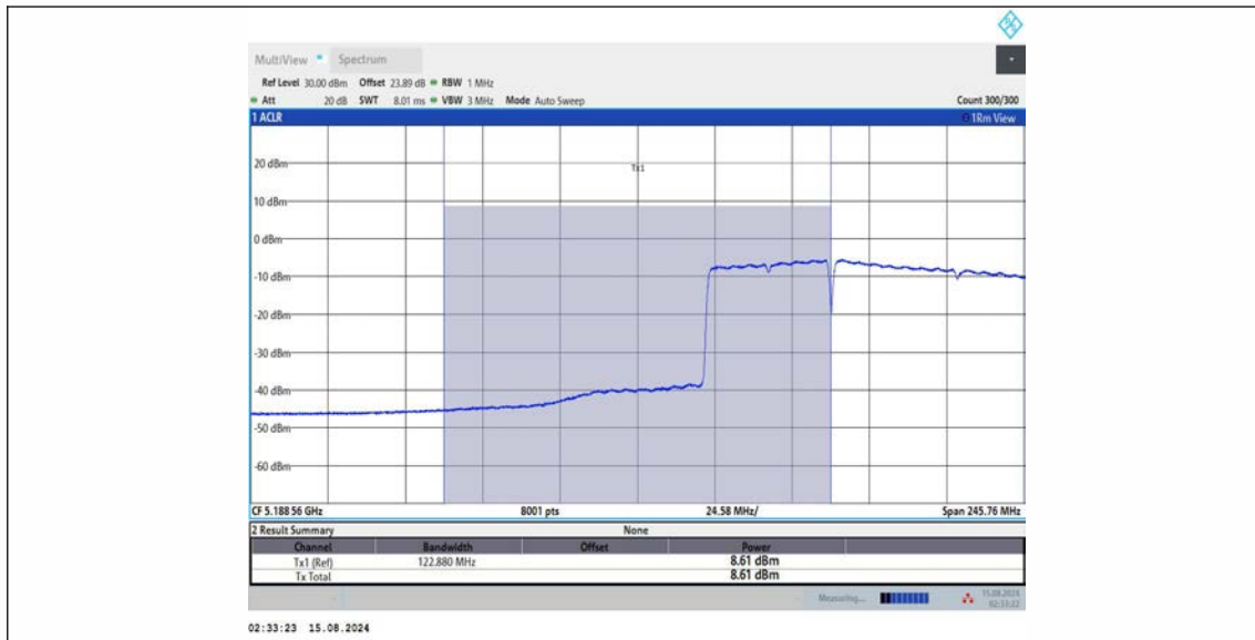
11BE160MIMO_Ant2_5250_UNII-1_996+484_OFDMA_1
