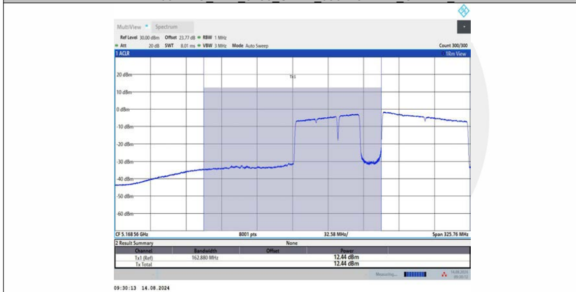
11BE160MIMO_Ant1_5250_UNII-1_996+484+242_OFDMA_5
