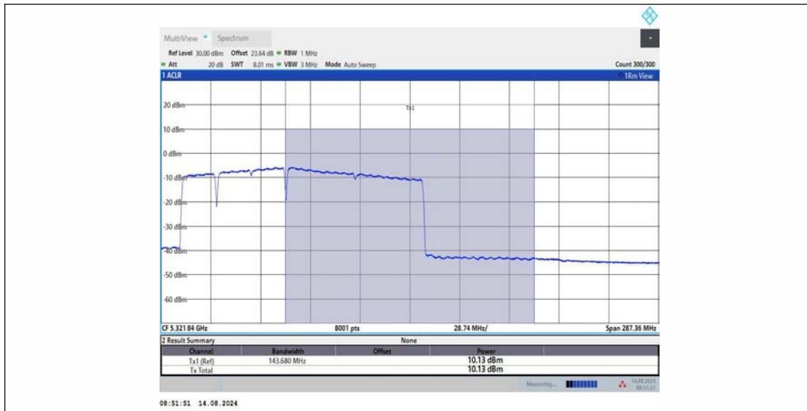
11BE160MIMO_Ant2_5250_UNII-2A_996+484+242_OFDMA_1
