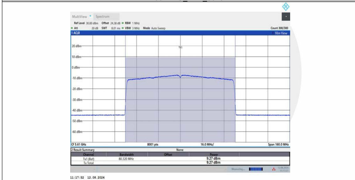
11AX80MIMO Ant2 5610
