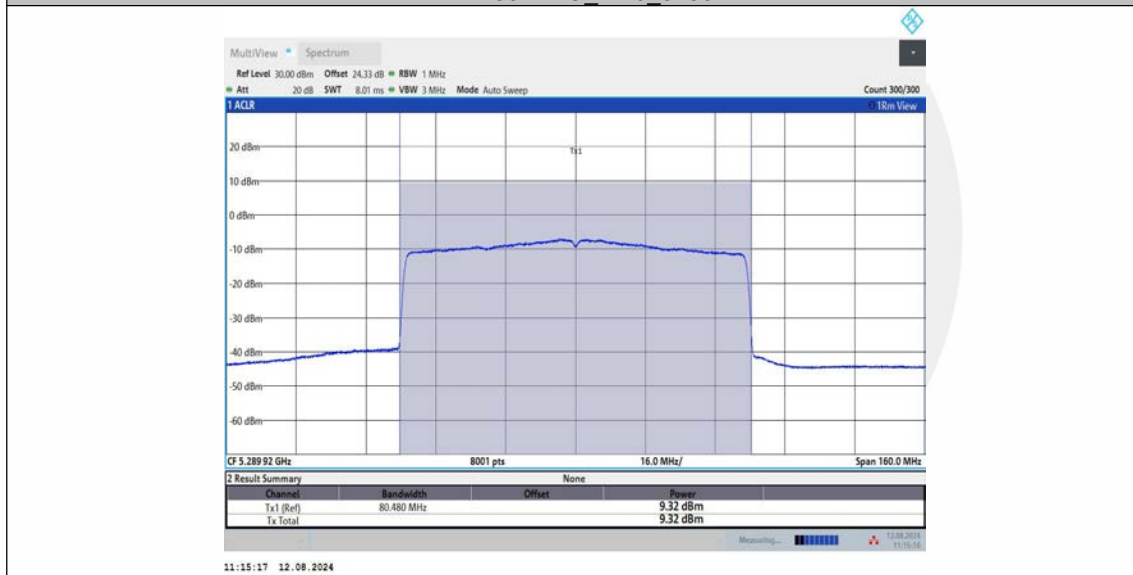
11AX80MIMO Ant3 5290
