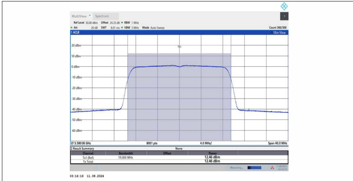
11AC20MIMO Ant3 5580
