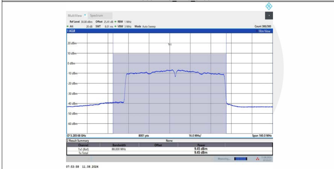
11AC80MIMO Ant3 5290
