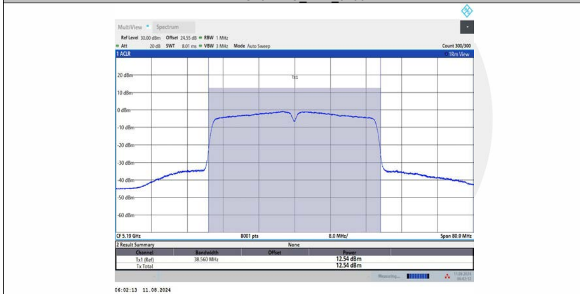
11AC40MIMO Ant3_5190
