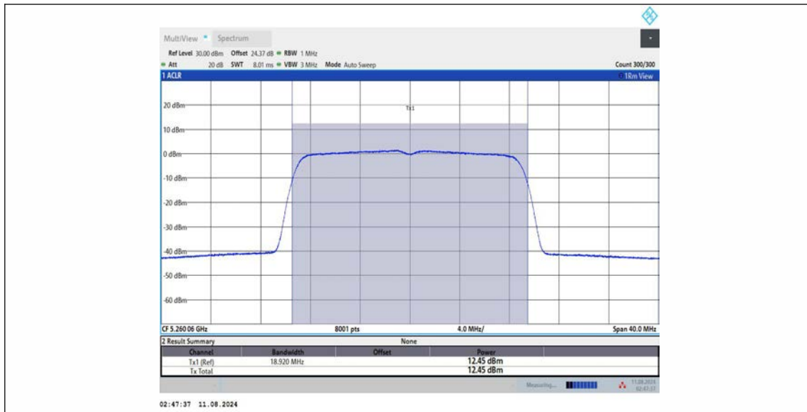
11AC20MIMO Ant3 5260
