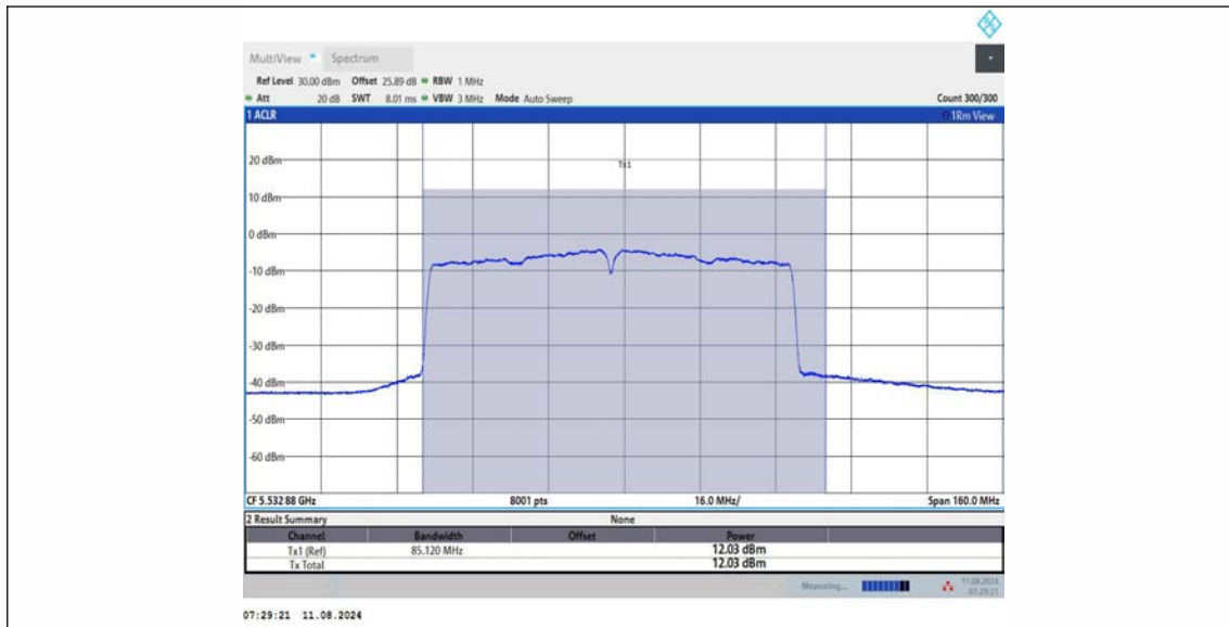
11AC80MIMO Ant3 5530
