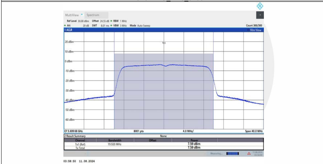
11AC20MIMO Ant3 5700
