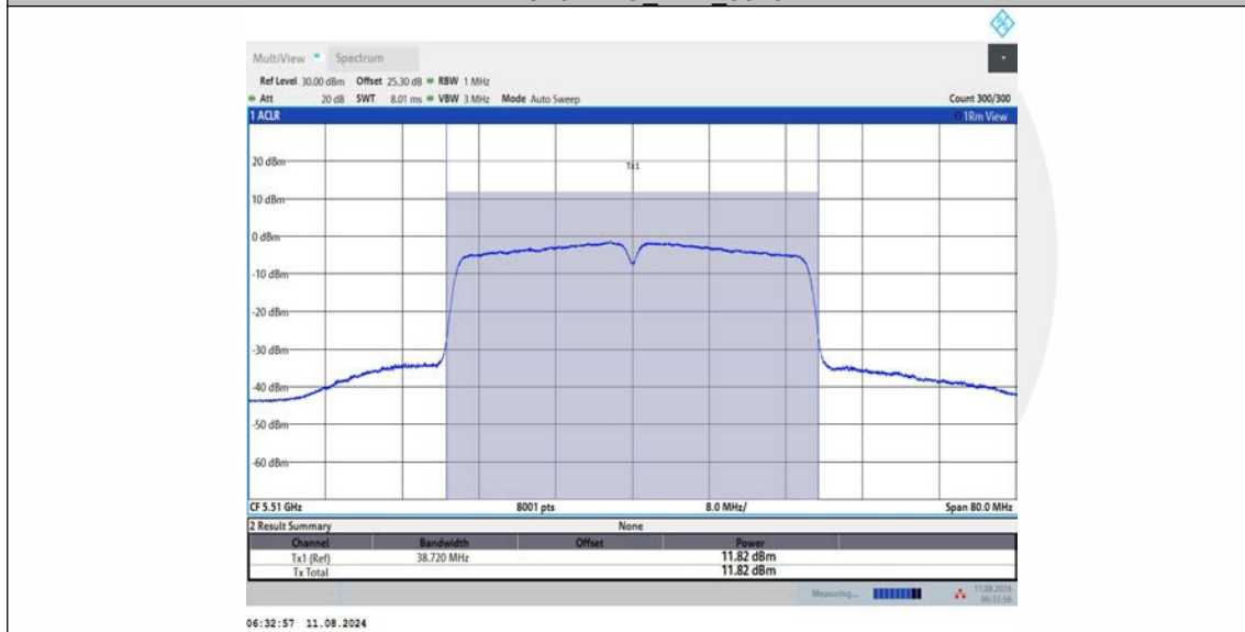
11AC40MIMO Ant3_5510
