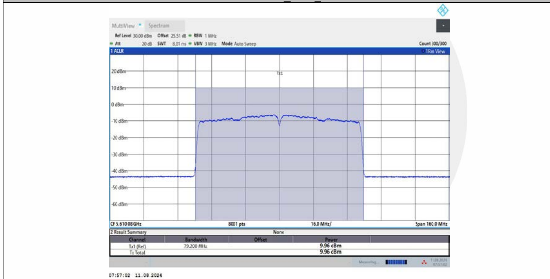
11AC80MIMO Ant3 5610
