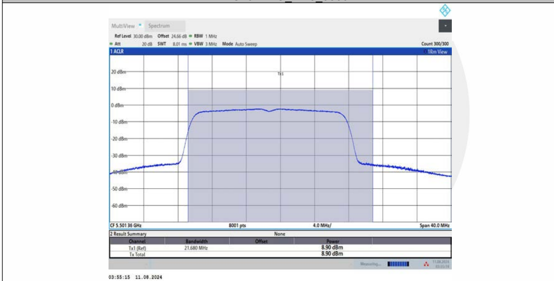
11AC20MIMO Ant3 5500
