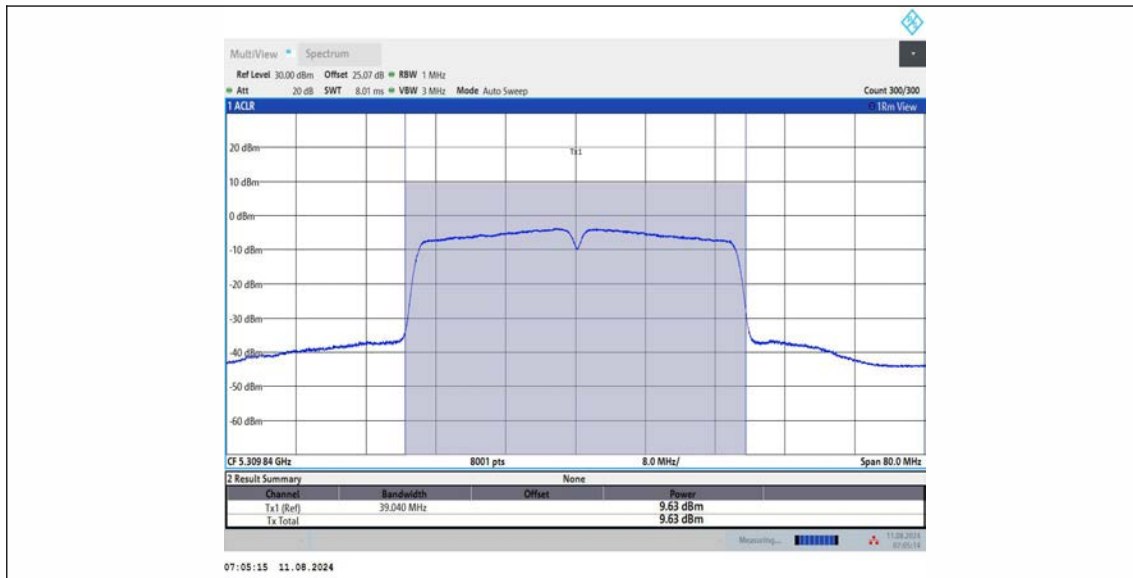
11AC40MIMO Ant3 5310
