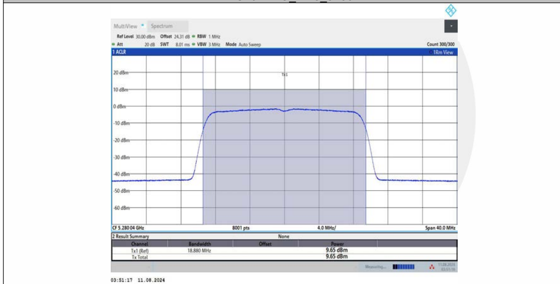
11AC20MIMO Ant3 5280
