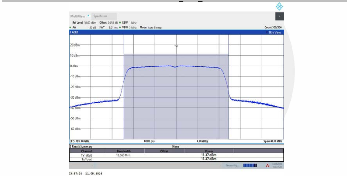
11AC20MIMO Ant3_5785
