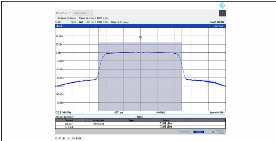
11AC20MIMO Ant3 5320
