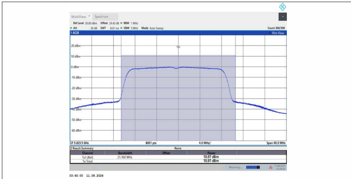
11AC20MIMO Ant3 5825
