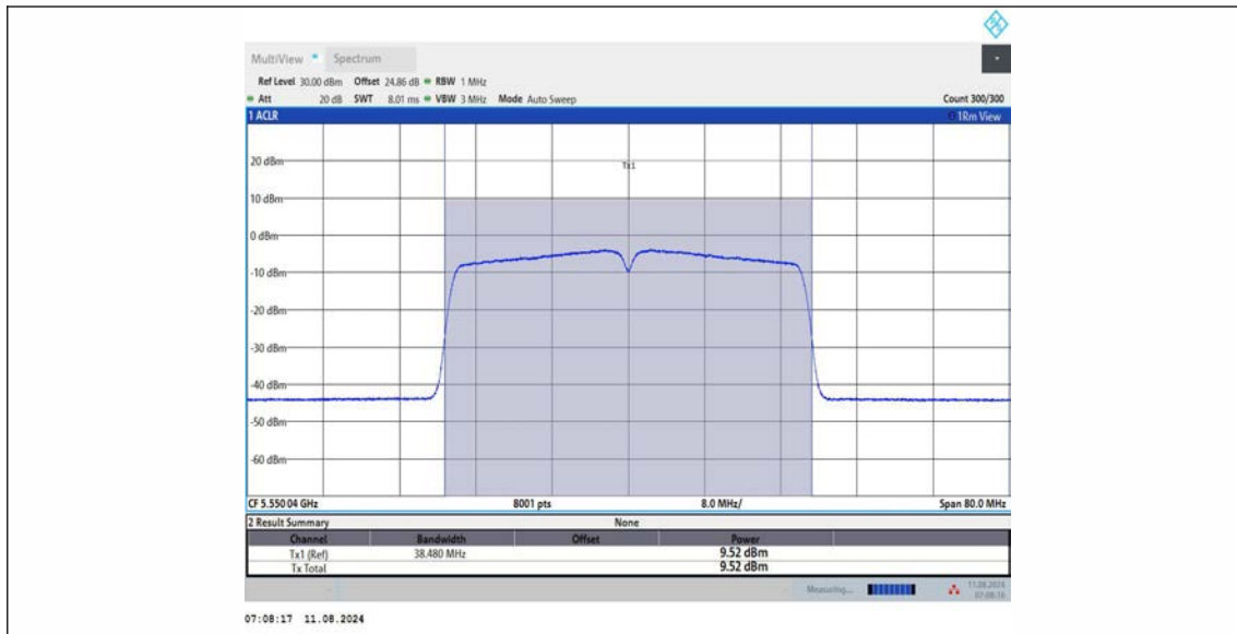
11AC40MIMO Ant3 5550
