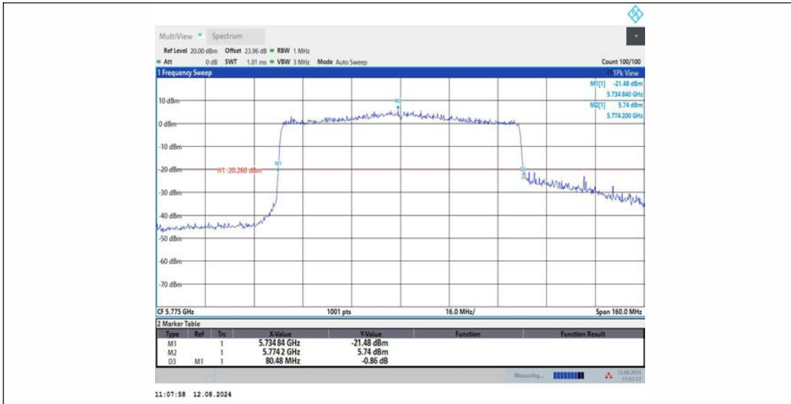
11AX80MIMO Ant2_5775
