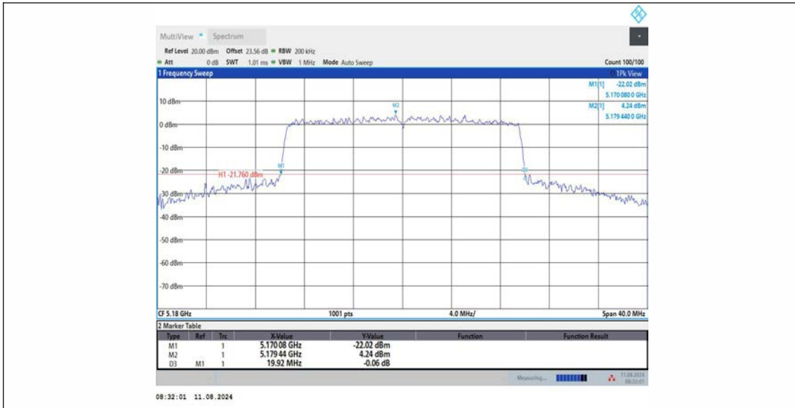
11AX20MIMO Ant3_5180
