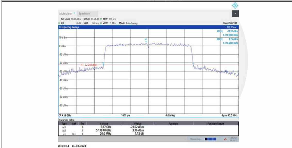
11AX20MIMO Ant2_5180
