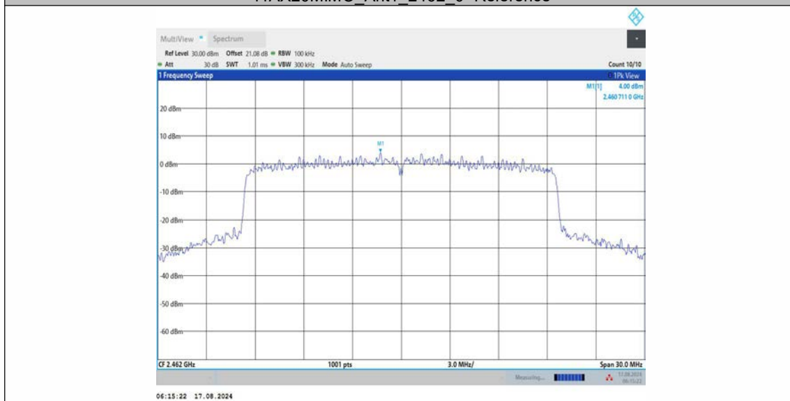
11AX20MIMO Ant1_2462_0~Reference
