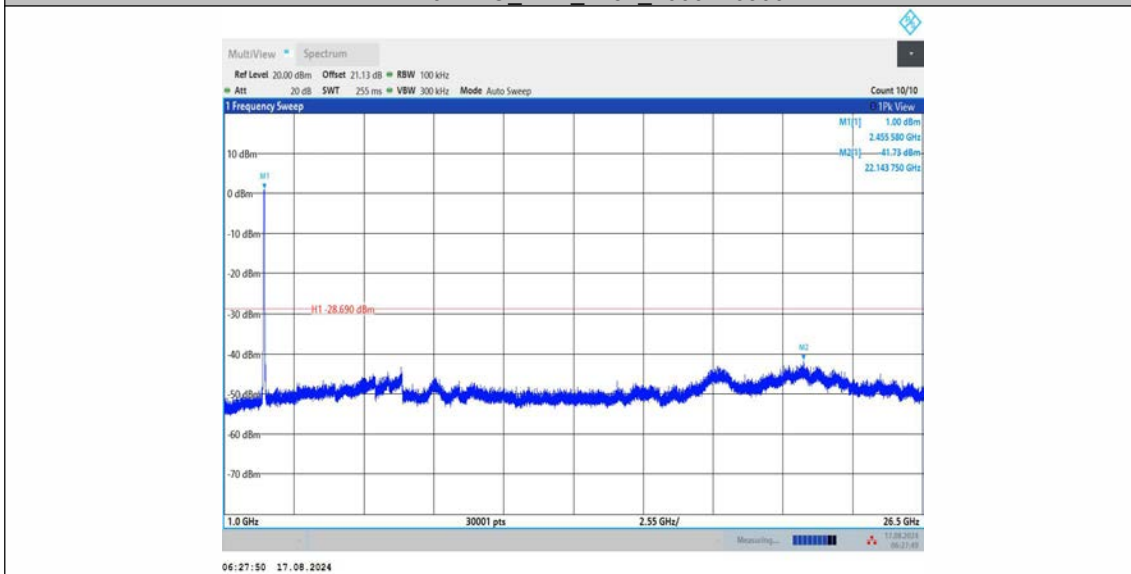
11AX40MIMO Ant1_2452_1000~26500
