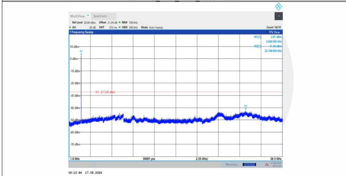
11AX20MIMO Ant1_2462_0~Reference
