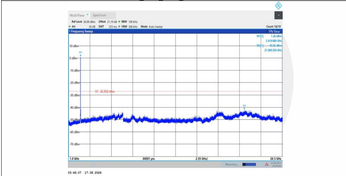
11G_Ant1_2437_0~Reference
