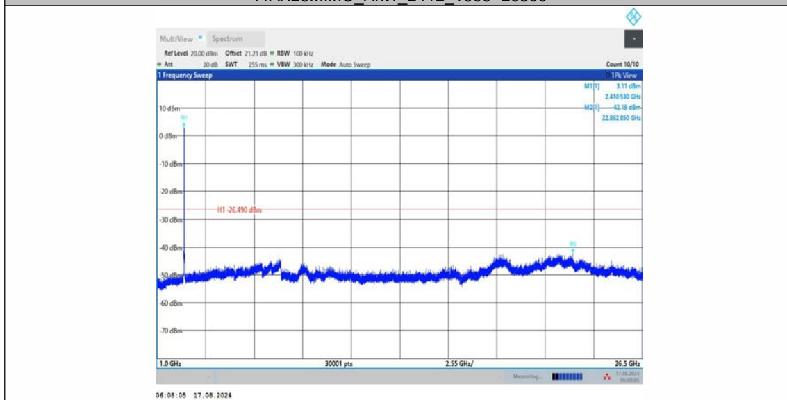
11AX20MIMO Ant1_2412_1000~26500
