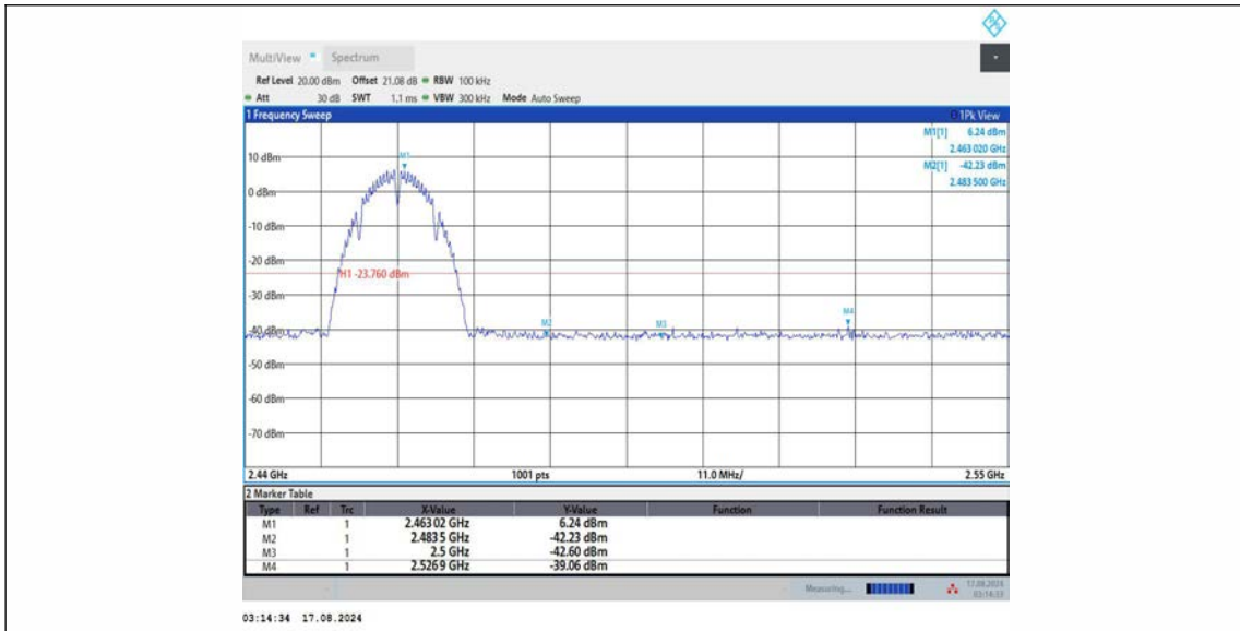
11B_Ant2_High_2462
