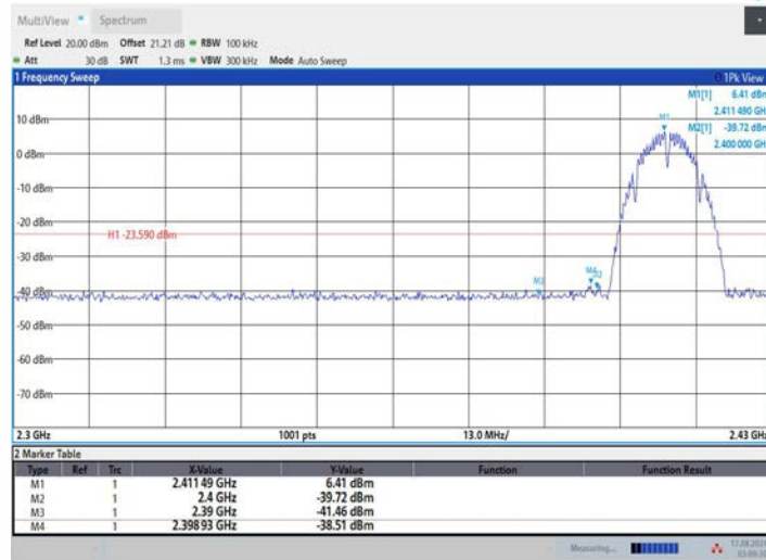
11B_Ant2_Low_2412
