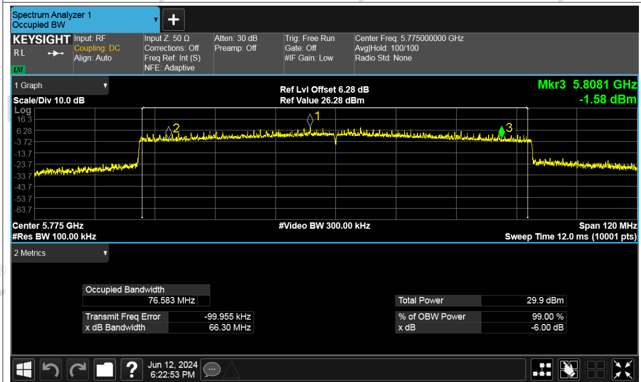
-6dB Bandwidth NVNT be80 5775MHz Ant3
