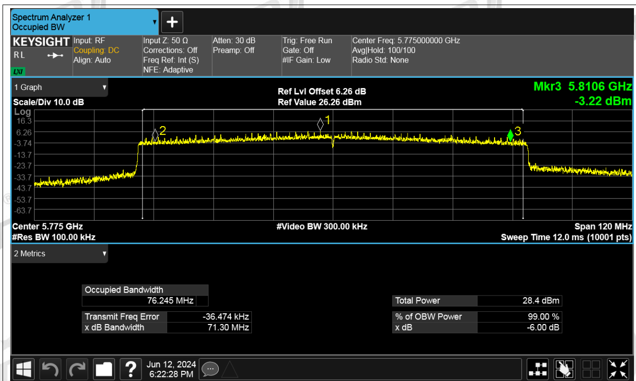
-6dB Bandwidth NVNT be80 5775MHz Ant2
