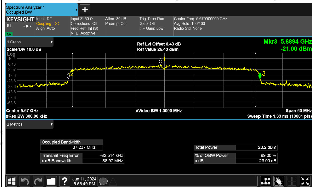
-26dB Bandwidth NVNT ax40 5670MHz Ant3
