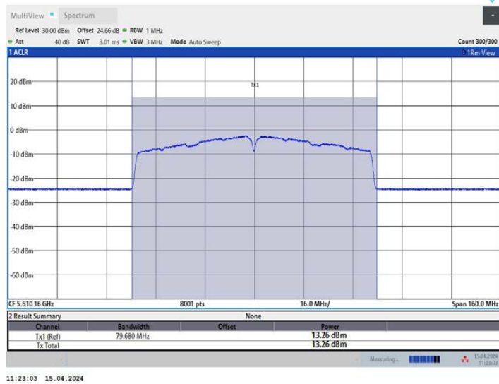
11AC80MIMO Ant3_5610
