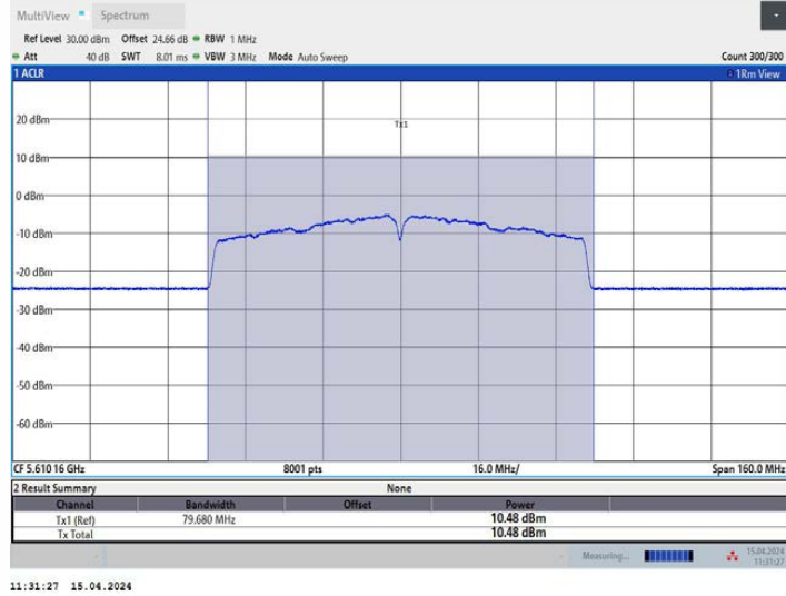
11AC80MIMO Ant2_5610
