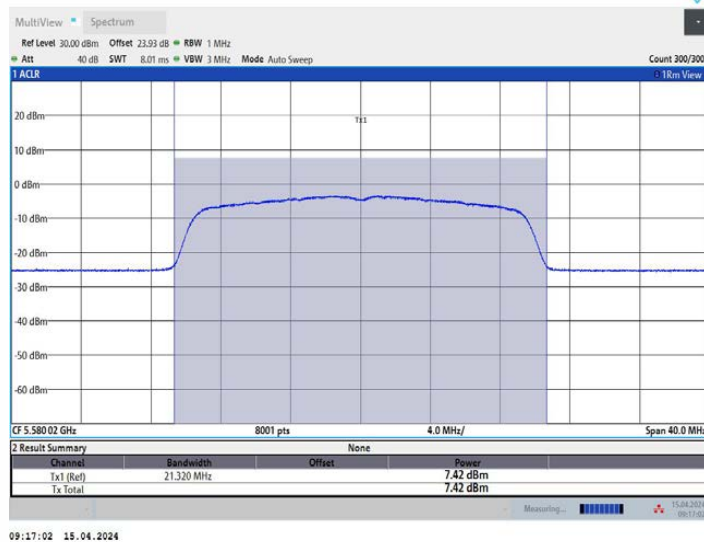
11AX20MIMO Ant1_5580
