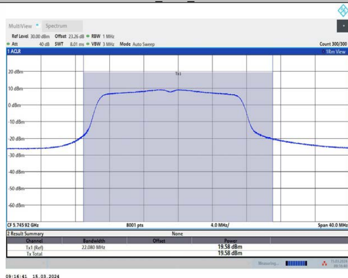
11A_Ant3_5745
