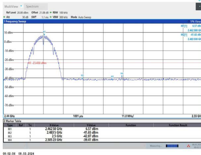
11B_Ant1_High_2462
