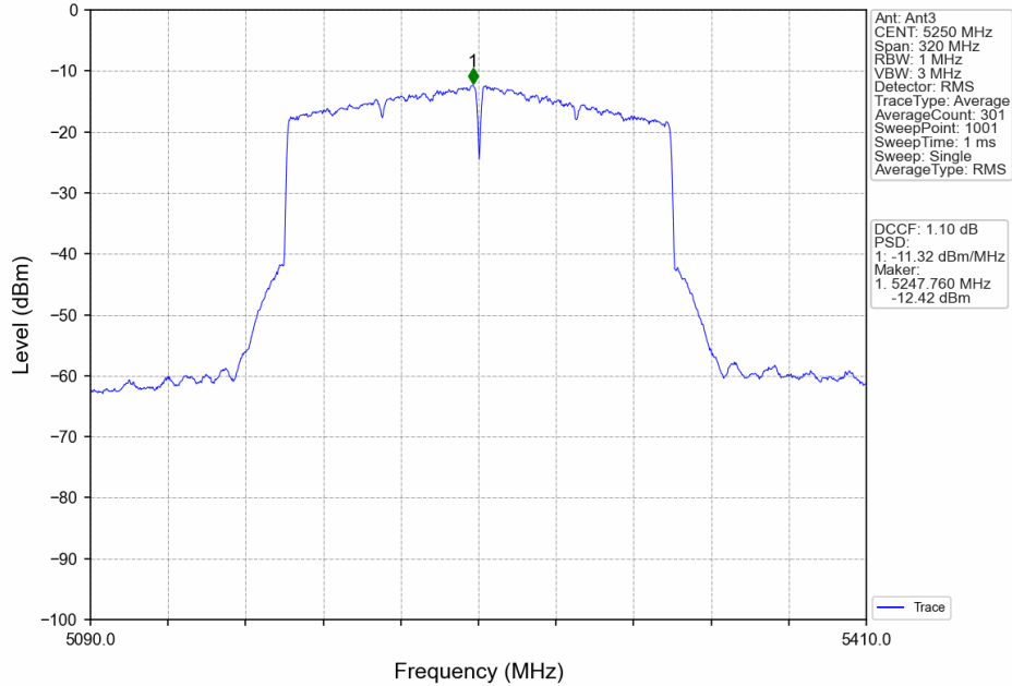
802.11ax(HEW160)_MCH_5250MHz_2xRU996_Left_MIMO_NTNV
