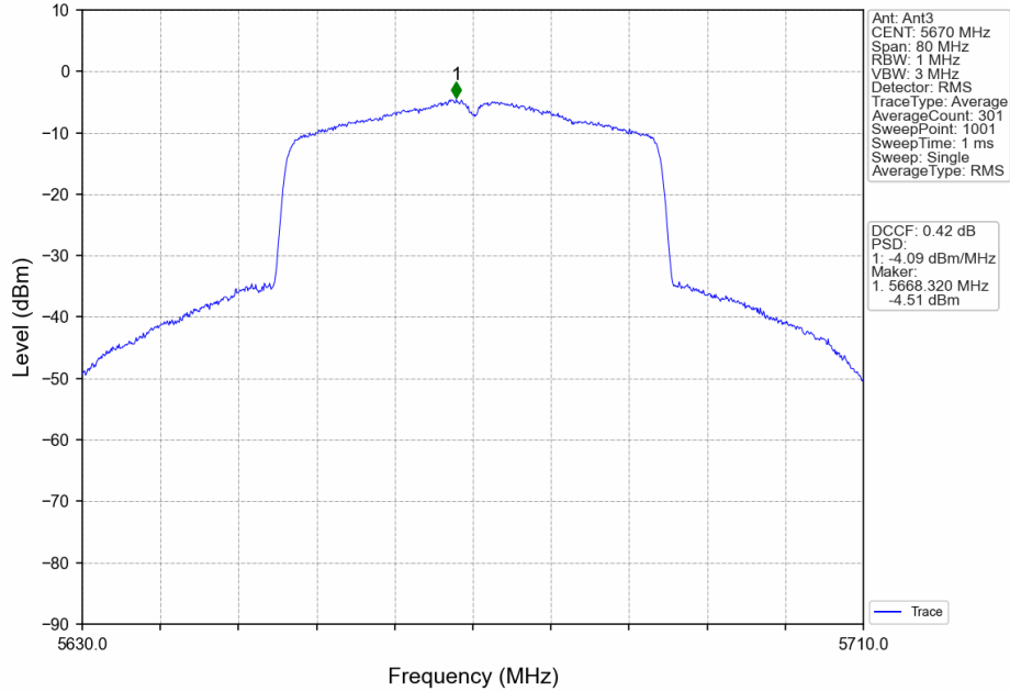
802.11ax(HEW40)_HCH_5670MHz_RU484_Left_MIMO_NTNV
